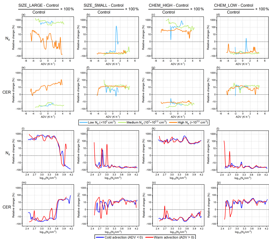
Figure 9. Percentage changes in N_d (a–d, i–l) and CER (e–h, m–p) for the SIZE_LARGE (first column), SIZE_SMALL (second column), CHEM_HIGH (third column), and CHEM_LOW (fourth column) experiments relative to the Control experiment. Upper two rows: dependence on ADV ( x axis) for different N_a conditions; lower two rows: dependence on N_a ( x axis) for different ADV conditions.
