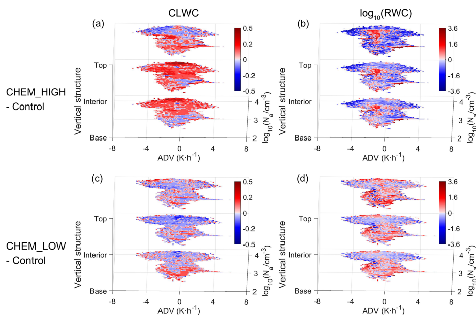
Figure 13. Differences between the CHEM_HIGH (a–b) and CHEM_LOW (c–d) experiments and the Control experiment in CLWC (left column, unit: \text{g m}^{-3} ) and RWC (right column, unit: \text{g m}^{-3} , presented logarithmically in base 10) as a function of N_a , ADV and cloud parts.
