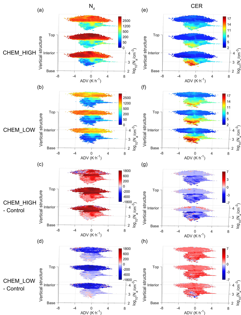
Figure 12. Variation of N_d (left column, in \text{cm}^{-3} ) and CER (right column, in \mu\text{m} ) with N_a , ADV and cloud parts for the CHEM_HIGH (a, e) and CHEM_LOW (b, f) experiments, and the differences of the CHEM_HIGH (c, g) and CHEM_LOW (d, h) experiments relative to the Control experiment.
