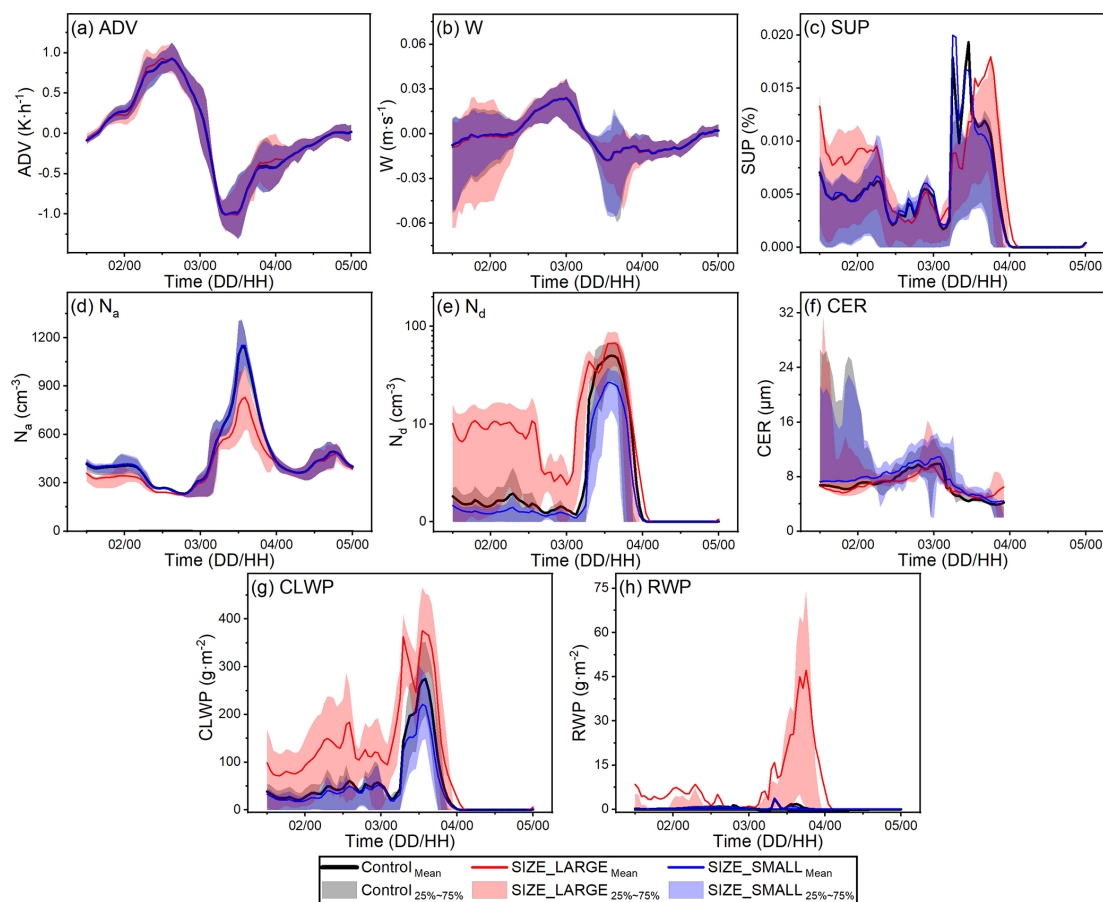
Figure 2. Temporal variations (lines, ECO regional mean) and the 25%–75% interquartile range (shading, regional variability) of vertically weighted average temperature advection ( a ), vertical velocity ( b ) and supersaturation ( c ) from near the surface up to 1300 m (this height range is selected because over 97% of cloud droplets during the simulation period exist within this range, ensuring an accurate representation of the meteorological influence on ACI), column-mean N_a ( d ) and N_d ( e ), as well as CER ( f ), CLWP ( g ) and RWP ( h ) over ECO from the Control, SIZE_LARGE, and SIZE_SMALL experiments.
