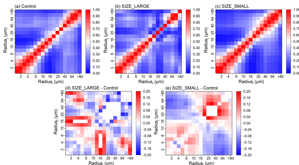
Figure 6. Correlation map between liquid droplet number concentrations in size bins i and j from the Control (a), SIZE_LARGE (b), and SIZE_SMALL (c) experiments, and differences of SIZE_LARGE (d) and SIZE_SMALL (e) with the Control. For each size bin, the four-dimensional (time, height, latitude, longitude) droplet number concentration field is first flattened into a one-dimensional array in the same order, and the Pearson correlation coefficient between bins i and j is then computed.
