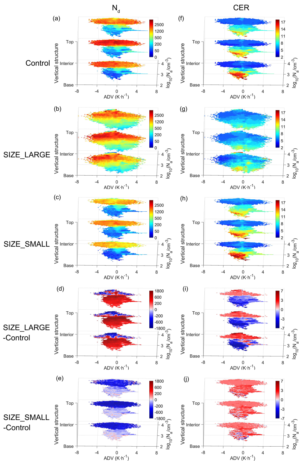
Figure 4. Variation of N_d (left column, in cm^{-3} ) and CER (right column, in \mu m ) of liquid-phase clouds with N_a , ADV and cloud parts for the Control (a, f), SIZE_LARGE (b, g), and SIZE_SMALL (c, h) experiments, and the differences of the SIZE_LARGE (d, i) and SIZE_SMALL (e, j) experiments relative to the Control experiment.
