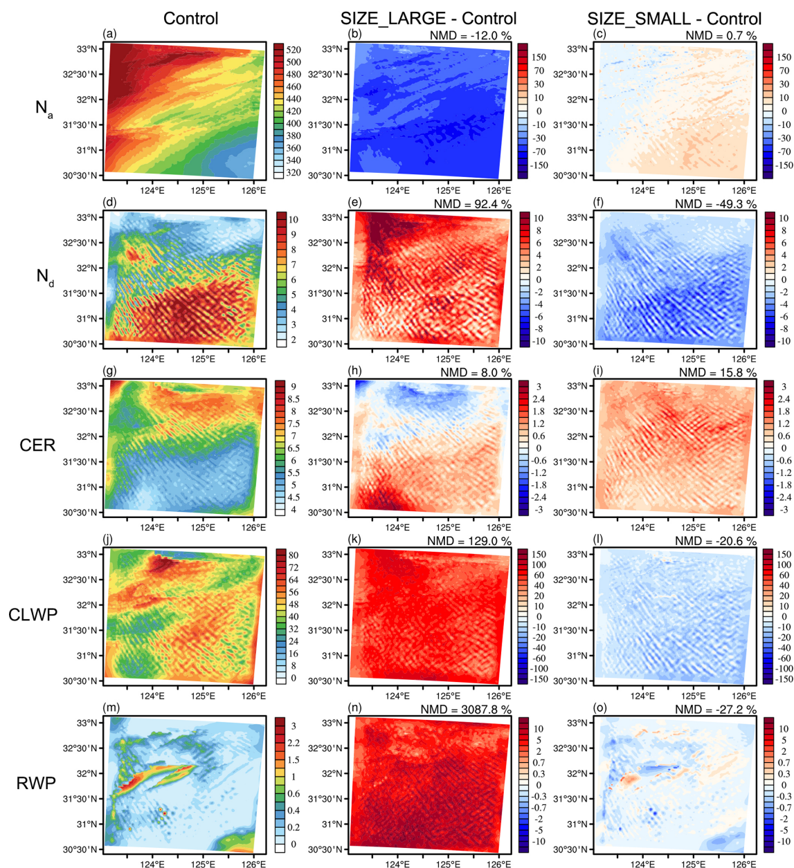
Figure 3. Spatial distributions of column-mean N_a (a–c, in \text{cm}^{-3} ) and N_d (d–f, in \text{cm}^{-3} ), mean CER (g–i, in \mu\text{m} ), CLWP (j–l, in \text{m}^{-2} ), and RWP (m–o, in \text{g m}^{-2} ) averaged over the simulation period from the Control experiment (left column), and differences of SIZE_LARGE (middle column) and SIZE_SMALL (right column) relative to the Control (NMD of each sensitivity experiment relative to the Control is indicated at the top-right of each subplot). Values represent liquid-phase clouds averaged over the simulation period, and grid points without clouds or with non-liquid-phase clouds are excluded. N_a and N_d are column averages, CLWP and RWP are column totals, and CER is calculated based on the droplet number in each bin.
