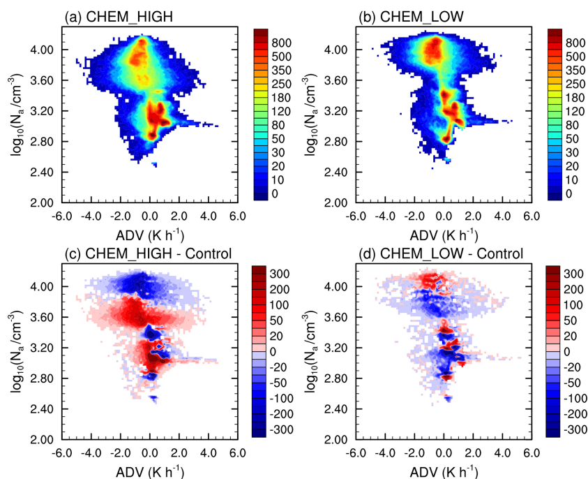
Figure 14. Variation of cloud lifetime (characterized by liquid-phase cloud sample count) with ADV and N_a . (a), (b), (c), and (d) are the results of the CHEM_HIGH and CHEM_LOW experiments and the differences of the CHEM_HIGH and CHEM_LOW experiments relative to the Control experiment, respectively.
