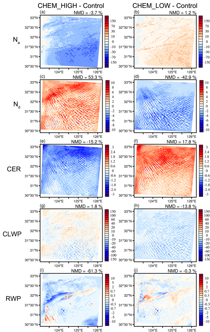
Figure 11. Same as Fig. 3, but showing differences in each variable ( N_a : a–b , in \text{cm}^{-3} ; N_d : c–d , in \text{cm}^{-3} ; CER: e–f , in \mu\text{m} ; CLWP: g–h , in \text{g m}^{-2} ; RWP: i–j , in \text{g m}^{-2} ) between the CHEM_HIGH (left column) and CHEM_LOW (right column) experiments and the Control experiment.
