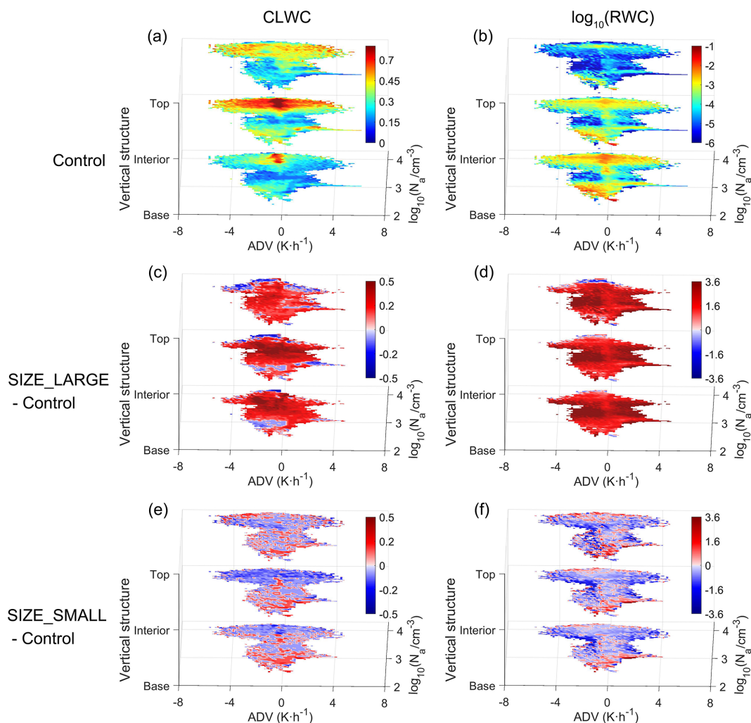
Figure 7. Variation of CLWC (left column, unit: \text{g m}^{-3} ) and RWC (right column, unit: \text{g m}^{-3} , presented logarithmically in base 10) with N_a , ADV and cloud parts for the Control (a–b) experiment, and the differences of the SIZE_LARGE (c–d) and SIZE_SMALL (e–f) experiments relative to the Control experiment.
