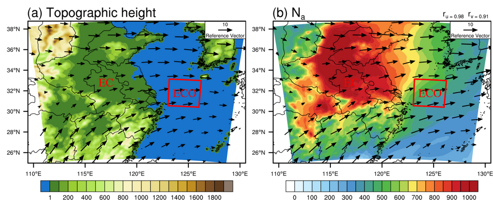
Figure 1. Topographic map of the outer domain ( a , in m) and the distribution of column-mean N_a of the Control experiment ( b , in \text{cm}^{-3} ) during the simulation period. The locations of EC and ECO are highlighted in red text, with the ECO extent (i.e., the inner domain) indicated by a red box. The time-averaged wind fields in ( a ) and ( b ) are derived from MICAPS data and the Control simulation, respectively. The values r_u and r_v in the upper-right corner of ( b ) denote the Pearson product-moment correlation coefficients for the u and v wind components between MICAPS and the simulation.
