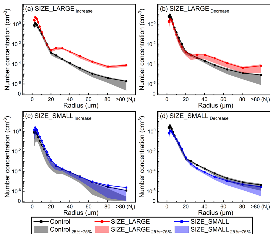
Figure 5. Changes in droplet spectra (lines, mean; shading, the 25 %–75 % interquartile range; droplets with a radius greater than 80 \mu\text{m} are raindrops and those less than 80 \mu\text{m} are cloud droplets) for the samples with an increase (a, c) or decrease (b, d) in N_d of more than 0.1 \text{ cm}^{-3} , in response to increases (upper row) or decreases (lower row) in aerosol size.
