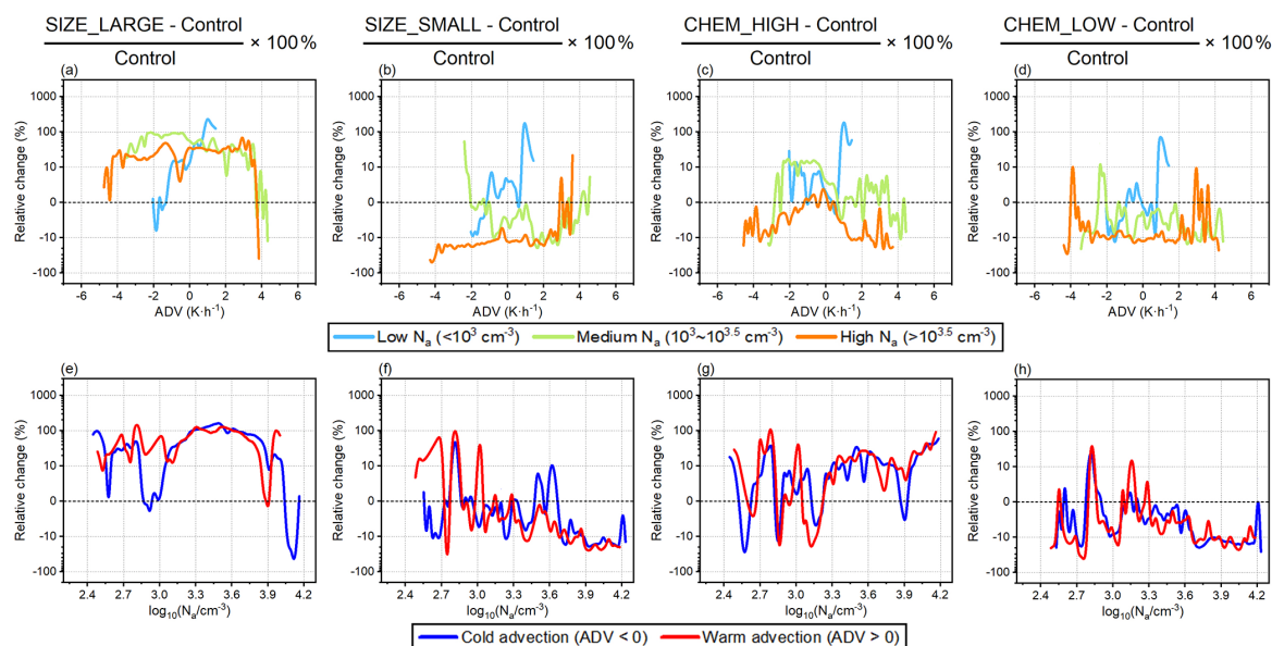
Figure 10. Percentage changes in CLWC for the SIZE_LARGE (first column), SIZE_SMALL (second column), CHEM_HIGH (third column), and CHEM_LOW (fourth column) experiments relative to the Control experiment. The first row: dependence on ADV ( x axis) for different N_a conditions; the second row: dependence on N_a ( x axis) for different ADV conditions.
