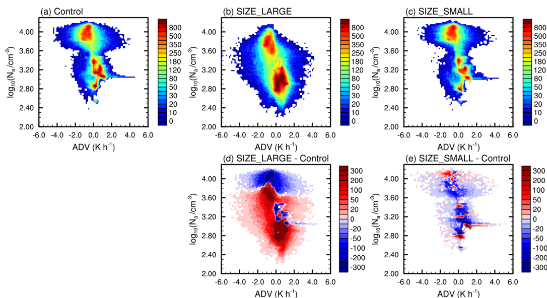
Figure 8. Variation of cloud lifetime (characterized by liquid-phase cloud sample count) with ADV and N_a . (a), (b), (c), (d), and (e) are the results of the Control, SIZE_LARGE, and SIZE_SMALL experiments, and the differences of SIZE_LARGE and SIZE_SMALL experiments relative to the Control experiment, respectively.
