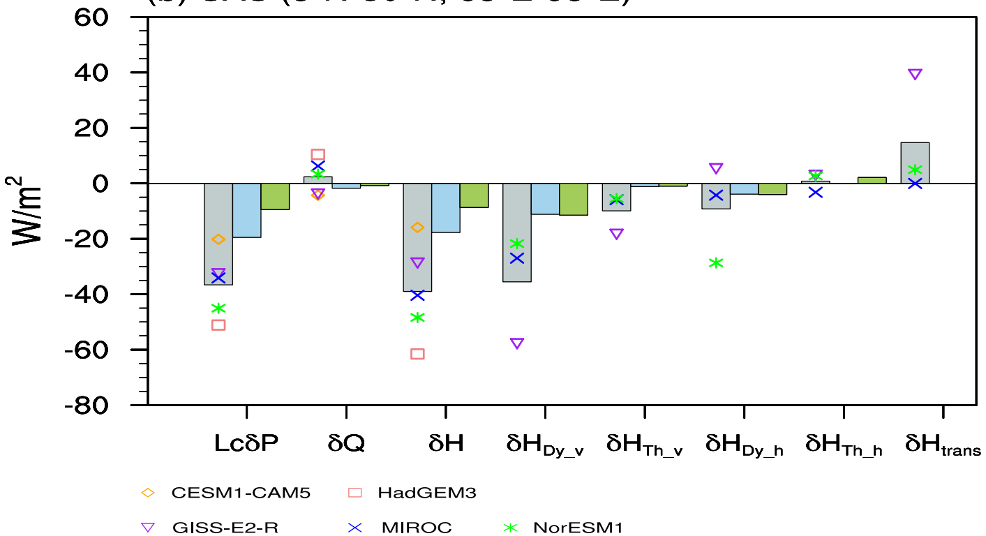
(b) SAS (5°N-30°N, 65°E-95°E)
