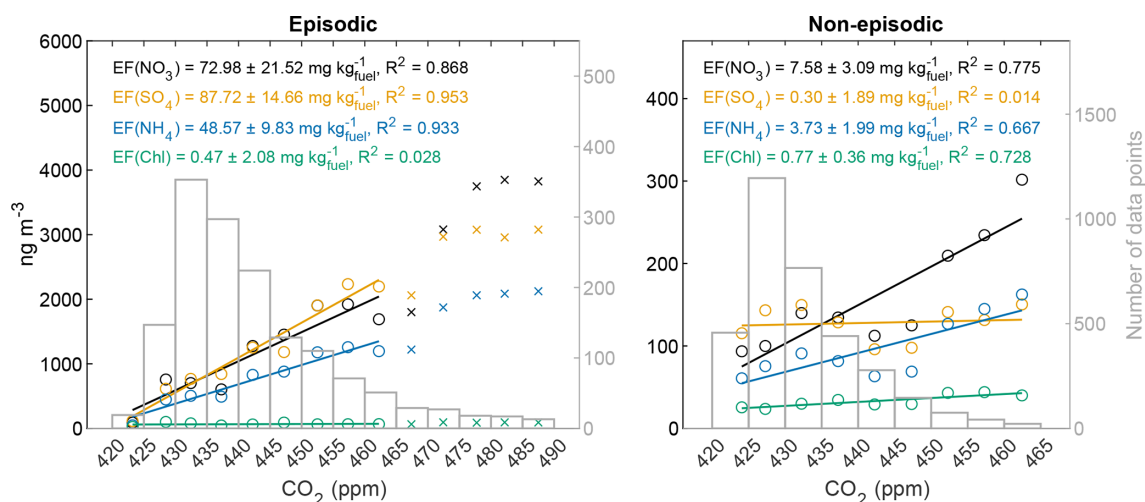
Figure 6. Concentrations of nitrates ( NO_3 ), sulphates ( SO_4 ), ammonium ( NH_4 ) and chloride (Chl) as a function of CO_2 concentration and the determined EFs, including 95 % confidence intervals and R^2 of the averaged linear fits. The episodic data on left and non-episodic data on right. Notice the different x- and y-axes. Also, the number of data points in each CO_2 concentration bin is shown. See Fig. S14 for organics.
