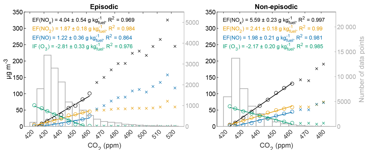
Figure 3. \text{NO}_x , \text{NO} , \text{NO}_2 and \text{O}_3 concentrations as a function of \text{CO}_2 concentration and the determined EFs for \text{NO}_x , \text{NO} , \text{NO}_2 and the inverse IF for \text{O}_3 , including 95 % confidence intervals and R^2 of the averaged linear fits. The episodic data on left and non-episodic data on right. Notice the different x-axis. Also, the number of data points in each \text{CO}_2 concentration bin is shown.
