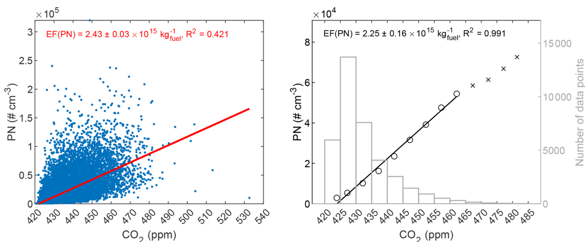
Figure 1. Left: Scatter plot of all individual non-episodic 1 min-average PN and \text{CO}_2 concentrations, together with a linear fit. Right: Average (geometric mean) PN and \text{CO}_2 concentrations over 5 ppm \text{CO}_2 concentration bins, together with a linear fit, which was calculated in the range of 420–465 ppm of \text{CO}_2 (circular markers). Also, the number of data points (1 min) in each \text{CO}_2 concentration bin shown is shown in the histogram.
