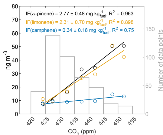
Figure 5. Concentrations of selected terpenoids ( \alpha -pinene, limonene and camphene) as a function of \text{CO}_2 concentration and the determined IFs with 95 % confidence intervals and R^2 of the averaged linear fits. Also, the number of data points in each \text{CO}_2 concentration bin is shown.
