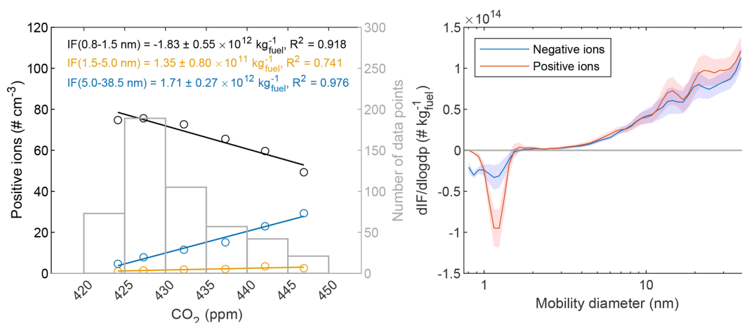
Figure 4. Left: Concentrations of selected positive ions in the size ranges of 0.8–1.5, 1.5–5.0 and 5.0–38.5 nm as a function of CO 2 concentration and the determined IFs with 95 % confidence intervals and R^2 of the averaged linear fits. Also, the number of data points in each CO 2 concentration bin is shown. Right: Size-resolved IFs of negative and positive ions with 95 % confidence intervals (shaded areas).
