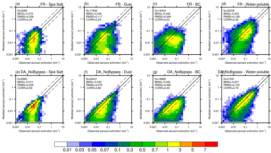
Figure S3. Same as Fig. 3 but for DA_NoBypass experiment.
