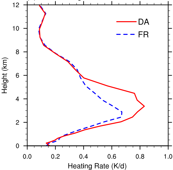
(a) SW Heating Rate
