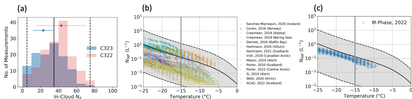
Figure 3. Comparison between the perturbed range and the measurements: (a) N_d with measured in-cloud N_d from M-Phase C322 and C323 using the CDP (cloud droplet probe) onboard, and N_d (mean \pm one standard deviation) calculated based on retrievals from MODIS instrument onboard the Aqua satellite; (b) perturbed temperature-dependent N_{\text{INP}} ranges compared to INP measurements at high latitudes in the Northern Hemisphere (Sanchez-Marroquin et al., 2020; Franz Conen, 2016; Creamean et al., 2018, 2019; DeMott et al., 2016; Hartmann et al., 2020, 2021; Irish et al., 2019; Mason et al., 2016; Porter et al., 2020, 2022; Si et al., 2019; Welti et al., 2020; Raif et al., 2024); (c) perturbed temperature-dependent N_{\text{INP}} ranges compared to all INP measurements from the M-Phase campaign (Tarn et al., 2025). Boundaries of each perturbed range (maximum and minimum values) are shown with dashed black lines, and the values used for the control simulations are shown with solid black lines. Cloud top temperatures are around -15^{\circ}\text{C} for the CAO clouds in this case and -15^{\circ}\text{C} is marked with bold gray solid line in (b) and (c).
