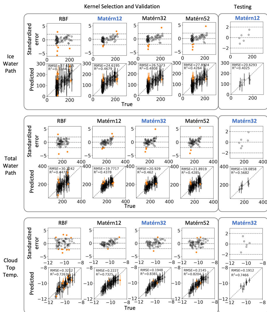
Figure C4. Kernel selection and testing results of the GP emulators on IWP, TWP, and cloud top temperature in the Cu model analysis region. Points in orange indicate a failed emulated point in the standardized error check. The kernel name highlighted in blue indicates that the kernel was selected and the testing results are from comparing the emulator trained with the selected kernel with the testing dataset.
