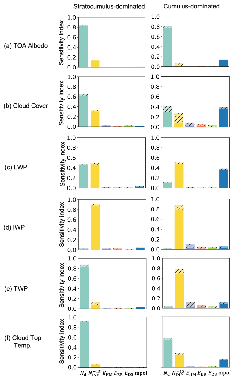
Figure G1. Sensitivity indices of all the perturbed parameters for TOA albedo (unitless), cloud cover (unitless), all-sky LWP ( \text{g m}^{-2} ), all-sky IWP ( \text{g m}^{-2} ), all-sky TWP ( \text{g m}^{-2} ), and cloud top temperature ( ^{\circ}\text{C} ). Each sensitivity index consists of the first-order, main effect (solid fill) and the second-order, interactive effects (dashed). Indices are shown separately for the Sc (left column) and Cu (right column) regions.
