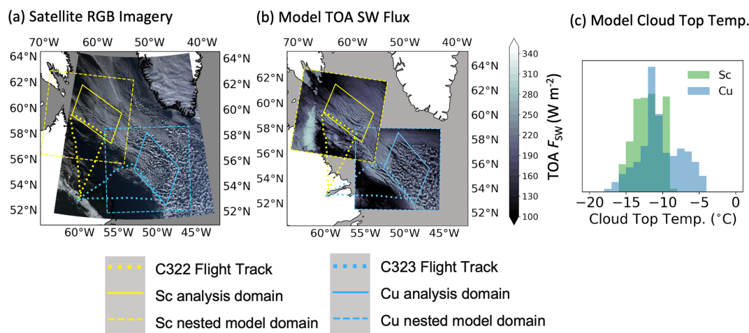
Figure 1. Flight tracks (dotted line), nested model domains (dashed squares) and model analysis domains (solid rectangles) for Sc region (yellow) and Cu region (blue) on 24 October 2022 over the Labrador Sea: (a) the RGB satellite imagery created using bands 1 (620–670 nm), 3 (459–479 nm), and 4 (545–565 nm) from MODIS (Moderate Resolution Imaging Spectroradiometer) Level 1B Calibrated Radiances Product (Collection 6.1) (MODIS Characterization Support Team (MCST), 2017) onboard the Aqua satellite, (b) the SW (shortwave) reflectance at the top-of-the-atmosphere from the control simulations. The selected model time is the same as the satellite retrieval time at 17:00 UTC and the model output fields are instantaneous. Cloud top temperatures in the two analysis domains are shown in (c) . The cloud top temperatures were derived using the air temperature at the highest model grid in a column, with a cloudy grid defined using total cloud water content \geq 10^{-6} \text{ kg kg}^{-1} . The model output time for CTT in the Sc region is 14:00 UTC and is 19:00 UTC in the Cu region for the corresponding times of flights. The temperature profiles were evaluated in our previous work (Huang et al., 2025).
