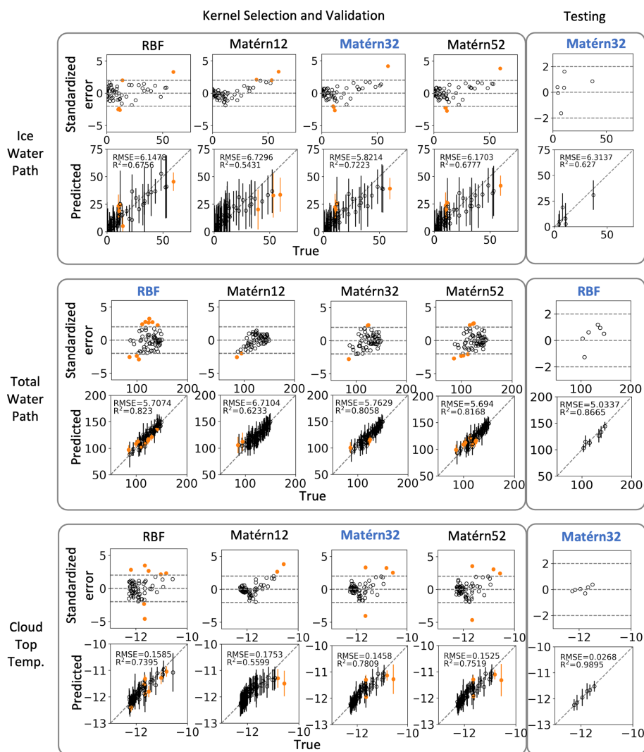
Figure C2. Kernel selection and testing results of the GP emulators on IWP, TWP, and cloud top temperature in the Sc model analysis region. Points in orange indicate a failed emulated point in the standardized error check. The kernel name highlighted in blue indicates that the kernel was selected and the testing results are from comparing the emulator trained with the selected kernel with the testing dataset.
