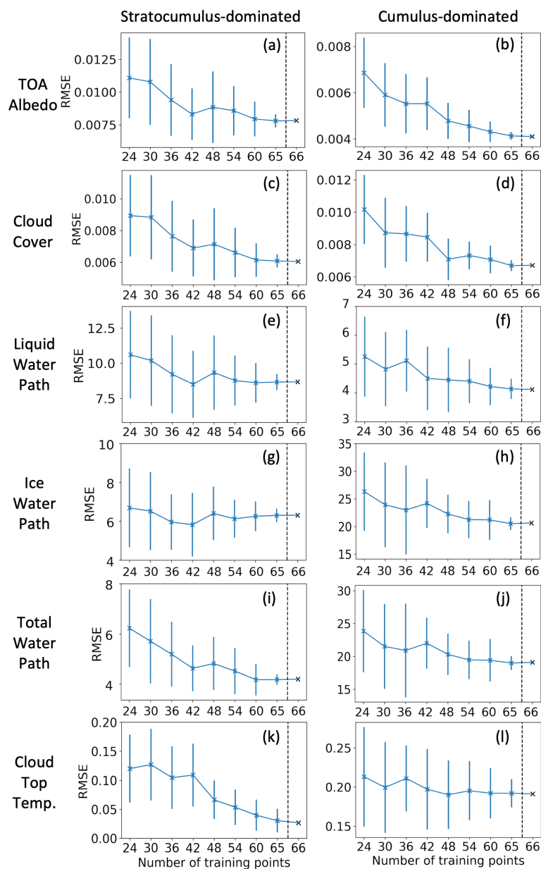
Figure C5. Convergence test results (RMSE) by using different number of training points over the Sc region (left) and the Cu region (right) for: (a, b) TOA albedo (unitless), (c, d) cloud cover (unitless), (e, f) liquid water path ( \text{gm}^{-2} ), (g, h) ice water path ( \text{gm}^{-2} ), (i, j) total water path ( \text{gm}^{-2} ), and (k, l) cloud top temperature ( ^{\circ}\text{C} ).
