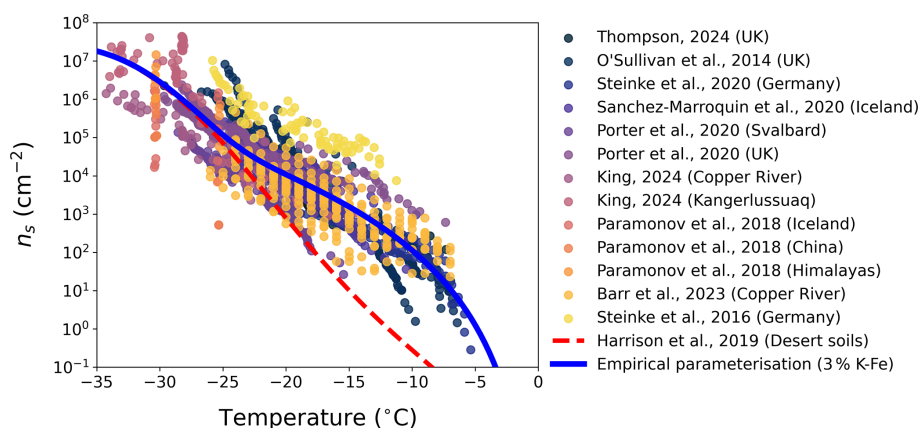
Figure A1. Empirical soil-dust parameterisation of n_{s,\text{soil}}(T) . Coloured circles show measurements from laboratory studies (references within figure) that have measured the ice-nucleating activity of soil dust sampled from locations around the world. The red dashed line shows the parameterisation for desert soils from Harrison et al. (2019), whilst the solid blue line shows the best fit to the data assuming a K-Fe component (weight percent of 3%) and a biogenic component described by a power law.
