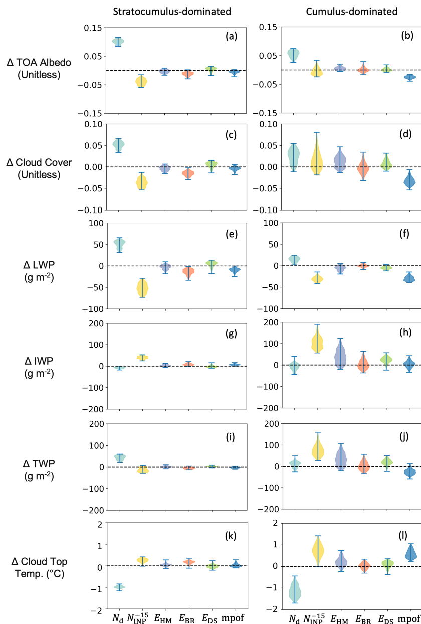
Figure 9. Distributions of the cloud property changes resulting from an increase of individual parameters one-at-a-time (OAT) in multiple OAT tests for: all-sky TOA albedo (a, b), cloud cover (c, d), all-sky LWP (e, f), all-sky IWP (g, h), all-sky TWP (i, j) and cloud top temperature (k, l). The left panel shows the results from the Sc region, and the right panel shows the results from the Cu region. Errors of the GP model are propagated through into these multiple OAT test results, but the errors are generally much smaller than the variations shown here (Appendix C). For the process of performing the multiple OAT test, please refer to the details in Sect. 3.3.
