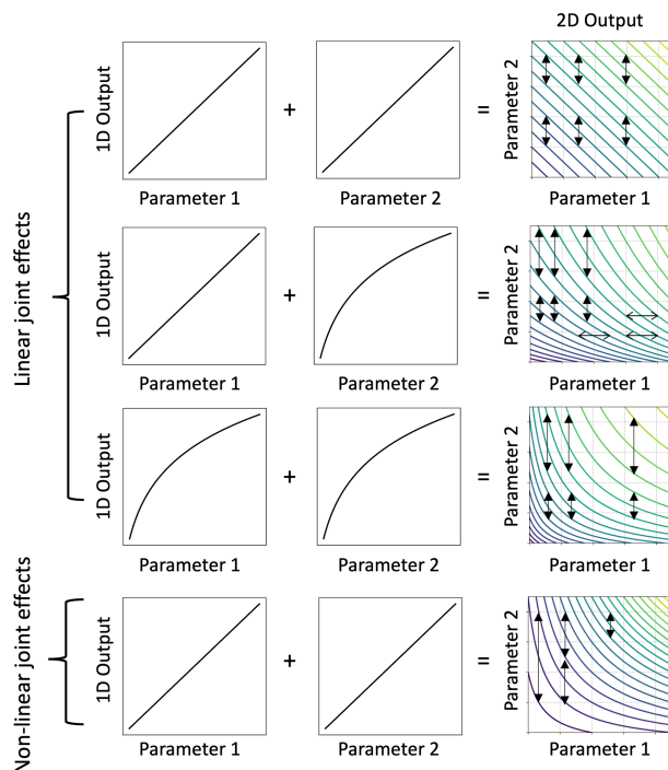
Figure E1. A simple illustration of linear and non-linear joint effects between two parameters. This diagram is adapted from Fig. 3.3 in the work of Sansom (2023). With linear joint effects, the effect of changing one parameter on the model output is independent of the value of the other parameter. With non-linear joint effects, the effect of changing one parameter on the model output is then dependent on the value of the other parameter. The length of the arrows shown in the 2D output represents the variation needed for a parameter to across three contour lines. All the contour lines shown here are with linear scale.
