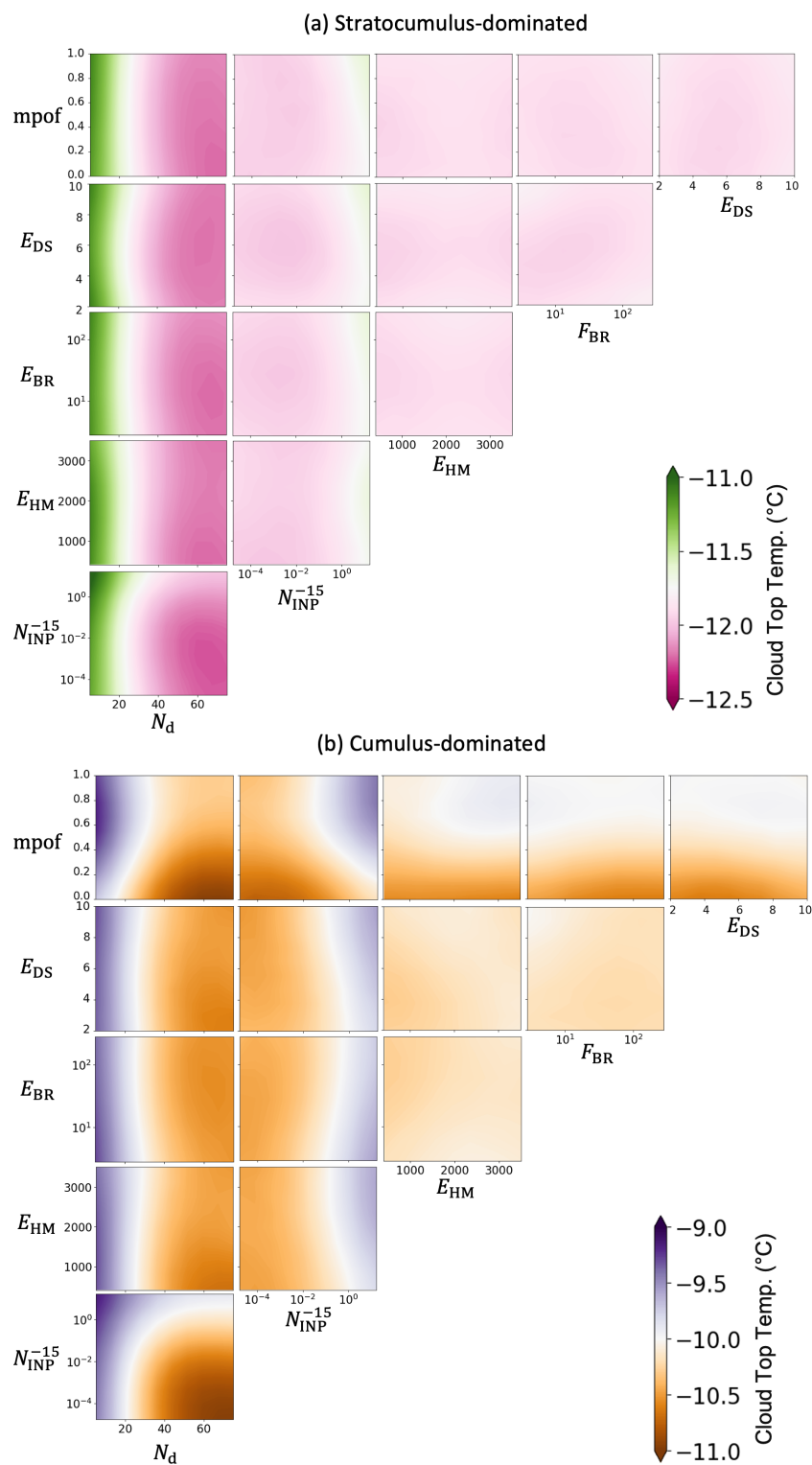
Figure F4. Projected mean model responses of cloud top temperature to paired parameters in (a) Sc region and (b) Cu region.
