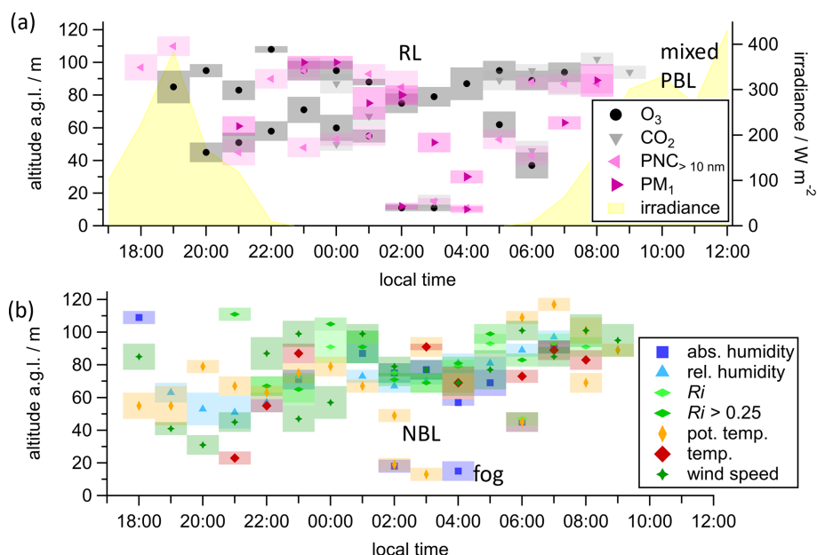
Figure 1. Estimated boundary layer heights (solid markers, with uncertainty ranges depicted as shaded areas) during the night of 20 to 21 June 2024. The boundary layer heights were derived from strongest gradient changes of the respective trace matter variables (a) and meteorological variables (b) and when the criterion Ri > 0.25 was fulfilled. The yellow shaded area in (a) represents the measured irradiance, which was reduced by cloudiness in the afternoon and the late morning.
