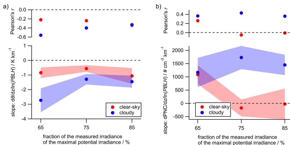
Figure 3. Influence of the irradiance threshold as a criterion to separate “clear-sky” (red) and “cloudy” days (blue) on the dependency of d\theta/dz and d\text{PNC}_{>10\text{nm}}/dz on the PBLH (in m). Pearson’s correlation coefficient r and slopes of the respective gradients versus the logarithm of the PBLH are depicted with 1\sigma -confidence bands. The classification criteria are the ratios of the measured irradiance in respect to the maximal potential irradiance.
