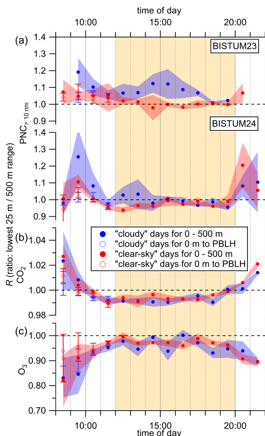
Figure 5. A diurnal variation the representativity R of \text{PNC}_{>10\text{nm}} (a), \text{CO}_2 (b) and \text{O}_3 (c) of ground-based measurements for the 500 m-column above. Open markers represent ratios calculated for measurements solely within the PBLH, when PBLH was lower than 500 m. The yellow shading represents hours with the PBLH being higher than 500 m. Propagated uncertainty for data points derived from the whole 500 m and from ground to the PBLH are represented as shaded areas and error bars as 1\sigma -uncertainties, respectively.
