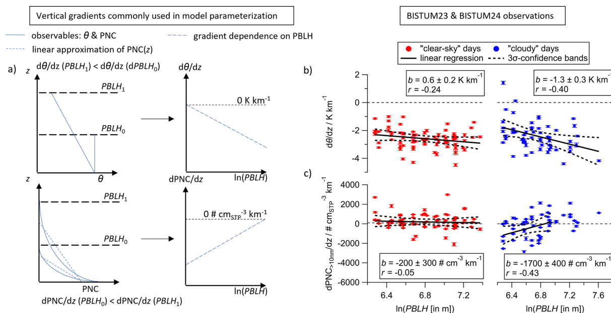
Figure 2. (a) Schematic description of the dependency of atmospheric stability (reflected by \theta(z) , with the altitude z ) and a pollutant with source at ground level ( PNC(z) ) on altitude for the well-mixed planetary boundary layer with a height PBLH_i as commonly used in model parameterizations (a, left). Deriving the dependence of d\theta/dz and dPNC/dz from PBLH results in a linear-logarithmic dependency of respective gradients on the boundary layer height (a, right). Experimental data of gradients of the potential temperature \theta (b) and the particle number concentration PNC_{>10nm} (c) in the lowermost 500 m in a mixed PBL from both campaigns are plotted versus associated logarithms of respective planetary boundary layer heights ( PBLH , in m). Linear regression with the slope b and its 3 \sigma -confidence bands are depicted in solid and dotted lines.
