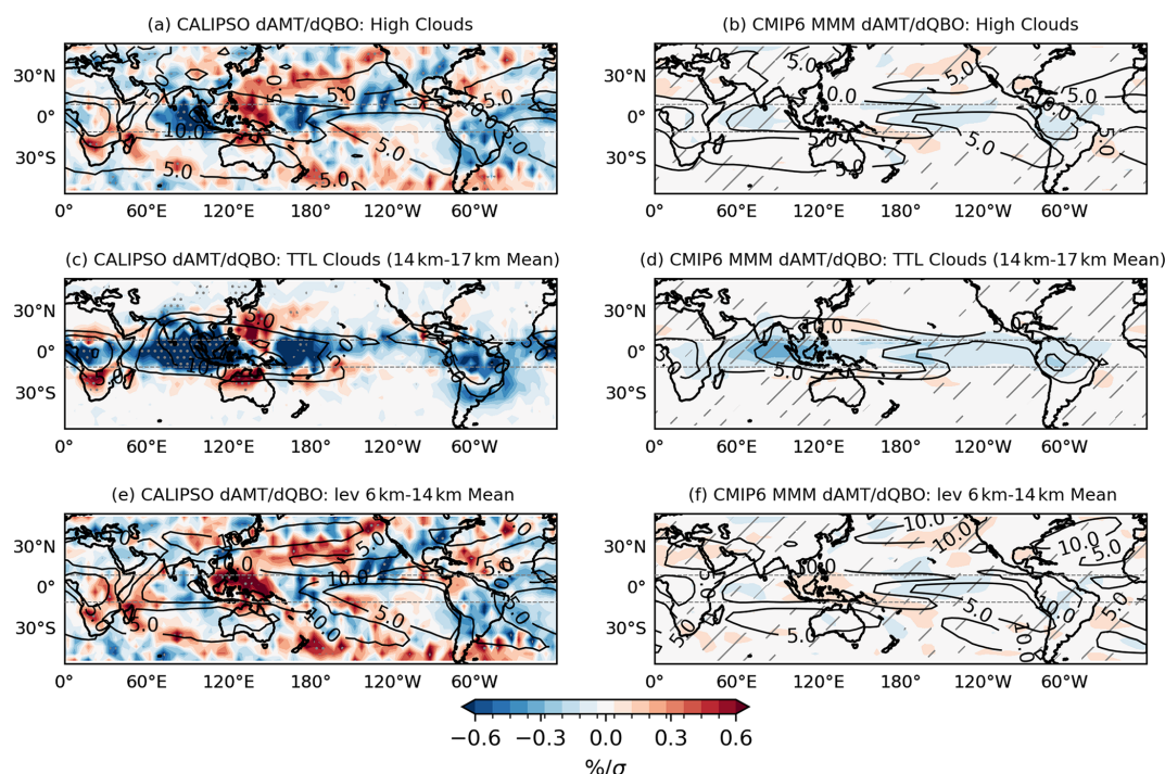
Figure 2. QBO regressed high-cloud fraction ( < 440 hPa), TTL cloud fraction ( < 180 hPa), and 440–180 hPa cloud fraction in CALIPSO (a, c, e) and CMIP6 MMM (b, d, f), represented in units of standard deviation of the QBO index. Overlaid line contours indicate the climatology of respective cloud fraction. Stippling in (a), (c) and (e) denotes 90 % confidence, and hatching in (b), (d) and (f) denotes six out of 7 models having the same sign.
