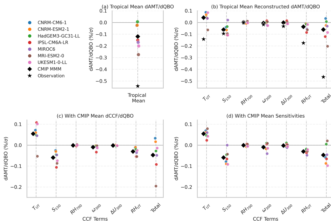
Figure 5. (a) Tropical mean ( 10^{\circ}\text{S} – 10^{\circ}\text{N} ) of QBO-regressed TTL cloud fraction in observations, CMIP6 models and the MMM. (b) Individual CCF contributions to the tropical-mean QBO-induced TTL cloud response and the total. (c) Same as (b) but replacing model-specific QBO-regressed CCF anomalies with the MMM CCF responses. (d) Same as (b) but replacing model-specific cloud sensitivities with the CMIP6 MMM sensitivities. Changes are per unit standard deviation of QBO.
