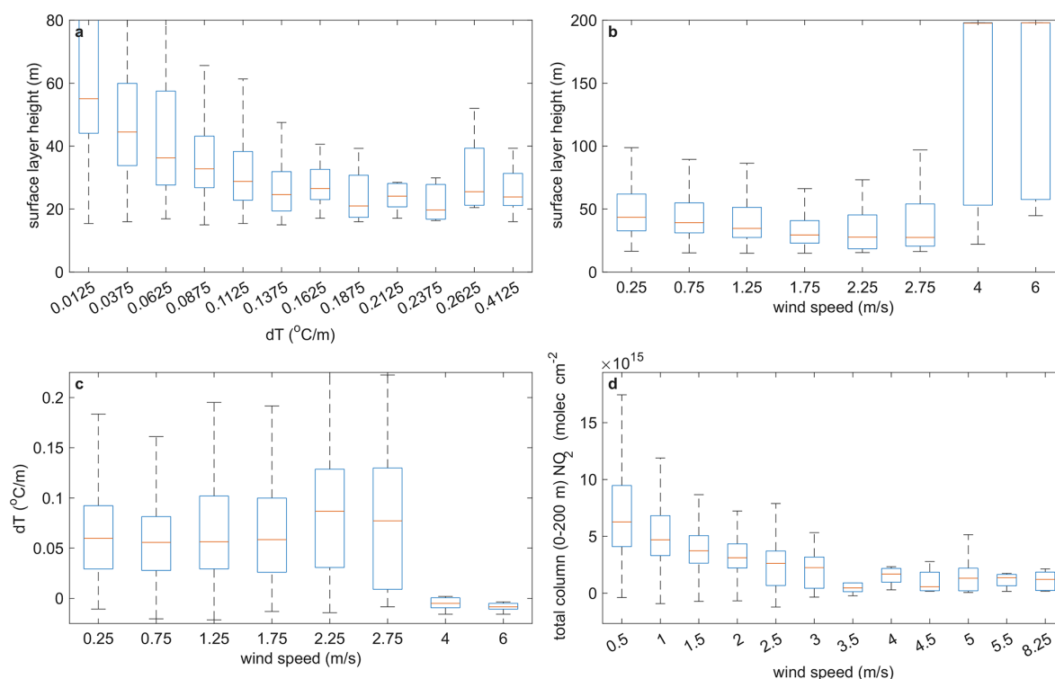
Figure 4. Statistical analysis of the dependence of (a) surface layer height on temperature gradient; (b) surface layer height on 23 m wind speed; (c) surface temperature gradient on wind speed, and (d) \text{NO}_2 column density on wind speed.
