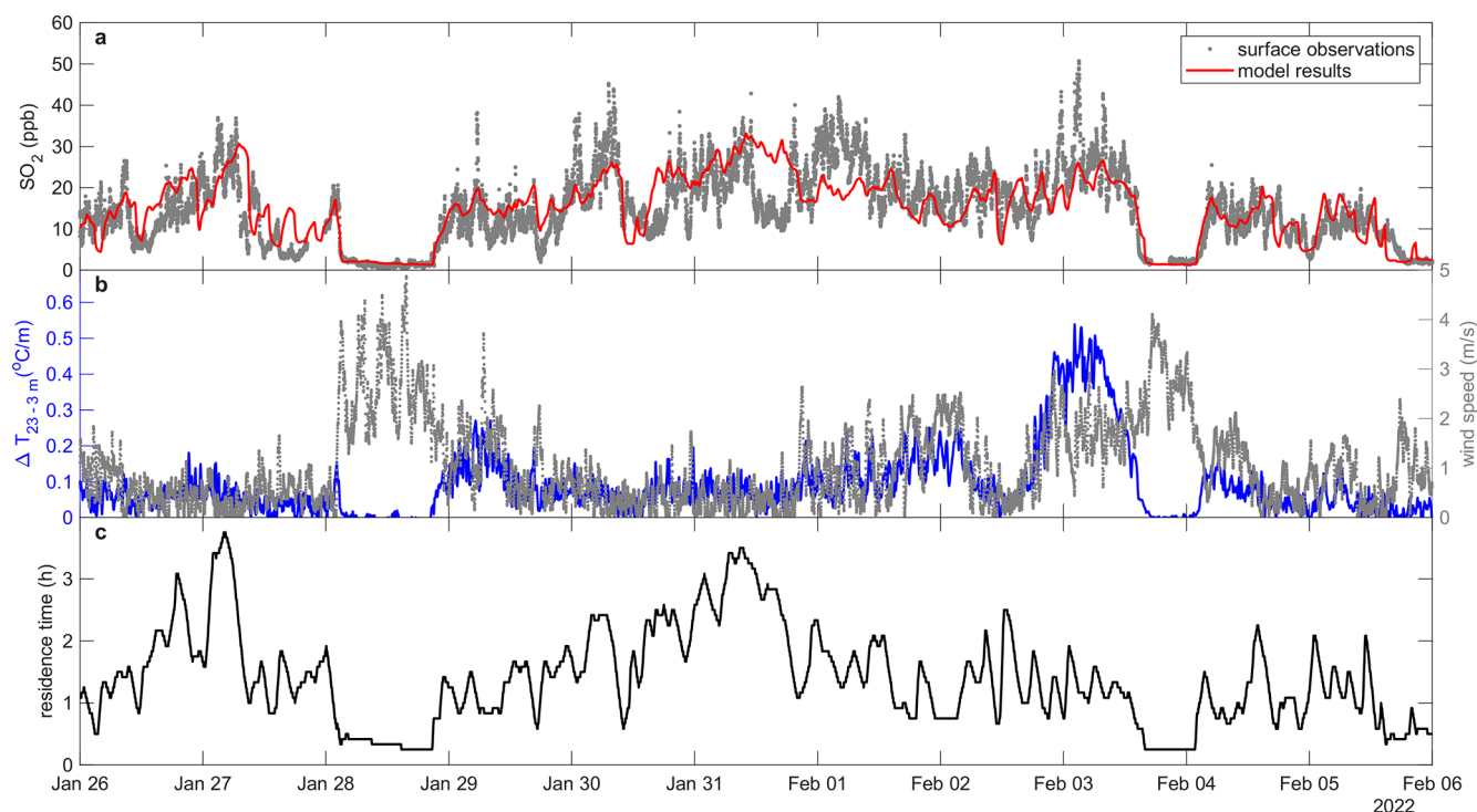
Figure 10. Observed and modeled \text{SO}_2 (a) shows the variability imposed by PSL transport processes, which are associated with surface temperature gradients and wind speed (b, shown after applying a 15 min running average). The residence time determined from the model (c) shows low values at times of wind speeds exceeding 2 \text{ m s}^{-1} . Residence times of 1 h or longer are associated with the presence of temperature inversions.
