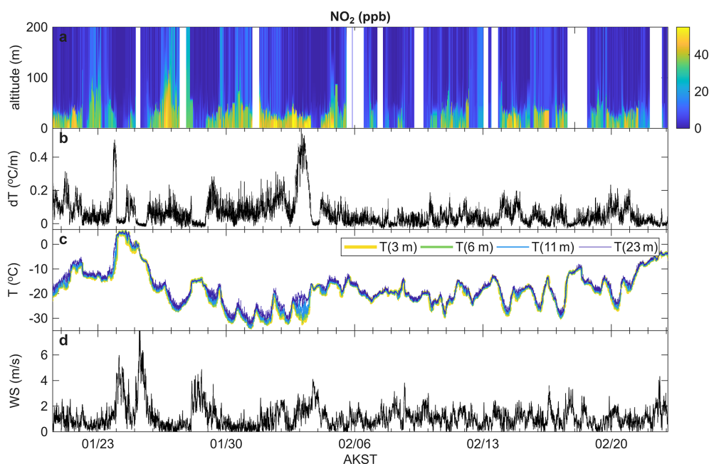
Figure 3. Retrieved vertical profiles of NO 2 (a) compared to temperatures at 3, 6, 11, and 23 m (c) and temperature gradients (b). Wind speeds at 23 m are displayed in panel (d).
