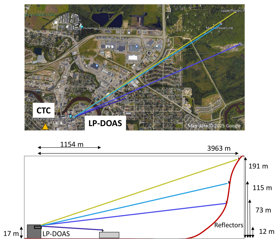
Figure 1. Sketch of the LP-DOAS instrument and location of absorption paths and in-situ observations. In-situ measurements were located at the CTC building marked by the yellow triangle. The distance between the LP-DOAS and the CTC building is approximately 500 m.
