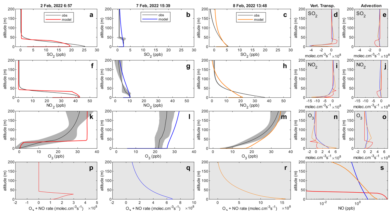
Figure 8. Examples of retrieved and modeled vertical mixing ratio profiles of \text{SO}_2 , \text{NO}_2 , and \text{O}_3 . The shaded area shows the profile uncertainty due to the measurement error. Shaded panels on the right depict the modeled vertical and advective transport rates of \text{SO}_2 (d, e), \text{NO}_2 (i, j), and \text{O}_3 (n, o). The bottom three panels (p–r) show the vertical profiles of the \text{O}_3 + \text{NO} reaction rate for the three examples, where the respective NO vertical profiles from the model are shown in panel (s).
