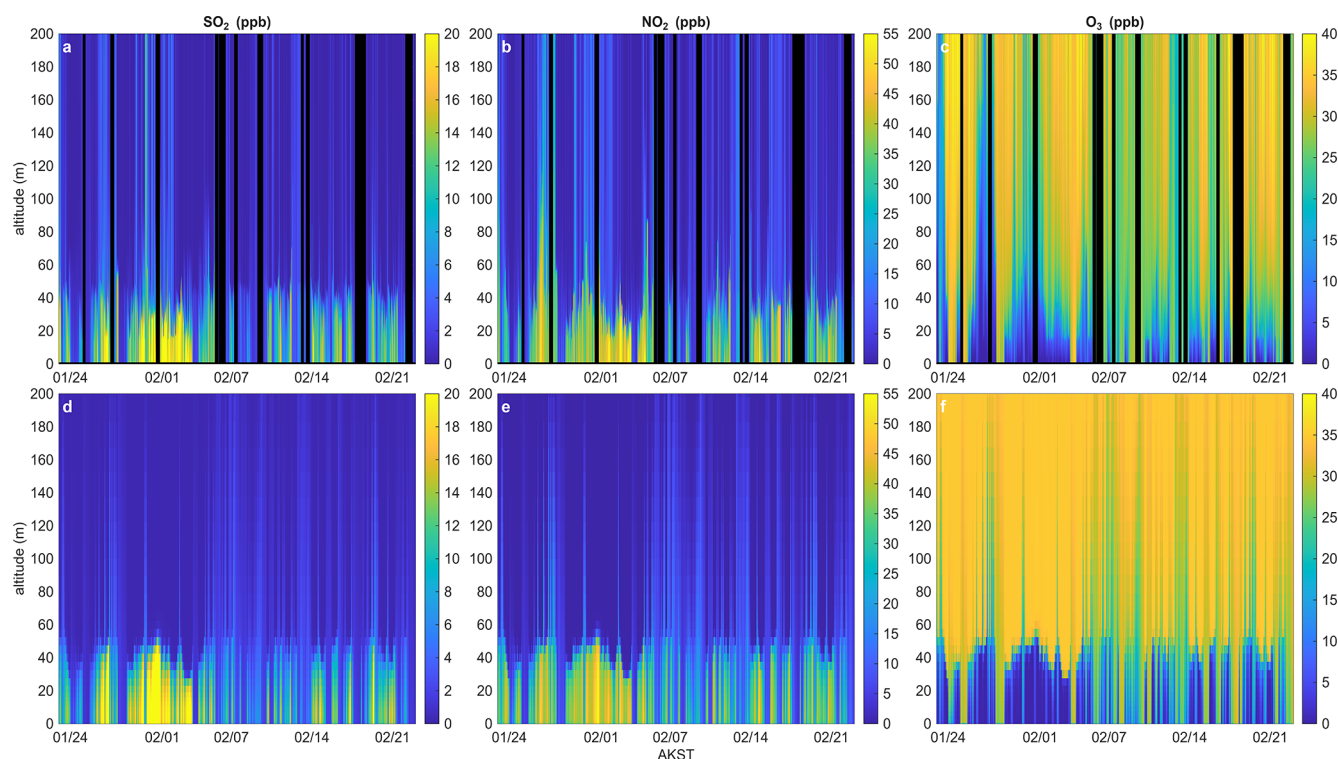
Figure 6. Campaign overview of retrieved (a–c) and modeled (d–f) vertical mixing ratio profiles of SO 2 (a, d), NO 2 (b, e), and O 3 (panels c, f).
