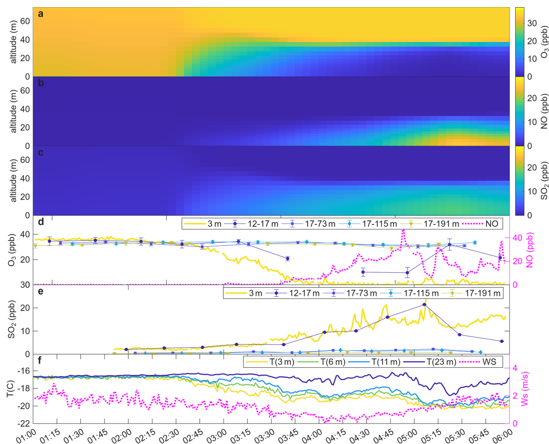
Figure 9. Formation of the PSL on 4 February 2022. The top three panels (a–c) show the model results for this event. Panel (d) shows the path-averaged LP-DOAS and in-situ ozone data (left y axis) and the surface NO data (magenta, right y axis). The light path above 17 m height shows a constant O 3 mixing ratio of ~ 35 ppb, while the PSL mixing ratios drop at the onset of the event at around 02:45 AKST. Panel (e) shows the observations of SO 2 for LP-DOAS and in-situ data. The PSL observations of the two instruments agree very well, and also show an increase in SO 2 during this event. Temperature gradients (panel f, left y axis) form around 02:15 AKST, during a time when the wind speed (magenta, right y axis) is around 2 m s -1 .
