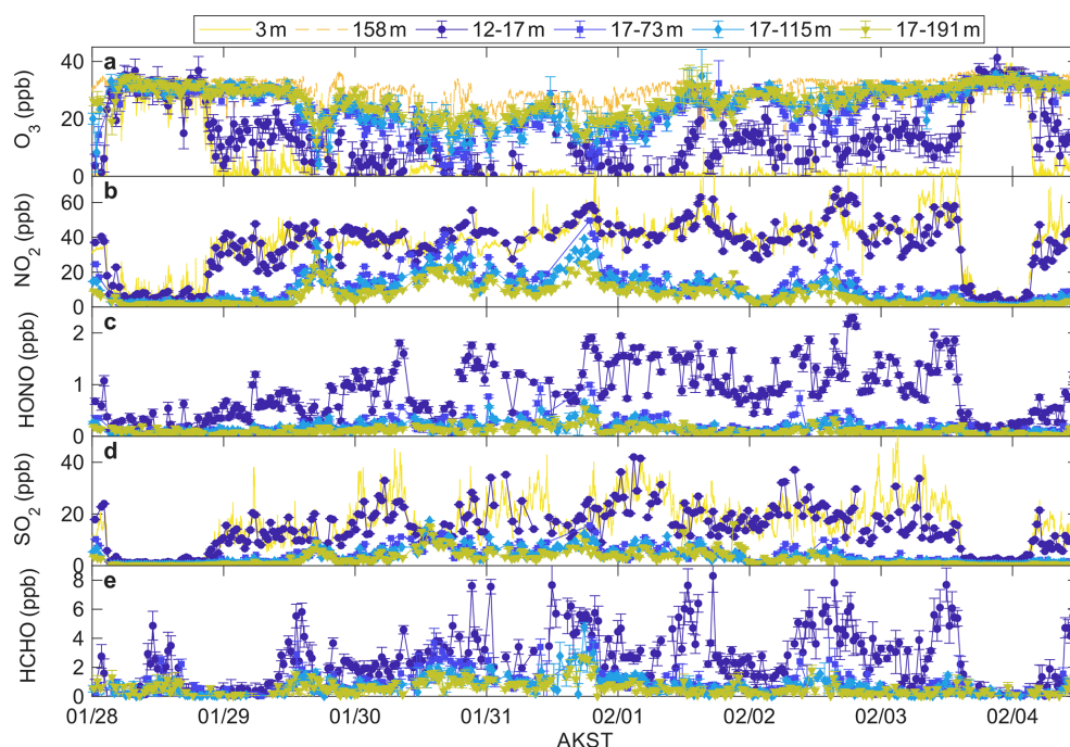
Figure 2. Overview of one week of path-averaged LP-DOAS data along the four different lightpaths using the same color coding as in Fig. 1. Surface (3 m) in-situ data is shown as a yellow line, while the Birch Hill data (158 m) is shown as a dashed dark yellow line. The full dataset is shown in Fig. S1.
