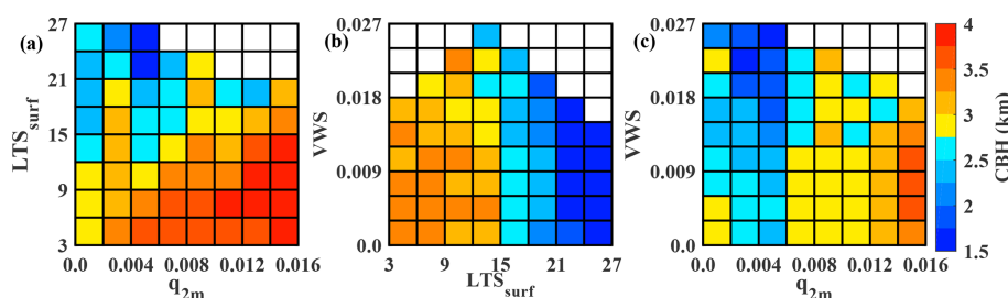
Figure 9. Bivariate regulation of CBH by thermodynamic and dynamical factors across China in 2024, based on observations from 80 MMCR stations. Each panel illustrates the response of CBH to the combined modulating effects of a specific pair of key atmospheric factors: (a) LTS_{surf} and q_{2m} , (b) VWS and LTS_{surf} , and (c) VWS and q_{2m} . All ERA5 reanalysis variables were spatially and temporally matched with MMCR data to ensure the validity and reliability of this bivariate joint dependence analysis.
