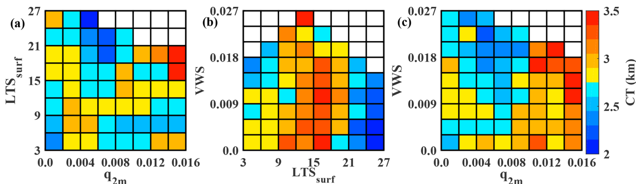
Figure 13. Similar as Fig. 9, but for CT.
