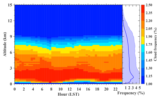
Figure 6. Annual mean diurnal cycle of height-resolved cloud occurrence frequency and corresponding vertical profiles derived from measurements at all 80 MMCR stations (Fig. 1) across China in 2024. Data samples are binned at a vertical resolution of 200 m and a temporal resolution of 30 min. Cloud occurrence frequency at a given altitude is defined as the ratio of cloudy samples at that altitude to the total number of cloudy samples across all altitudes. Also presented are the corresponding vertical probability distributions of clouds.
