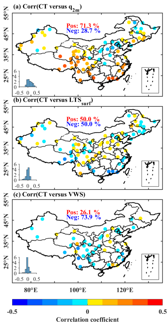
Figure 12. Similar as Fig. 8, but for CT.
