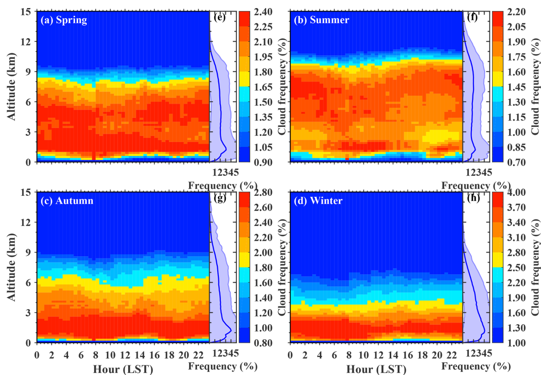
Figure 7. Similar to Fig. 6, but for the seasonal mean diurnal cycle of height-resolved cloud occurrence frequency and corresponding vertical profiles over China in (a) spring, (b) summer, (c) autumn, and (d) winter.
