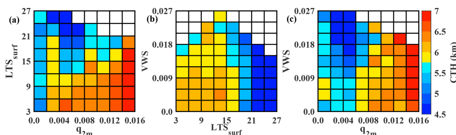
Figure 11. Similar as Fig. 9, but for CTH.
