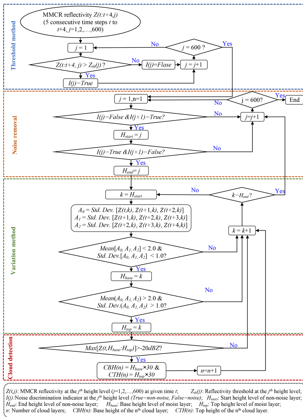
Figure 2. Flowchart for identifying the cloud vertical structure (CVS) from high-temporal-resolution MMCR measurements. This flowchart comprises four sequential key steps in the CVS retrieval process: first, the threshold method involves comparing the MMCR reflectivity Z(t : t + 4, j) against the height-dependent threshold Z_{th}(j) to generate the noise discrimination indicator I(j) , which distinguishes non-noise and noise layers; subsequently, the noise removal step identifies the start ( H_{start} ) and end ( H_{end} ) height levels of non-noise layers based on the indicator I(j) ; then, the variation method determines the base ( H_{base} ) and top ( H_{top} ) height levels of moist layers by calculating the statistical variation (including standard deviation and mean) of reflectivity within the identified non-noise layers; finally, the cloud detection step retrieves the base height ( CBH(n) ) and top height ( CTH(n) ) of each cloud layer by verifying the reflectivity magnitude of the moist layers, thereby yielding the final cloud vertical structure.
