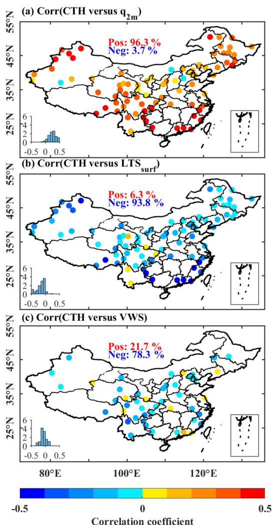
Figure 10. Similar as Fig. 8, but for the CTH.
