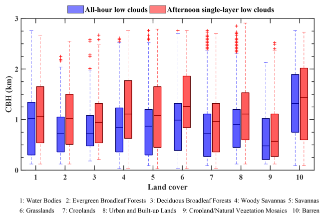
Figure 14. Land-surface influence on CBH across China in 2024, based on 80 MMCR stations. Blue bars indicate all-hour low clouds, and red bars represent afternoon single-layer low clouds. Land cover types are derived from the MODIS Land Cover Type Yearly Climate Modeling Grid product (MCD12C1; https://lpdaac.usgs.gov/products/mcd12c1v061/ , last access: 12 September 2026).
