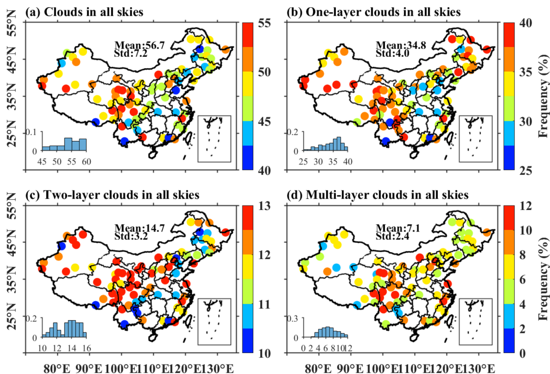
Figure 3. Spatial distribution of annual mean cloud occurrence frequency for different cloud layering classifications: (a) all clouds, (b) single-layer clouds, (c) two-layer clouds, and (d) multi-layer clouds (three-, four-, and five-layer clouds) under all-sky conditions in 2024. The data is derived from the 80 MMCR stations presented in Fig. 1. Notably, the color bars are scaled independently across panels to improve visual clarity. In addition, each panel shows the histograms depicting the probability distributions of cloud occurrence frequencies, with the corresponding mean values and standard deviations also presented for each distribution.
