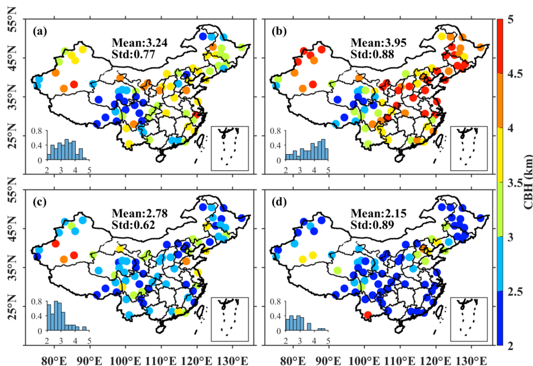
Figure 4. Seasonal geographic distribution of cloud base height (CBH) over China in 2024, derived from the 80 MMCR stations of the same network referenced in Fig. 1. The four panels correspond to (a) spring (March–April–May), (b) summer (June–July–August), (c) autumn (September–October–November), and (d) winter (December–January–February). Note that each panel presents a histogram illustrating the probability distribution of cloud occurrence frequency, with the corresponding mean value and standard deviation provided for each distribution.
