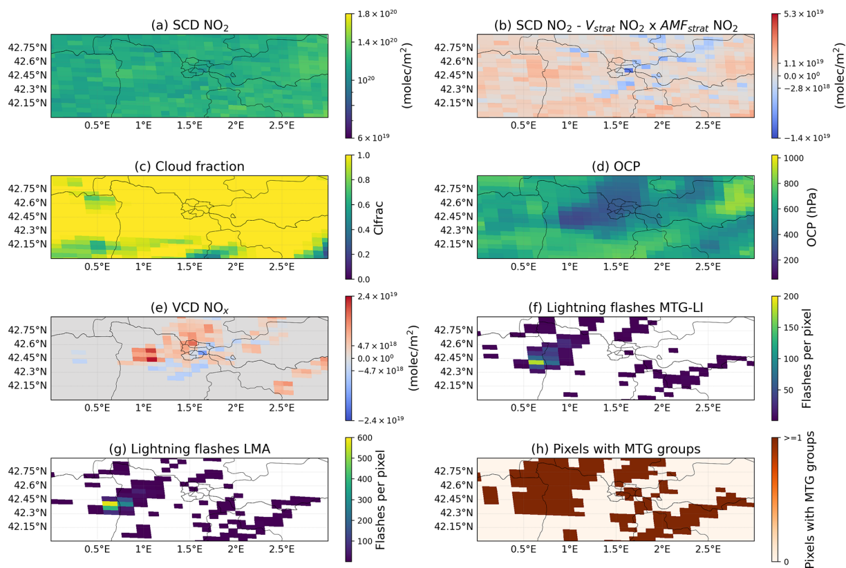
Figure 5. TROP-DLR product of orbit 34875, Meteosat 12 LI and LMA lightning data for the case 6 July 2024. (a) Slant Column Density (SCD) \text{NO}_2 provided by the TROP-DLR \text{NO}_2 research product. (b) SCD \text{NO}_2 minus the stratospheric vertical column density multiplied by the stratospheric air mass factor of \text{NO}_2 ( \text{AMF}_{\text{strat}} ) obtained from the TROP-DLR \text{NO}_2 research product. (c) and (d) Cloud Fraction (CF) and Optical Centroid Pressure (OCP) from the TROP-DLR \text{NO}_2 research product, respectively. (e) VCD \text{NO}_x ( V_{\text{tropNO}_x} from Eq. 3) over pixels satisfying the Deep Convective Constraint (DCC). (f) and (g) Lightning flashes during the 5 h period per TROPOMI pixel before the TROPOMI overpass reported by Meteosat 12 LI and the LMA, respectively. (h) TROPOMI pixels containing at least one lightning group detected by Meteosat 12 LI. Sentinel-5P TROPOMI data © ESA, processed by DLR. Meteosat 12 LI lightning data © EUMETSAT.
