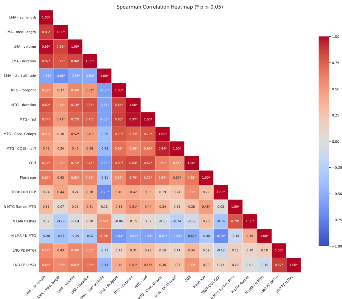
Figure 7. Spearman correlation heatmap of the most important lightning characteristics and \text{LNO}_x PE estimates. These results are based on calculations with \tau = 5 h.
