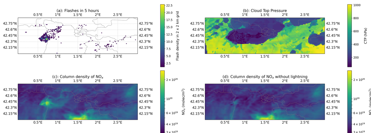
Figure 3. WRF-Chem simulation results for 6 July 2024 at 13:50 UTC, focused on the region of interest. (a) Assimilated lightning flashes between 08:50 and 13:50 UTC reported by Meteosat 12 LI. (b) Cloud Top Pressure (CTP). (c) Vertical Column Density of \text{NO}_x . (d) Vertical column density of \text{NO}_x in the simulation without fresh \text{LNO}_x , i.e., with \text{LNO}_x deactivated after 07:00 UTC. Meteosat 12 LI lightning data © EUMETSAT.
