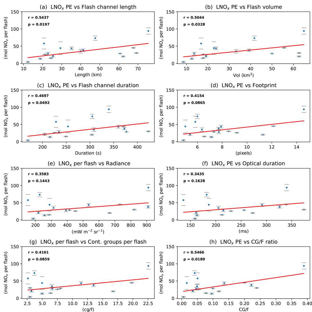
Figure 8. Pearson correlation between the \text{LNO}_x PE and the most important lightning characteristics included in this study. The average \text{LNO}_x PE (blue points) is obtained as the average between the \text{LNO}_x PE estimates by using both Meteosat 12 LI and the LMA for each analyzed case, while each pair of grey bars are the values of the \text{LNO}_x PE estimates by using Meteosat 12 LI and the LMA separately. The flash channel length, the flash volume and the flash durations in panels (a), (b) and (c) are the average values calculated from LMA measurements. The footprint, the radiance, the flash durations and the total number of contiguous groups per flash in panels (d), (e), (f) and (g) are the average values calculated from Meteosat 12 LI measurements. The average ratio of CG to total flashes in panel (h) is obtained from LLS-SMC and LMA lightning measurements. Each subplot includes the Pearson correlation coefficient r and its corresponding p -value, as well as a linear fitting of the blue points (red line). These results are based on calculations with \tau = 5 h.
