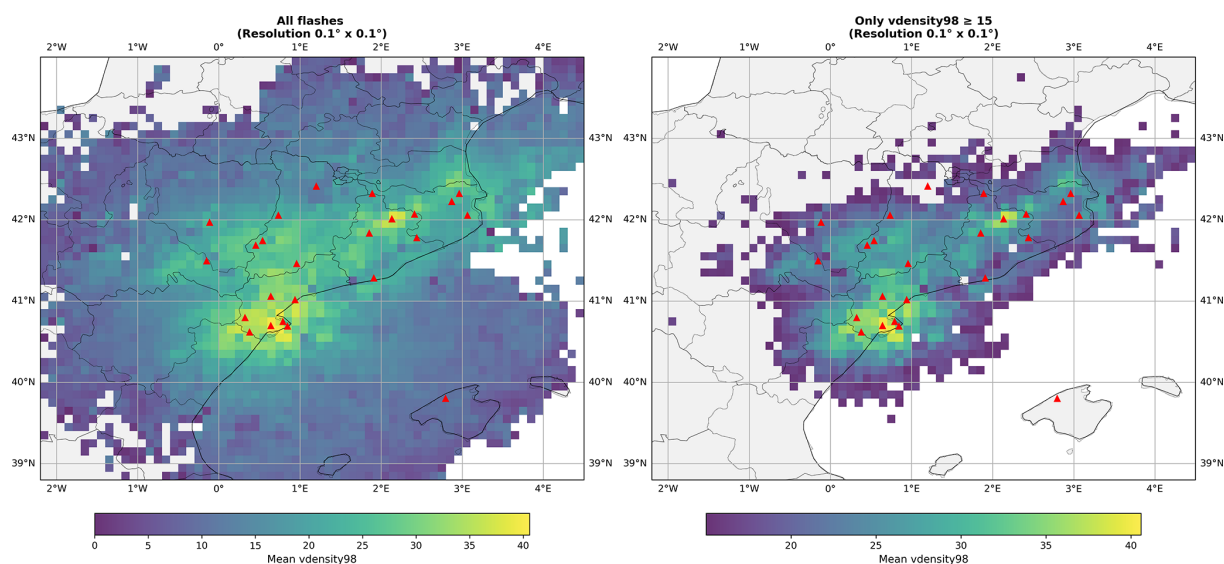
Figure 2. Left panel: 98th percentile vertical density score (vdensity98) averaged over all the flashes analyzed in this study and contained in each 0.1^\circ \times 0.1^\circ . Right panel: Masked data showing only pixels with \text{vdensity98} \geq 15 , showing the region with the best quality XCALMA data. Locations of the XCALMA sensors are included (red triangles).
