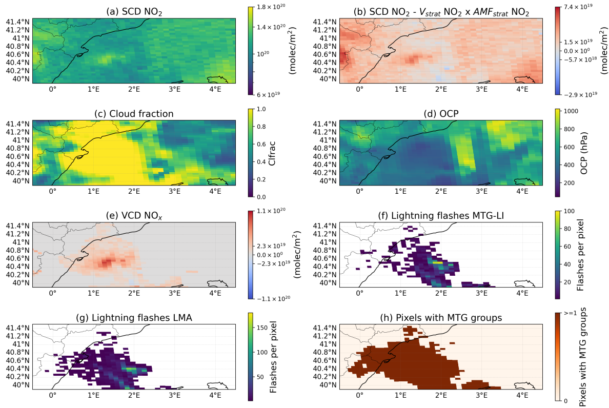
Figure S36. TROP-DLR product of orbit 36549, Meteoros 12 LI and LMA lightning data for the case 1 November 2024. (a): Slant Column Density (SCD) of \text{NO}_2 provided by the TROP-DLR \text{NO}_2 research product. (b): SCD \text{NO}_2 minus the stratospheric vertical column density and divided to the stratospheric air mass factor of \text{NO}_2 obtained from the TROP-DLR \text{NO}_2 research product. (c) and (d): Cloud Fraction (CF) and Optical Centroid Pressure (OCP) from the TROP-DLR \text{NO}_2 research product, respectively. (e): VCD of \text{NO}_x ( V_{\text{tropNO}_x} ) over pixels satisfying the DCC. (f) and (g): Lightning flashes during the 5 h period per TROPOMI pixel before the TROPOMI overpass reported by Meteoros 12 LI and the LMA, respectively. (h): TROPOMI pixels containing at least one lightning group detected by Meteoros 12 LI.
