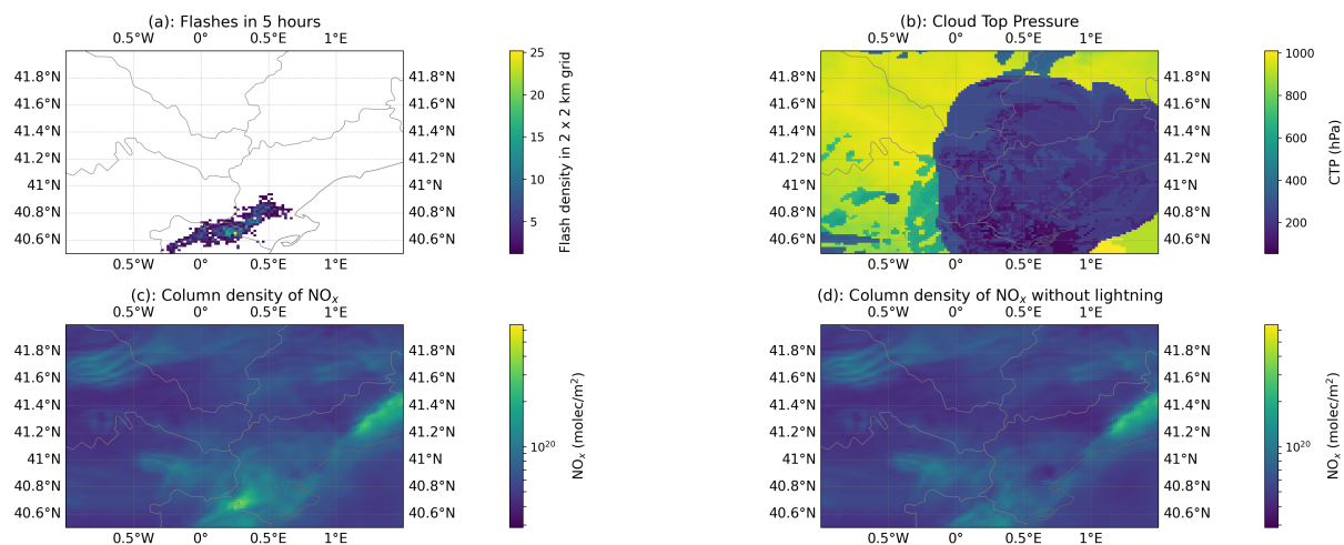
Figure S49. Simulation results for 4 May 2025 at 12:50 UTC, focused on the region of interest. (a): Assimilated lightning flashes between 07:50 and 12:50 UTC reported by Meteosat 12 LI. (b): Cloud Top Pressure (CTP). (c): Vertical Column Density of \text{NO}_x . (d): Vertical column density of \text{NO}_x in the simulation without fresh \text{LNO}_x , i.e., with \text{LNO}_x deactivated after 07:00 UTC.
