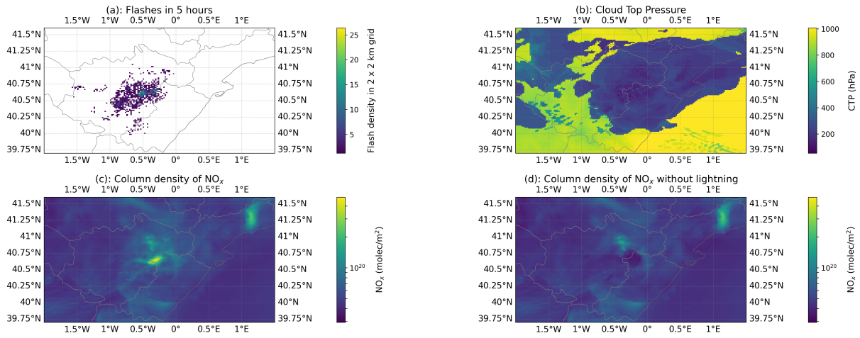
Figure S4. Simulation results for 2 August 2024 at 13:50 UTC, focused on the region of interest. (a): Assimilated lightning flashes between 08:50 and 13:50 UTC reported by Meteosat 12 LI. (b): Cloud Top Pressure (CTP). (c): Vertical Column Density of \text{NO}_x . (d): Vertical column density of \text{NO}_x in the simulation without fresh \text{LNO}_x , i.e., with \text{LNO}_x deactivated after 07:00 UTC.
