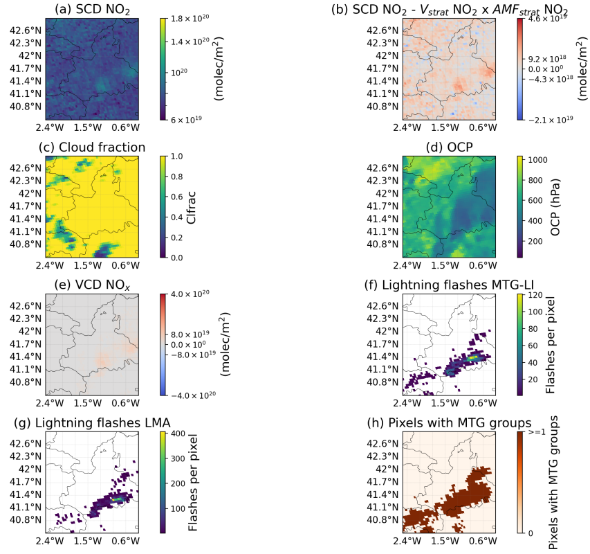
Figure S27. TROP-DLR product of orbit 35967, Meteosat 12 LI and LMA lightning data for the case 21 September 2024. (a): Slant Column Density (SCD) of \text{NO}_2 provided by the TROP-DLR \text{NO}_2 research product. (b): SCD \text{NO}_2 minus the stratospheric vertical column density and divided to the stratospheric air mass factor of \text{NO}_2 obtained from the TROP-DLR \text{NO}_2 research product. (c) and (d): Cloud Fraction (CF) and Optical Centroid Pressure (OCP) from the TROP-DLR \text{NO}_2 research product, respectively. (e): VCD of \text{NO}_x ( V_{trop\text{NO}_x} ) over pixels satisfying the DCC. (f) and (g): Lightning flashes during the 5 h period per TROPOMI pixel before the TROPOMI overpass reported by Meteosat 12 LI and the LMA, respectively. (h): TROPOMI pixels containing at least one lightning group detected by Meteosat 12 LI.
