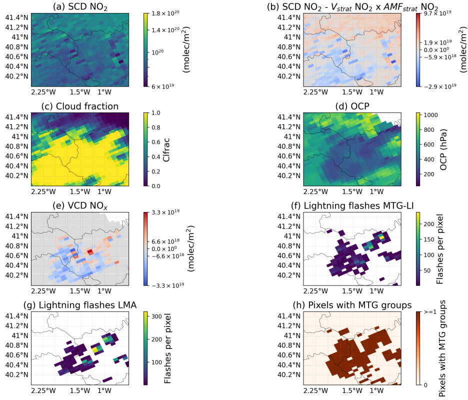
Figure S21. TROP-DLR product of orbit 35697, Meteosat 12 LI and LMA lightning data for the case 2 September 2024. (a): Slant Column Density (SCD) of \text{NO}_2 provided by the TROP-DLR \text{NO}_2 research product. (b): SCD \text{NO}_2 minus the stratospheric vertical column density and divided to the stratospheric air mass factor of \text{NO}_2 obtained from the TROP-DLR \text{NO}_2 research product. (c) and (d): Cloud Fraction (CF) and Optical Centroid Pressure (OCP) from the TROP-DLR \text{NO}_2 research product, respectively. (e): VCD of \text{NO}_x ( V_{trop\text{NO}_x} ) over pixels satisfying the DCC. (f) and (g): Lightning flashes during the 5 h period per TROPOMI pixel before the TROPOMI overpass reported by Meteosat 12 LI and the LMA, respectively. (h): TROPOMI pixels containing at least one lightning group detected by Meteosat 12 LI.
