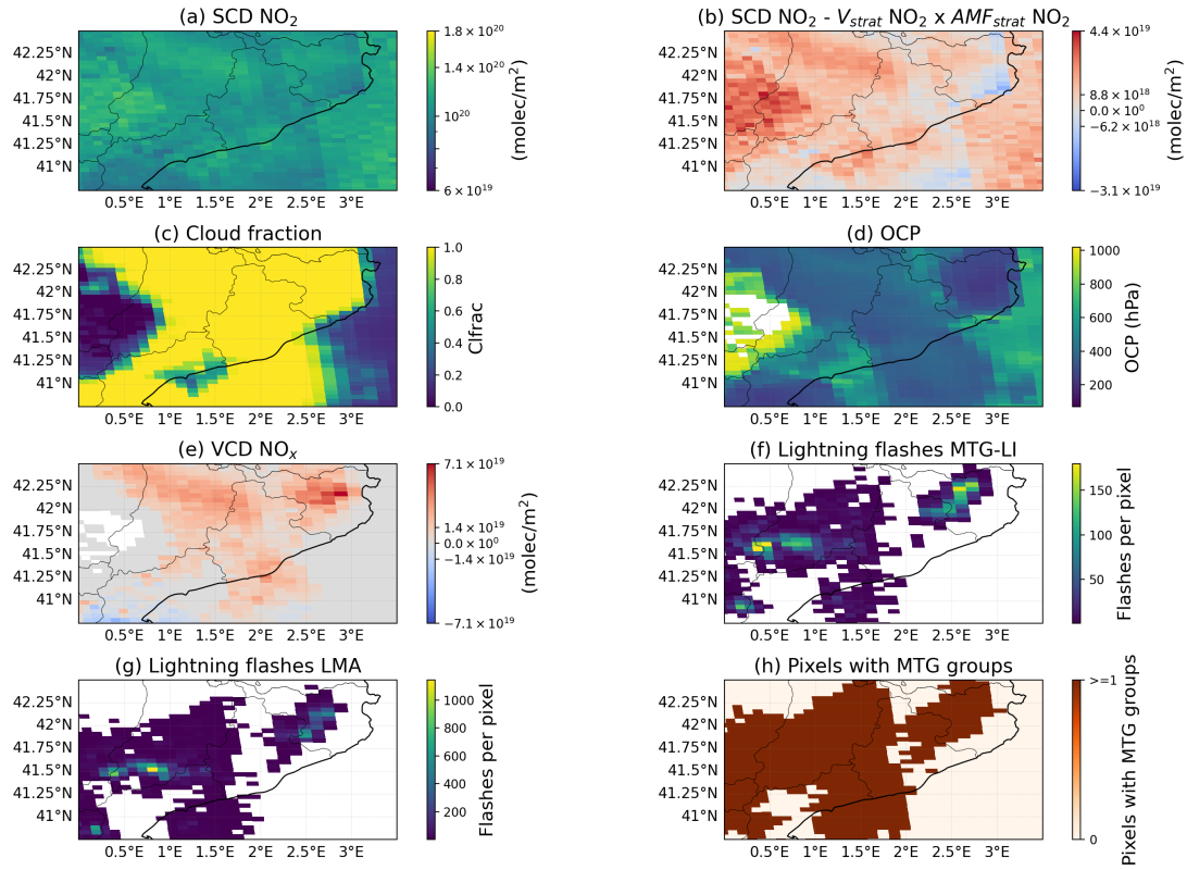
Figure S9. TROP-DLR product of orbit 35414, Meteosat 12 LI and LMA lightning data for the case 13 August 2024. (a): Slant Column Density (SCD) of NO 2 provided by the TROP-DLR NO 2 research product. (b): SCD NO 2 minus the stratospheric vertical column density and divided to the stratospheric air mass factor of NO 2 obtained from the TROP-DLR NO 2 research product. (c) and (d): Cloud Fraction (CF) and Optical Centroid Pressure (OCP) from the TROP-DLR NO 2 research product, respectively. (e): VCD of NO x ( V_{tropNO_x} ) over pixels satisfying the DCC. (f) and (g): Lightning flashes during the 5 h period per TROPOMI pixel before the TROPOMI overpass reported by Meteosat 12 LI and the LMA, respectively. (h): TROPOMI pixels containing at least one lightning group detected by Meteosat 12 LI.
