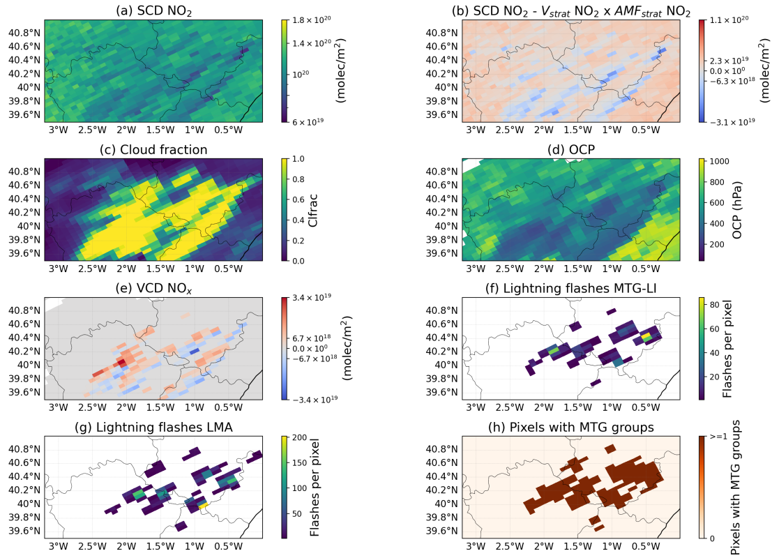
Figure S15. TROP-DLR product of orbit 35555, Meteosat 12 LI and LMA lightning data for the case 23 August 2024. (a): Slant Column Density (SCD) of \text{NO}_2 provided by the TROP-DLR \text{NO}_2 research product. (b): SCD \text{NO}_2 minus the stratospheric vertical column density and divided to the stratospheric air mass factor of \text{NO}_2 obtained from the TROP-DLR \text{NO}_2 research product. (c) and (d): Cloud Fraction (CF) and Optical Centroid Pressure (OCP) from the TROP-DLR \text{NO}_2 research product, respectively. (e): VCD of \text{NO}_x ( V_{\text{tropNO}_x} ) over pixels satisfying the DCC. (f) and (g): Lightning flashes during the 5 h period per TROPOMI pixel before the TROPOMI overpass reported by Meteosat 12 LI and the LMA, respectively. (h): TROPOMI pixels containing at least one lightning group detected by Meteosat 12 LI.
