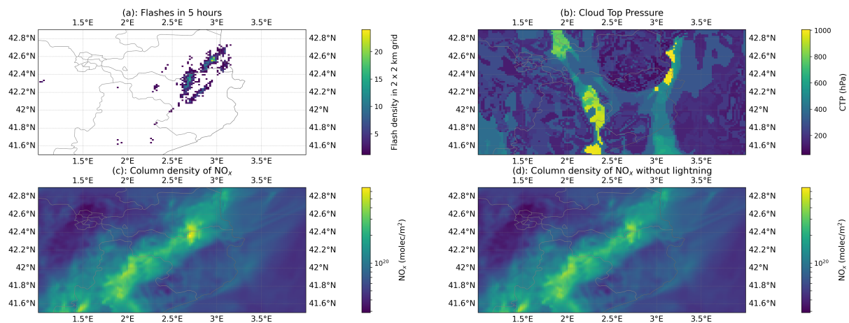
Figure S40. Simulation results for 15 April 2025 at 13:50 UTC, focused on the region of interest. (a): Assimilated lightning flashes between 08:50 and 13:50 UTC reported by Meteosat 12 LI. (b): Cloud Top Pressure (CTP). (c): Vertical Column Density of \text{NO}_x . (d): Vertical column density of \text{NO}_x in the simulation without fresh \text{LNO}_x , i.e., with \text{LNO}_x deactivated after 07:00 UTC.
