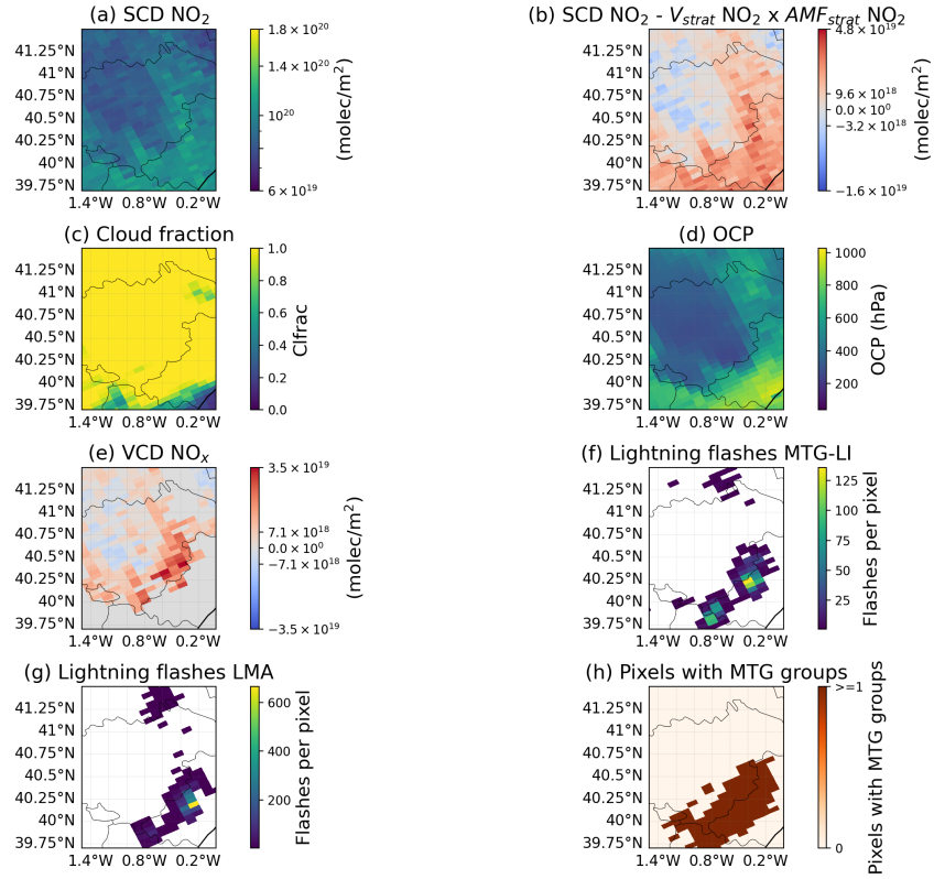
Figure S30. TROP-DLR product of orbit 36307, Meteosat 12 LI and LMA lightning data for the case 15 October 2024. (a): Slant Column Density (SCD) of \text{NO}_2 provided by the TROP-DLR \text{NO}_2 research product. (b): SCD \text{NO}_2 minus the stratospheric vertical column density and divided to the stratospheric air mass factor of \text{NO}_2 obtained from the TROP-DLR \text{NO}_2 research product. (c) and (d): Cloud Fraction (CF) and Optical Centroid Pressure (OCP) from the TROP-DLR \text{NO}_2 research product, respectively. (e): VCD of \text{NO}_x ( V_{trop\text{NO}_x} ) over pixels satisfying the DCC. (f) and (g): Lightning flashes during the 5 h period per TROPOMI pixel before the TROPOMI overpass reported by Meteosat 12 LI and the LMA, respectively. (h): TROPOMI pixels containing at least one lightning group detected by Meteosat 12 LI.
