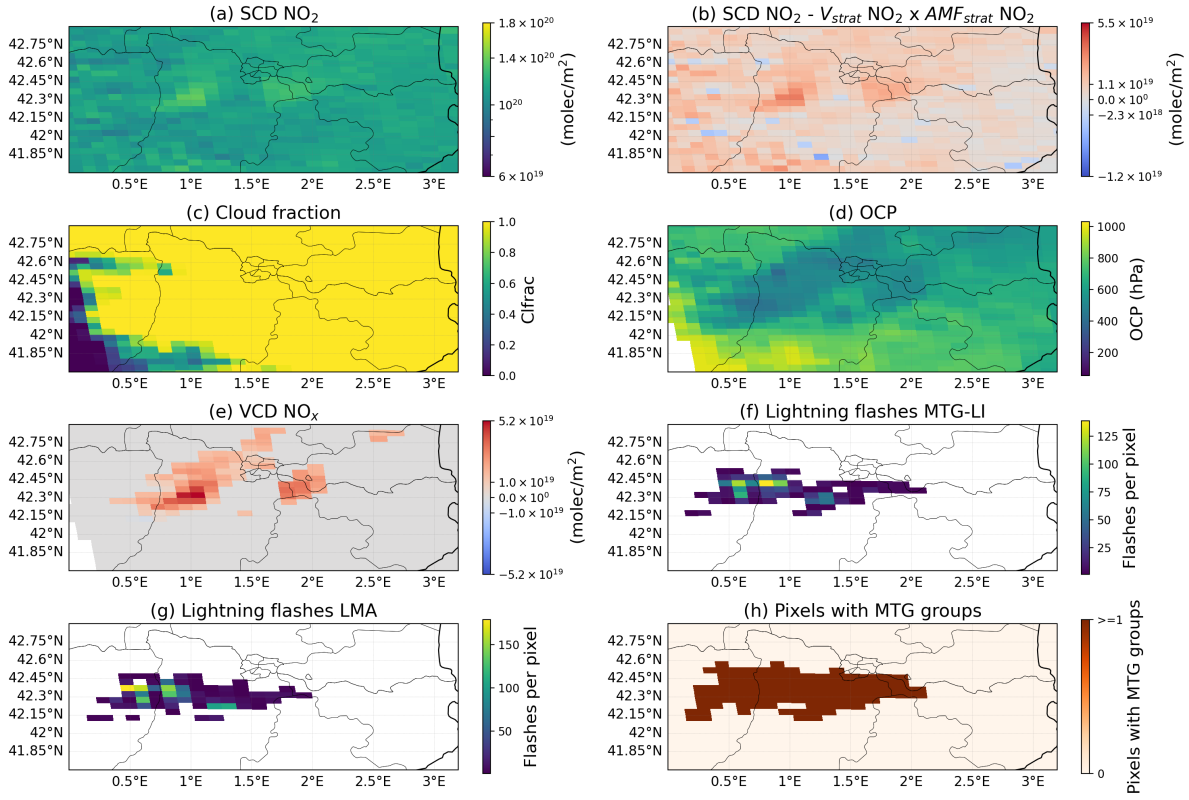
Figure S48. TROP-DLR product of orbit 39046, Meteosat 12 LI and LMA lightning data for the case 26 April 2025. (a): Slant Column Density (SCD) of \text{NO}_2 provided by the TROP-DLR \text{NO}_2 research product. (b): SCD \text{NO}_2 minus the stratospheric vertical column density and divided to the stratospheric air mass factor of \text{NO}_2 obtained from the TROP-DLR \text{NO}_2 research product. (c) and (d): Cloud Fraction (CF) and Optical Centroid Pressure (OCP) from the TROP-DLR \text{NO}_2 research product, respectively. (e): VCD of \text{NO}_x ( V_{\text{tropNO}_x} ) over pixels satisfying the DCC. (f) and (g): Lightning flashes during the 5 h period per TROPOMI pixel before the TROPOMI overpass reported by Meteosat 12 LI and the LMA, respectively. (h): TROPOMI pixels containing at least one lightning group detected by Meteosat 12 LI.
