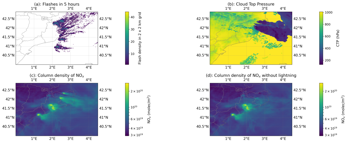
Figure S1. Simulation results for 21 July 2024 at 12:30 UTC, focused on the region of interest. (a): Assimilated lightning flashes between 07:30 and 12:30 UTC reported by Meteosat 12 LI. (b): Cloud Top Pressure (CTP). (c): Vertical Column Density of NO x . (d): Vertical column density of NO x in the simulation without fresh LNO x , i.e., with LNO x deactivated after 07:00 UTC.
