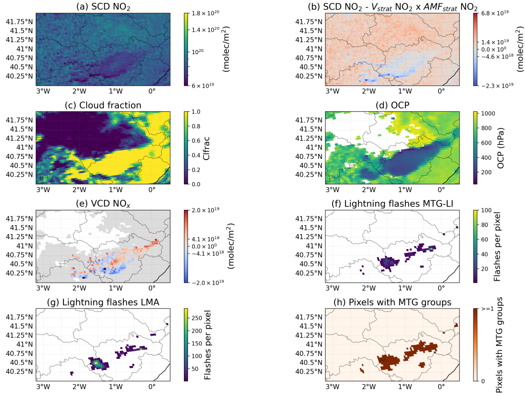
Figure S18. TROP-DLR product of orbit 35584, Meteosat 12 LI and LMA lightning data for the case 25 August 2024. (a): Slant Column Density (SCD) of \text{NO}_2 provided by the TROP-DLR \text{NO}_2 research product. (b): SCD \text{NO}_2 minus the stratospheric vertical column density and divided to the stratospheric air mass factor of \text{NO}_2 obtained from the TROP-DLR \text{NO}_2 research product. (c) and (d): Cloud Fraction (CF) and Optical Centroid Pressure (OCP) from the TROP-DLR \text{NO}_2 research product, respectively. (e): VCD of \text{NO}_x ( V_{\text{tropNO}_x} ) over pixels satisfying the DCC. (f) and (g): Lightning flashes during the 5 h period per TROPOMI pixel before the TROPOMI overpass reported by Meteosat 12 LI and the LMA, respectively. (h): TROPOMI pixels containing at least one lightning group detected by Meteosat 12 LI.
