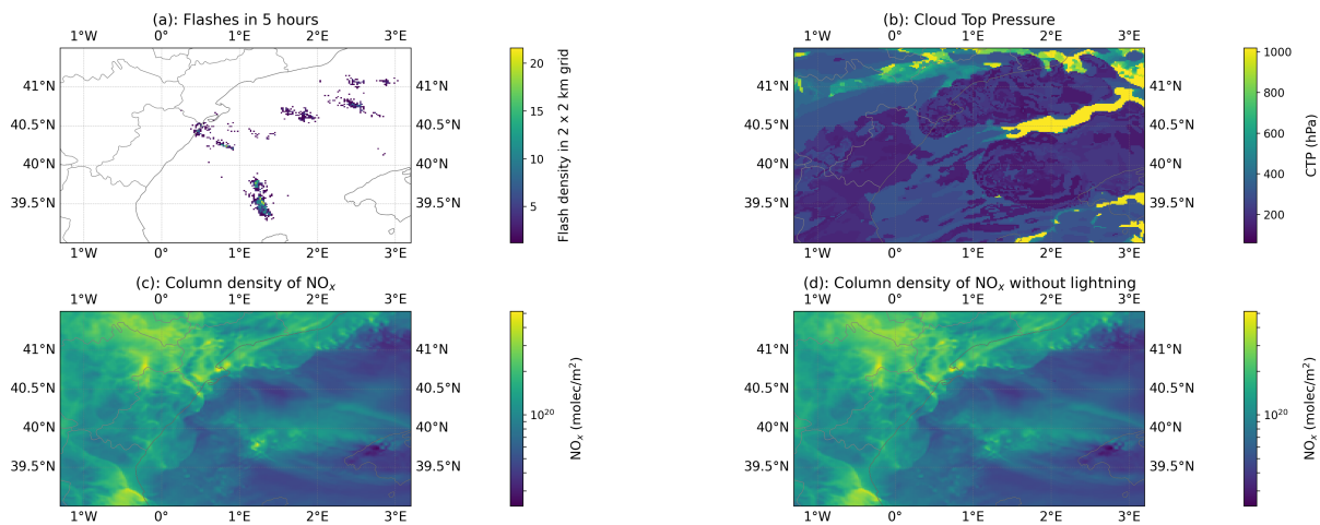
Figure S37. Simulation results for 13 November 2024 at 13:10 UTC, focused on the region of interest. (a): Assimilated lightning flashes between 08:10 and 13:10 UTC reported by Meteosat 12 LI. (b): Cloud Top Pressure (CTP). (c): Vertical Column Density of \text{NO}_x . (d): Vertical column density of \text{NO}_x in the simulation without fresh \text{LNO}_x , i.e., with \text{LNO}_x deactivated after 07:00 UTC.
