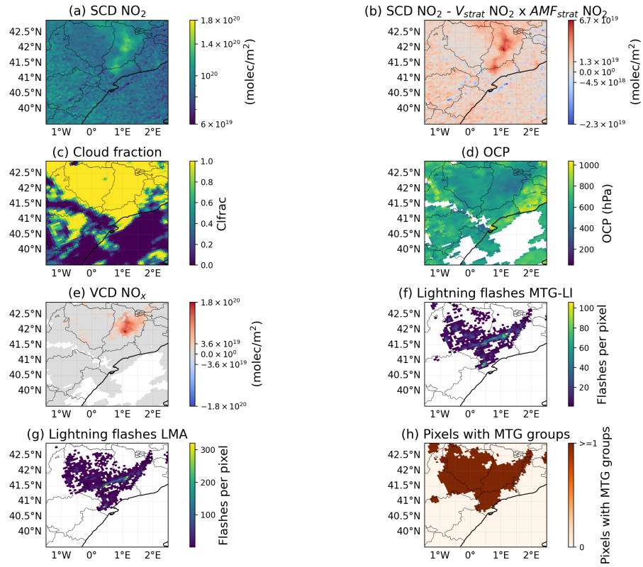
Figure S45. TROP-DLR product of orbit 38946, Meteosat 12 LI and LMA lightning data for the case 19 April 2025. (a): Slant Column Density (SCD) of \text{NO}_2 provided by the TROP-DLR \text{NO}_2 research product. (b): SCD \text{NO}_2 minus the stratospheric vertical column density and divided to the stratospheric air mass factor of \text{NO}_2 obtained from the TROP-DLR \text{NO}_2 research product. (c) and (d): Cloud Fraction (CF) and Optical Centroid Pressure (OCP) from the TROP-DLR \text{NO}_2 research product, respectively. (e): VCD of \text{NO}_x ( V_{\text{tropNO}_x} ) over pixels satisfying the DCC. (f) and (g): Lightning flashes during the 5 h period per TROPOMI pixel before the TROPOMI overpass reported by Meteosat 12 LI and the LMA, respectively. (h): TROPOMI pixels containing at least one lightning group detected by Meteosat 12 LI.
