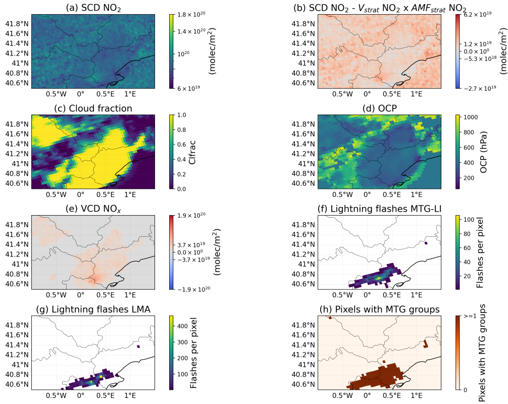
Figure S51. TROP-DLR product of orbit 39159, Meteosat 12 LI and LMA lightning data for the case 4 May 2025. (a): Slant Column Density (SCD) of NO 2 provided by the TROP-DLR NO 2 research product. (b): SCD NO 2 minus the stratospheric vertical column density and divided to the stratospheric air mass factor of NO 2 obtained from the TROP-DLR NO 2 research product. (c) and (d): Cloud Fraction (CF) and Optical Centroid Pressure (OCP) from the TROP-DLR NO 2 research product, respectively. (e): VCD of NO x ( V_{tropNOx} ) over pixels satisfying the DCC. (f) and (g): Lightning flashes during the 5 h period per TROPOMI pixel before the TROPOMI overpass reported by Meteosat 12 LI and the LMA, respectively. (h): TROPOMI pixels containing at least one lightning group detected by Meteosat 12 LI.
