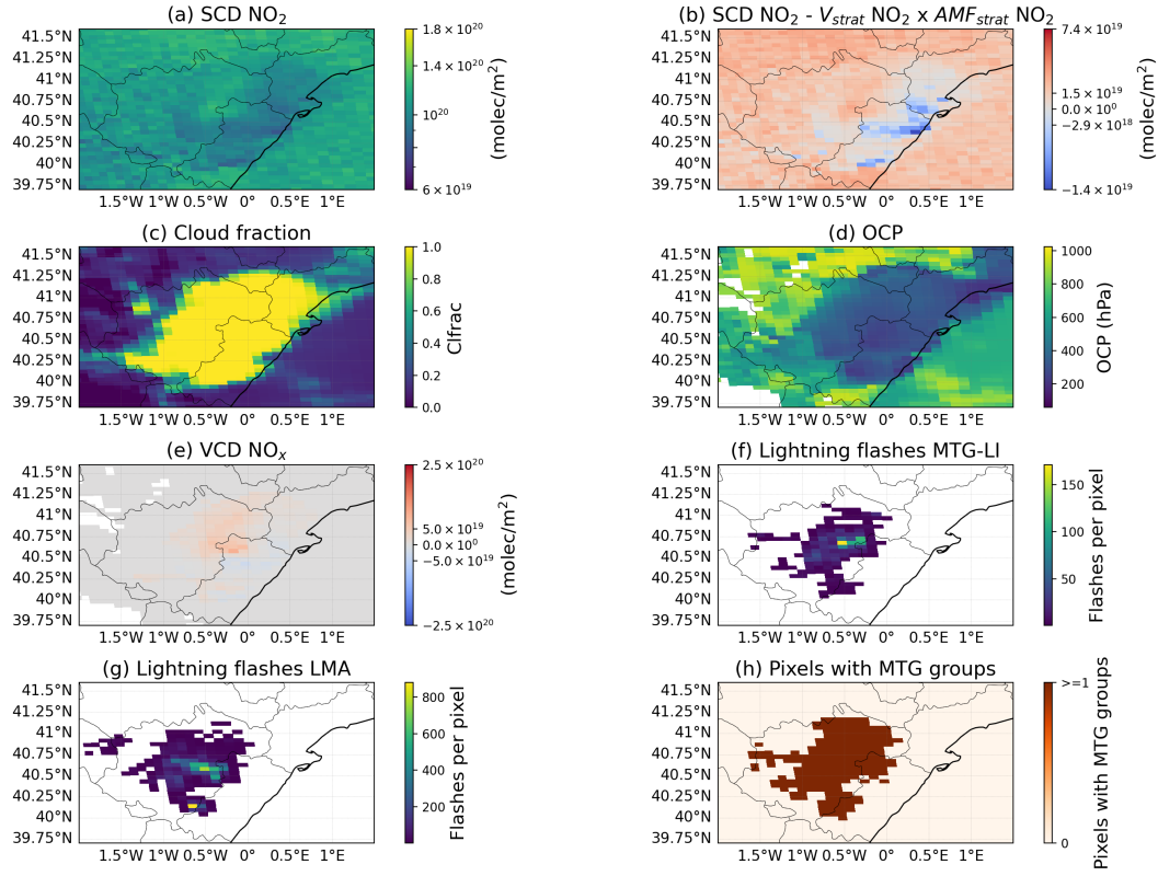
Figure S6. TROP-DLR product of orbit 35258, Meteosat 12 LI and LMA lightning data for the case 2 August 2024. (a): Slant Column Density (SCD) of \text{NO}_2 provided by the TROP-DLR \text{NO}_2 research product. (b): SCD \text{NO}_2 minus the stratospheric vertical column density and divided to the stratospheric air mass factor of \text{NO}_2 obtained from the TROP-DLR \text{NO}_2 research product. (c) and (d): Cloud Fraction (CF) and Optical Centroid Pressure (OCP) from the TROP-DLR \text{NO}_2 research product, respectively. (e): VCD of \text{NO}_x ( V_{\text{tropNO}_x} ) over pixels satisfying the DCC. (f) and (g): Lightning flashes during the 5 h period per TROPOMI pixel before the TROPOMI overpass reported by Meteosat 12 LI and the LMA, respectively. (h): TROPOMI pixels containing at least one lightning group detected by Meteosat 12 LI.
