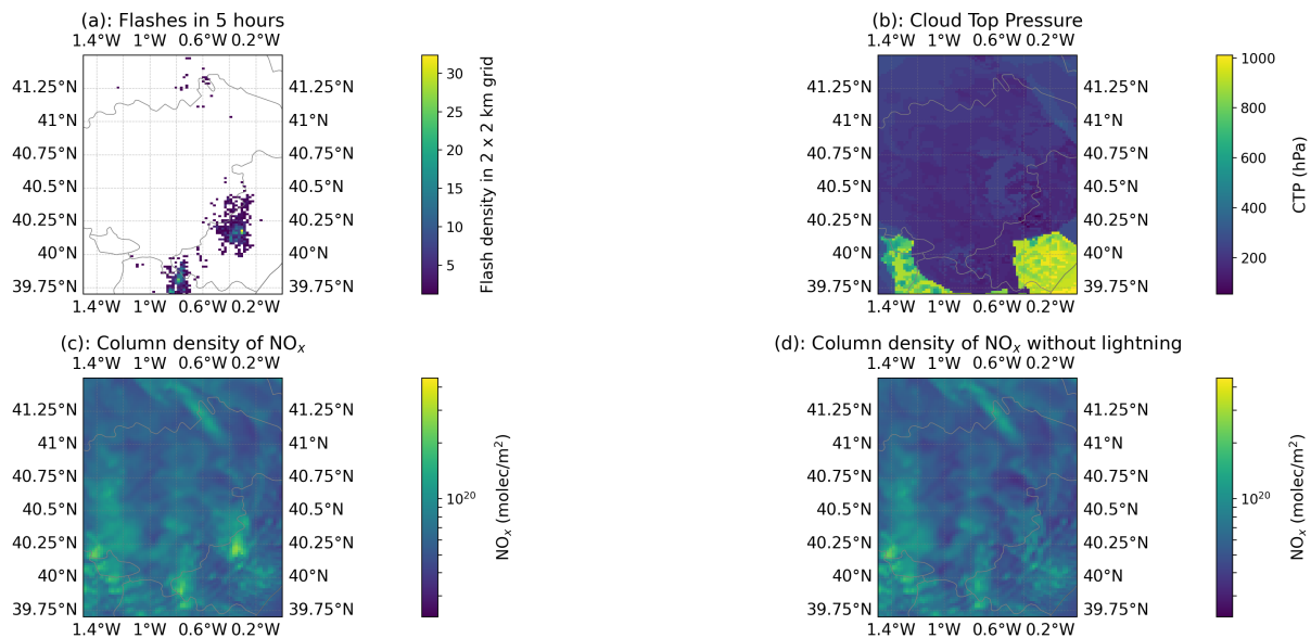
Figure S28. Simulation results for 15 October 2024 at 12:10 UTC, focused on the region of interest. (a): Assimilated lightning flashes between 07:10 and 12:10 UTC reported by Meteosat 12 LI. (b): Cloud Top Pressure (CTP). (c): Vertical Column Density of \text{NO}_x . (d): Vertical column density of \text{NO}_x in the simulation without fresh \text{LNO}_x , i.e., with \text{LNO}_x deactivated after 07:00 UTC.
