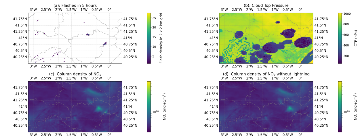
Figure S16. Simulation results for 25 August 2024 at 13:10 UTC, focused on the region of interest. (a): Assimilated lightning flashes between 08:10 and 13:10 UTC reported by Meteosat 12 LI. (b): Cloud Top Pressure (CTP). (c): Vertical Column Density of \text{NO}_x . (d): Vertical column density of \text{NO}_x in the simulation without fresh \text{LNO}_x , i.e., with \text{LNO}_x deactivated after 07:00 UTC.
