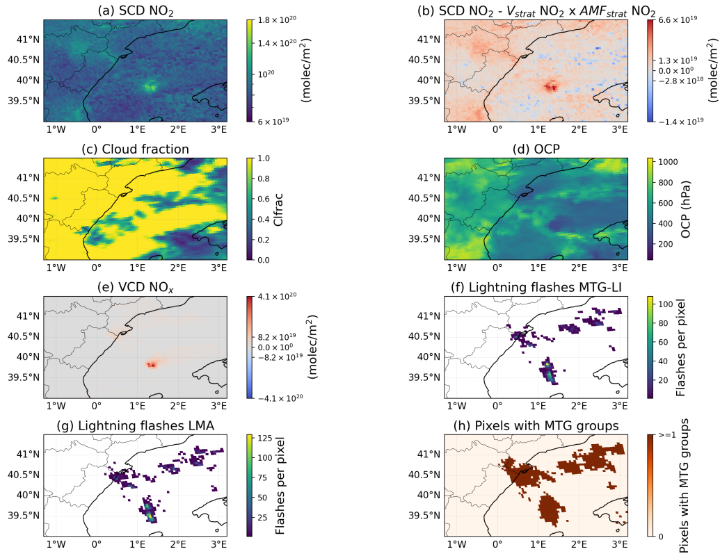
Figure S39. TROP-DLR product of orbit 36719, Meteosat 12 LI and LMA lightning data for the case 13 November 2024. (a): Slant Column Density (SCD) of \text{NO}_2 provided by the TROP-DLR \text{NO}_2 research product. (b): SCD \text{NO}_2 minus the stratospheric vertical column density and divided to the stratospheric air mass factor of \text{NO}_2 obtained from the TROP-DLR \text{NO}_2 research product. (c) and (d): Cloud Fraction (CF) and Optical Centroid Pressure (OCP) from the TROP-DLR \text{NO}_2 research product, respectively. (e): VCD of \text{NO}_x ( V_{trop\text{NO}_x} ) over pixels satisfying the DCC. (f) and (g): Lightning flashes during the 5 h period per TROPOMI pixel before the TROPOMI overpass reported by Meteosat 12 LI and the LMA, respectively. (h): TROPOMI pixels containing at least one lightning group detected by Meteosat 12 LI.
