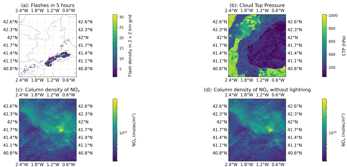
Figure S25. Simulation results for 21 September 2024 at 13:10 UTC, focused on the region of interest. (a): Assimilated lightning flashes between 08:10 and 13:10 UTC reported by Meteosat 12 LI. (b): Cloud Top Pressure (CTP). (c): Vertical Column Density of \text{NO}_x . (d): Vertical column density of \text{NO}_x in the simulation without fresh \text{LNO}_x , i.e., with \text{LNO}_x deactivated after 07:00 UTC.
