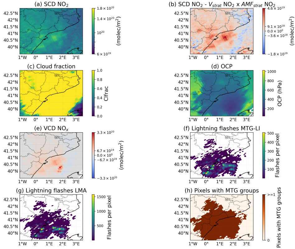
Figure S24. TROP-DLR product of orbit 35711, Meteosat 12 LI and LMA lightning data for the case 3 September 2024. (a): Slant Column Density (SCD) of \text{NO}_2 provided by the TROP-DLR \text{NO}_2 research product. (b): SCD \text{NO}_2 minus the stratospheric vertical column density and divided to the stratospheric air mass factor of \text{NO}_2 obtained from the TROP-DLR \text{NO}_2 research product. (c) and (d): Cloud Fraction (CF) and Optical Centroid Pressure (OCP) from the TROP-DLR \text{NO}_2 research product, respectively. (e): VCD of \text{NO}_x ( V_{trop\text{NO}_x} ) over pixels satisfying the DCC. (f) and (g): Lightning flashes during the 5 h period per TROPOMI pixel before the TROPOMI overpass reported by Meteosat 12 LI and the LMA, respectively. (h): TROPOMI pixels containing at least one lightning group detected by Meteosat 12 LI.
