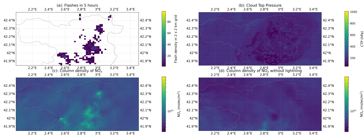
Figure S10. Simulation results for 14 August 2024 at 13:20 UTC, focused on the region of interest. (a): Assimilated lightning flashes between 08:20 and 13:20 UTC reported by Meteosat 12 LI. (b): Cloud Top Pressure (CTP). (c): Vertical Column Density of \text{NO}_x . (d): Vertical column density of \text{NO}_x in the simulation without fresh \text{LNO}_x , i.e., with \text{LNO}_x deactivated after 07:00 UTC.
