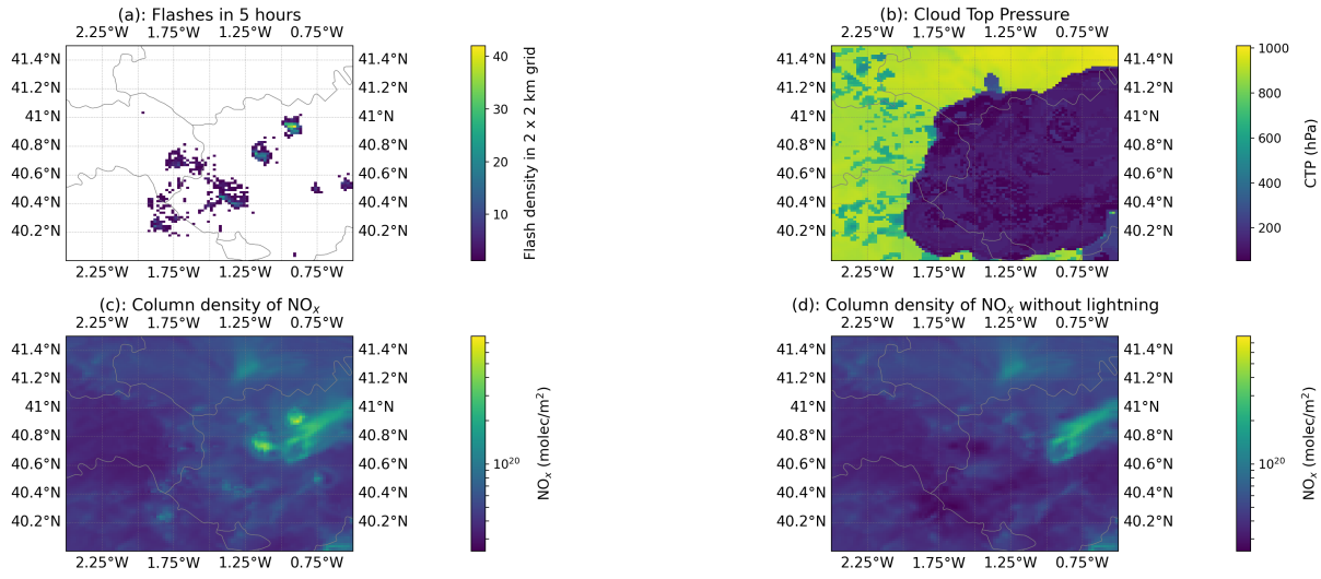
Figure S19. Simulation results for 2 September 2024 at 12:20 UTC, focused on the region of interest. (a): Assimilated lightning flashes between 07:20 and 12:20 UTC reported by Meteosat 12 LI. (b): Cloud Top Pressure (CTP). (c): Vertical Column Density of \text{NO}_x . (d): Vertical column density of \text{NO}_x in the simulation without fresh \text{LNO}_x , i.e., with \text{LNO}_x deactivated after 07:00 UTC.
