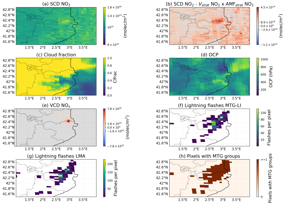
Figure S42. TROP-DLR product of orbit 38890, Meteosat 12 LI and LMA lightning data for the case 15 April 2025. (a): Slant Column Density (SCD) of NO 2 provided by the TROP-DLR NO 2 research product. (b): SCD NO 2 minus the stratospheric vertical column density and divided to the stratospheric air mass factor of NO 2 obtained from the TROP-DLR NO 2 research product. (c) and (d): Cloud Fraction (CF) and Optical Centroid Pressure (OCP) from the TROP-DLR NO 2 research product, respectively. (e): VCD of NO x ( V_{tropNOx} ) over pixels satisfying the DCC. (f) and (g): Lightning flashes during the 5 h period per TROPOMI pixel before the TROPOMI overpass reported by Meteosat 12 LI and the LMA, respectively. (h): TROPOMI pixels containing at least one lightning group detected by Meteosat 12 LI.
