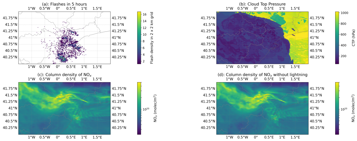
Figure S31. Simulation results for 31 October 2024 at 12:30 UTC, focused on the region of interest. (a): Assimilated lightning flashes between 07:30 and 12:30 UTC reported by Meteosat 12 LI. (b): Cloud Top Pressure (CTP). (c): Vertical Column Density of \text{NO}_x . (d): Vertical column density of \text{NO}_x in the simulation without fresh \text{LNO}_x , i.e., with \text{LNO}_x deactivated after 07:00 UTC.
