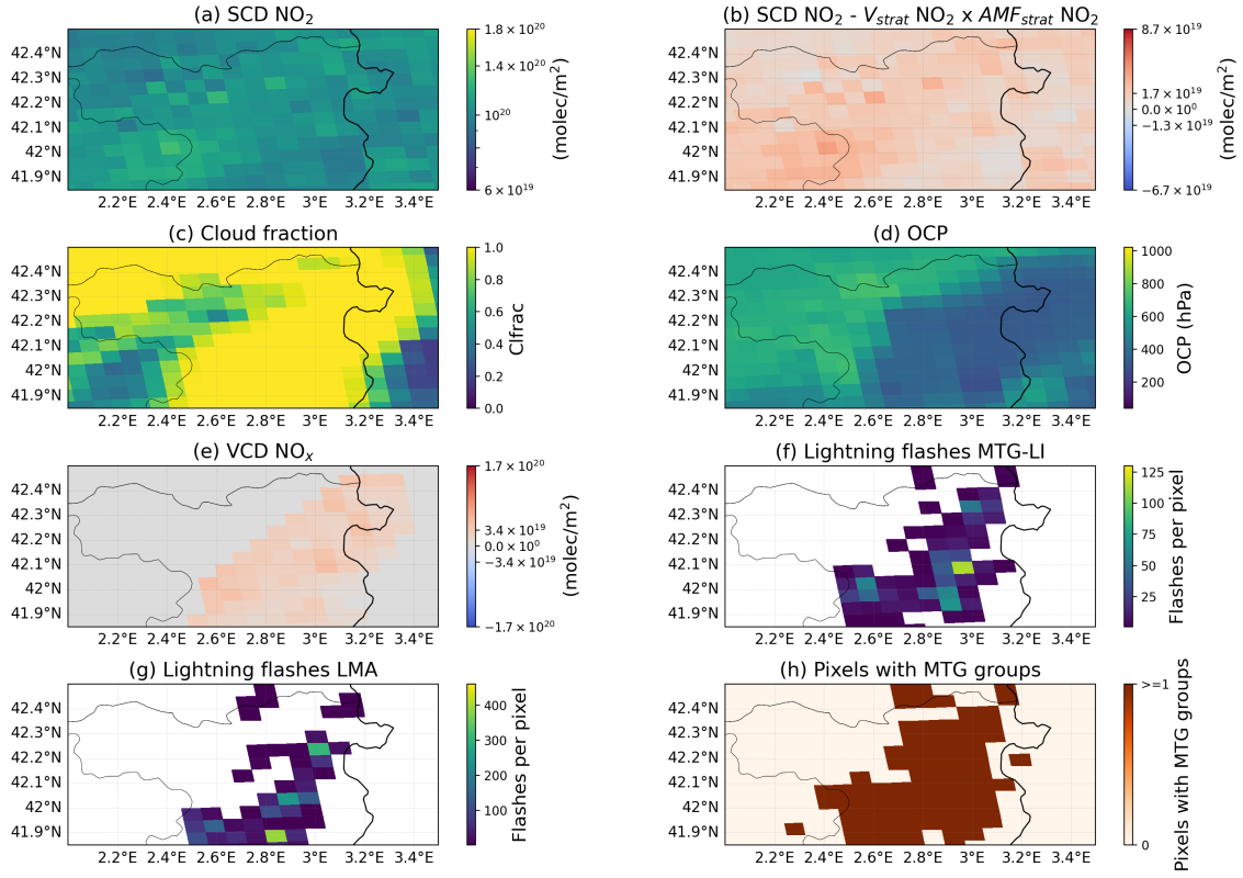
Figure S12. TROP-DLR product of orbit 35428, Meteosat 12 LI and LMA lightning data for the case 14 August 2024. (a): Slant Column Density (SCD) of \text{NO}_2 provided by the TROP-DLR \text{NO}_2 research product. (b): SCD \text{NO}_2 minus the stratospheric vertical column density and divided to the stratospheric air mass factor of \text{NO}_2 obtained from the TROP-DLR \text{NO}_2 research product. (c) and (d): Cloud Fraction (CF) and Optical Centroid Pressure (OCP) from the TROP-DLR \text{NO}_2 research product, respectively. (e): VCD of \text{NO}_x ( V_{\text{tropNO}_x} ) over pixels satisfying the DCC. (f) and (g): Lightning flashes during the 5 h period per TROPOMI pixel before the TROPOMI overpass reported by Meteosat 12 LI and the LMA, respectively. (h): TROPOMI pixels containing at least one lightning group detected by Meteosat 12 LI.
