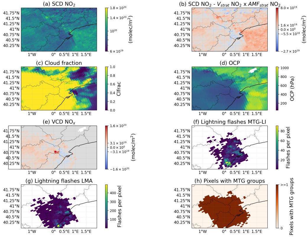
Figure S33. TROP-DLR product of orbit 36534, Meteosat 12 LI and LMA lightning data for the case 31 October 2024. (a): Slant Column Density (SCD) of \text{NO}_2 provided by the TROP-DLR \text{NO}_2 research product. (b): SCD \text{NO}_2 minus the stratospheric vertical column density and divided to the stratospheric air mass factor of \text{NO}_2 obtained from the TROP-DLR \text{NO}_2 research product. (c) and (d): Cloud Fraction (CF) and Optical Centroid Pressure (OCP) from the TROP-DLR \text{NO}_2 research product, respectively. (e): VCD of \text{NO}_x ( V_{\text{tropNO}_x} ) over pixels satisfying the DCC. (f) and (g): Lightning flashes during the 5 h period per TROPOMI pixel before the TROPOMI overpass reported by Meteosat 12 LI and the LMA, respectively. (h): TROPOMI pixels containing at least one lightning group detected by Meteosat 12 LI.
