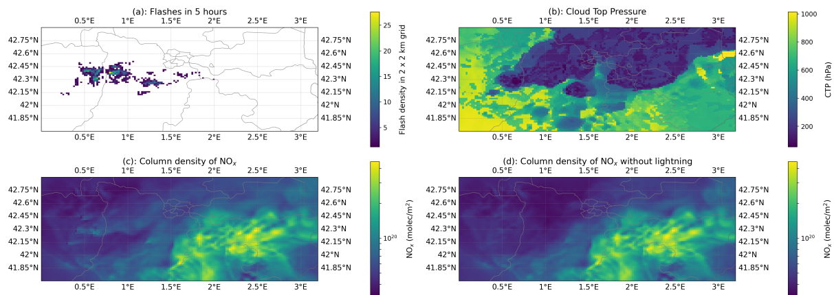
Figure S46. Simulation results for 26 April 2025 at 13:40 UTC, focused on the region of interest. (a): Assimilated lightning flashes between 08:40 and 13:40 UTC reported by Meteosat 12 LI. (b): Cloud Top Pressure (CTP). (c): Vertical Column Density of \text{NO}_x . (d): Vertical column density of \text{NO}_x in the simulation without fresh \text{LNO}_x , i.e., with \text{LNO}_x deactivated after 07:00 UTC.
