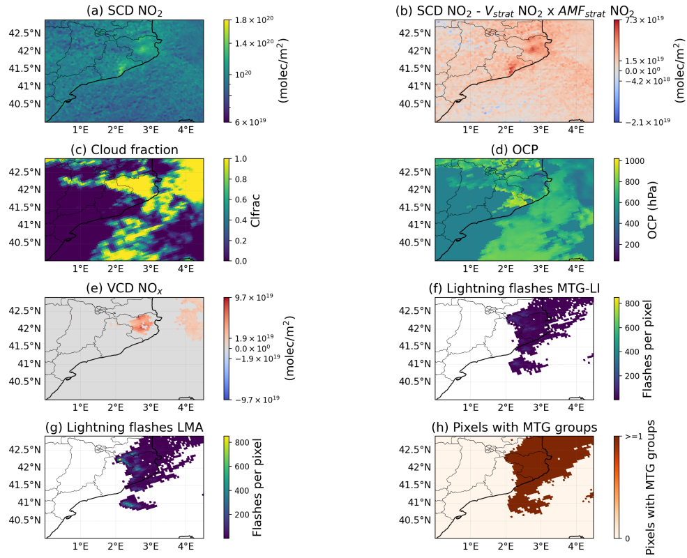
Figure S3. TROP-DLR product of orbit 35087, Meteosat 12 LI and LMA lightning data for the case 21 July 2024. (a): Slant Column Density (SCD) of NO 2 provided by the TROP-DLR NO 2 research product. (b): SCD NO 2 minus the stratospheric vertical column density and divided to the stratospheric air mass factor of NO 2 obtained from the TROP-DLR NO 2 research product. (c) and (d): Cloud Fraction (CF) and Optical Centroid Pressure (OCP) from the TROP-DLR NO 2 research product, respectively. (e): VCD of NO x ( V_{tropNOx} ) over pixels satisfying the DCC. (f) and (g): Lightning flashes during the 5 h period per TROPOMI pixel before the TROPOMI overpass reported by Meteosat 12 LI and the LMA, respectively. (h): TROPOMI pixels containing at least one lightning group detected by Meteosat 12 LI.
