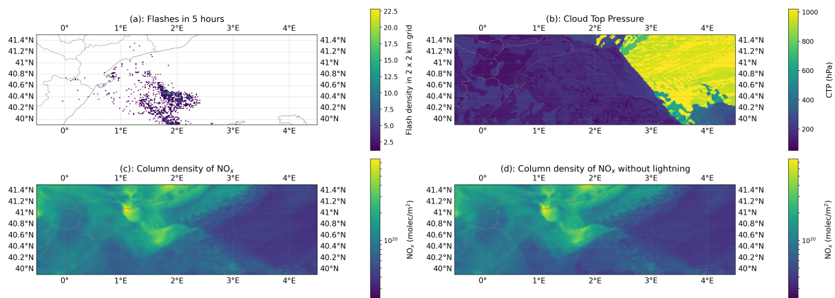
Figure S34. Simulation results for 1 November 2024 at 13:40 UTC, focused on the region of interest. (a): Assimilated lightning flashes between 08:40 and 13:40 UTC reported by Meteosat 12 LI. (b): Cloud Top Pressure (CTP). (c): Vertical Column Density of \text{NO}_x . (d): Vertical column density of \text{NO}_x in the simulation without fresh \text{LNO}_x , i.e., with \text{LNO}_x deactivated after 07:00 UTC.
