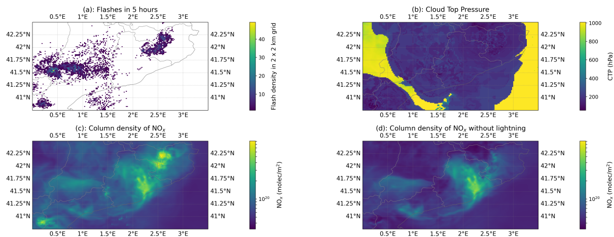
Figure S7. Simulation results for 13 August 2024 at 13:40 UTC, focused on the region of interest. (a): Assimilated lightning flashes between 08:40 and 13:40 UTC reported by Meteosat 12 LI. (b): Cloud Top Pressure (CTP). (c): Vertical Column Density of \text{NO}_x . (d): Vertical column density of \text{NO}_x in the simulation without fresh \text{LNO}_x , i.e., with \text{LNO}_x deactivated after 07:00 UTC.
