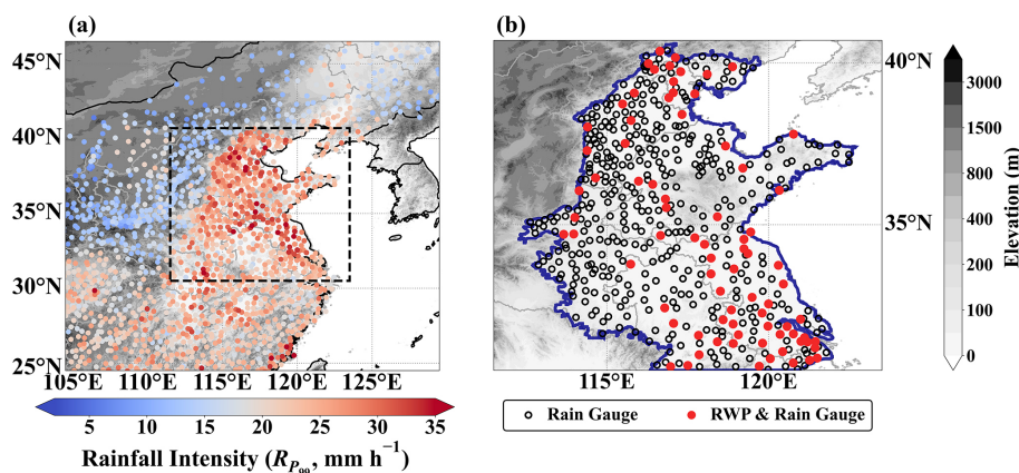
Figure 1. (a) Spatial distribution of 99th-percentile hourly rainfall intensity ( R_{P99} ; \text{mm h}^{-1} ) at rain gauges across eastern China during the warm seasons (June–September) of 2021–2025. Grayscale shading represents terrain elevation, and the dashed black rectangle marks the subdomain zoomed in panel (b). (b) Enlarged view of the study domain covering the eastern China plains. The dark blue contour denotes areas within 111.5\text{--}123.5^\circ\text{E} and 30.5\text{--}40.7^\circ\text{N} with terrain elevation at or below 200 m. Open black circles indicate standalone rain gauge sites, while red filled circles mark co-located radar wind profiler (RWP) and rain-gauge stations.
