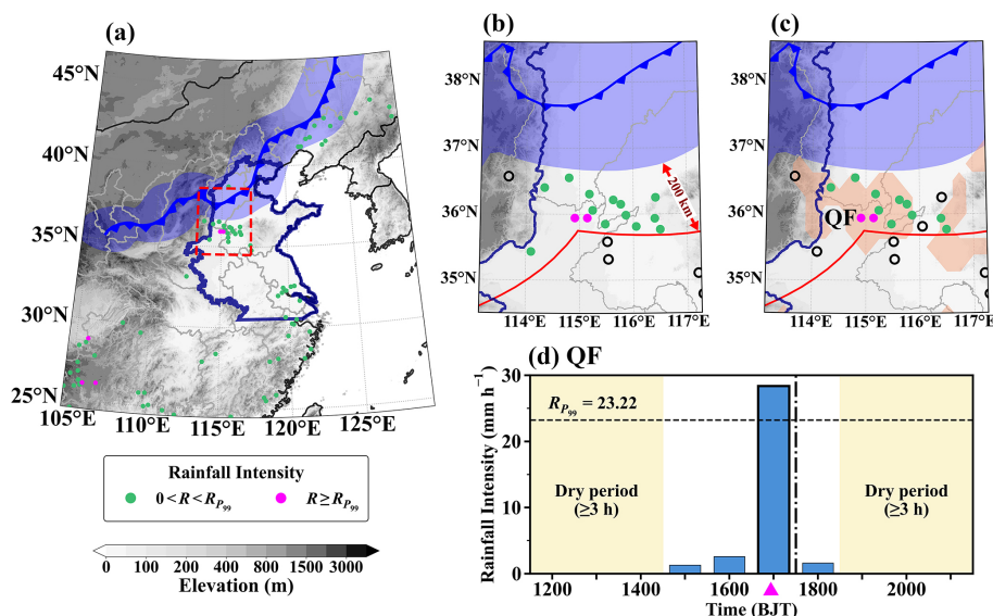
Figure 3. Example of an identified WSHR event at Qingfeng (QF) weather station on 18 August 2023. (a) Cold front (blue line) and its 200 km frontal zone (blue shading) at 17:00 BJT, with station rainfall overlaid (green dots: 0 < R < R_{p99} ; magenta dots: R \geq R_{p99} ). (b) and (c) Enlarged views of the red dashed rectangle in (a): (b) shows rainfall at stations 200–400 km from the front (the warm-sector candidate region); (c) additionally shows the warm-sector mask (orange shading) and rainfall at stations falling within it. Open black circles denote stations with rainfall ( R > 0 ) that fall outside the study region or fail the warm-sector criteria. (d) Hourly rainfall time series at QF station. The dashed line marks R_{p99} = 23.22 \text{ mm h}^{-1} ; the dash-dotted line marks the first hour reaching R_{p99} , with all rainfall hours from onset to this hour required to lie within the warm sector. Yellow shading denotes dry periods ( \geq 3 \text{ h} ) bounding the event, and the magenta triangle marks the hour identified as WSHR.
