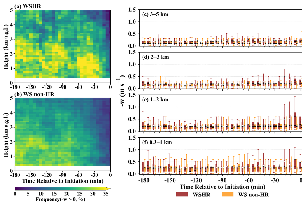
Figure 12. Composite ascending motion preceding the onset of WSHR events and WS non-HR events. (a, b) Frequency of ascending motion ( -w > 0 ; %) as a function of height (km a.g.l.) and time relative to the rainfall onset (min) for (a) WSHR events and (b) WS non-HR events. (c–f) Box plots of the across-event distributions of layer-maximum ascent speed ( -w ; \text{m s}^{-1} ) at each 6 min lead time for the WSHR (dark red) and WS non-HR (orange) events in the (c) 3–5 km, (d) 2–3 km, (e) 1–2 km, and (f) 0.3–1 km a.g.l. layers.
