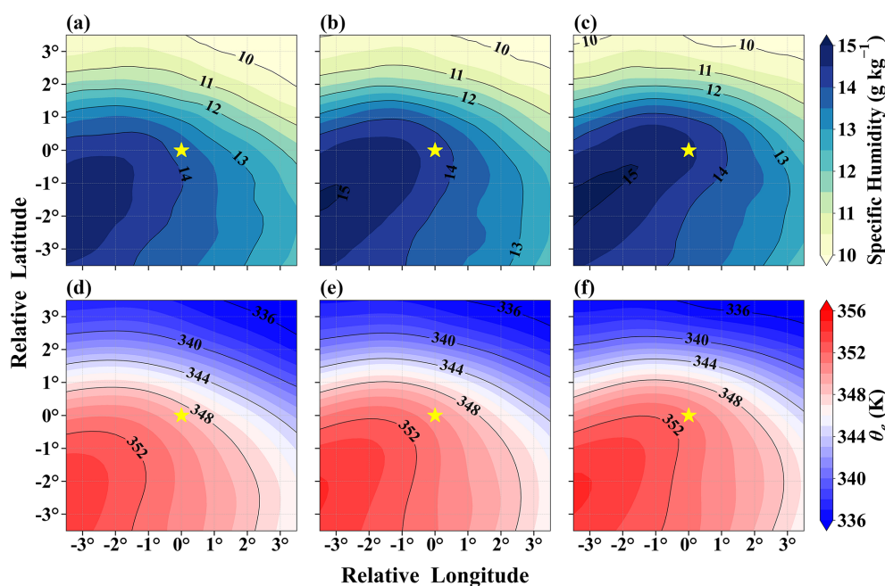
Figure 7. Composite 850 hPa specific humidity ( a–c ; shading, g\ kg^{-1} ; contours every 1\ g\ kg^{-1} ) and pseudo-equivalent potential temperature \theta_e ( d–f ; shading, K; contours every 4 K) fields for WSHR events, centered on the event target station (yellow star at origin). Columns correspond to 6 h before onset ( a , d ), 3 h before onset ( b , e ), and the onset hour ( c , f ).
