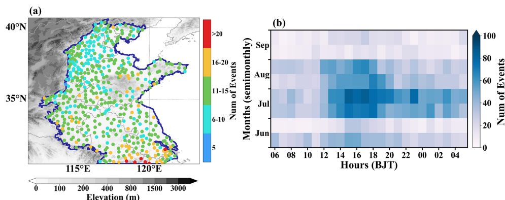
Figure 5. Same as Fig. 4, but for other heavy rainfall events.
