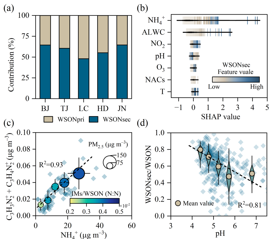
Figure 5. Aqueous formation of N-containing compounds in the NCP. Fractional contribution of primary water-soluble organic nitrogen (WSOnpri) and secondary WSON (WSOnsec) to the total (a); SHAP feature importance assessment for the key factors affecting WSOnsec (b); Linear correlation between IMs-related fragments and \text{NH}_4^+ with different \text{PM}_{2.5} loads (the fragment signals do not represent absolute molecular abundances) (c); panel (d) shows the linear fit regressions for WSOnsec / WSON with pH value across the NCP. (Circles in c and d show grouped mean statistics over all sampling site).
