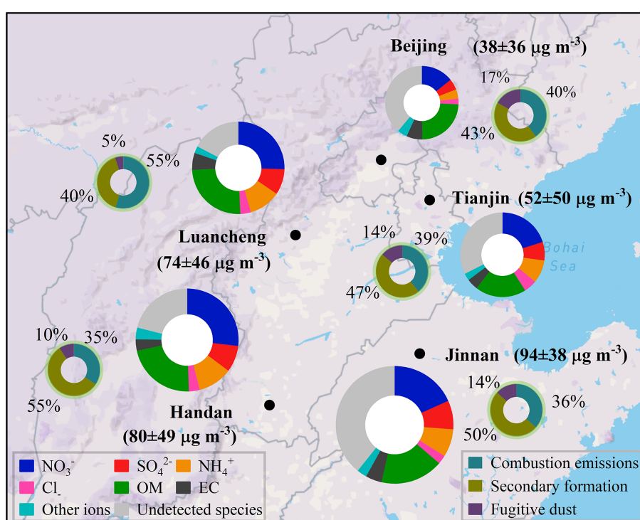
Figure 1. Chemical composition of \text{PM}_{2.5} and sources for organic matters (OM) at different sampling sites. The mass concentration data correspond to \text{PM}_{2.5} . The maps are the reproductions from © Mapbox ( https://account.mapbox.com/ , last access: 3 December 2025).
