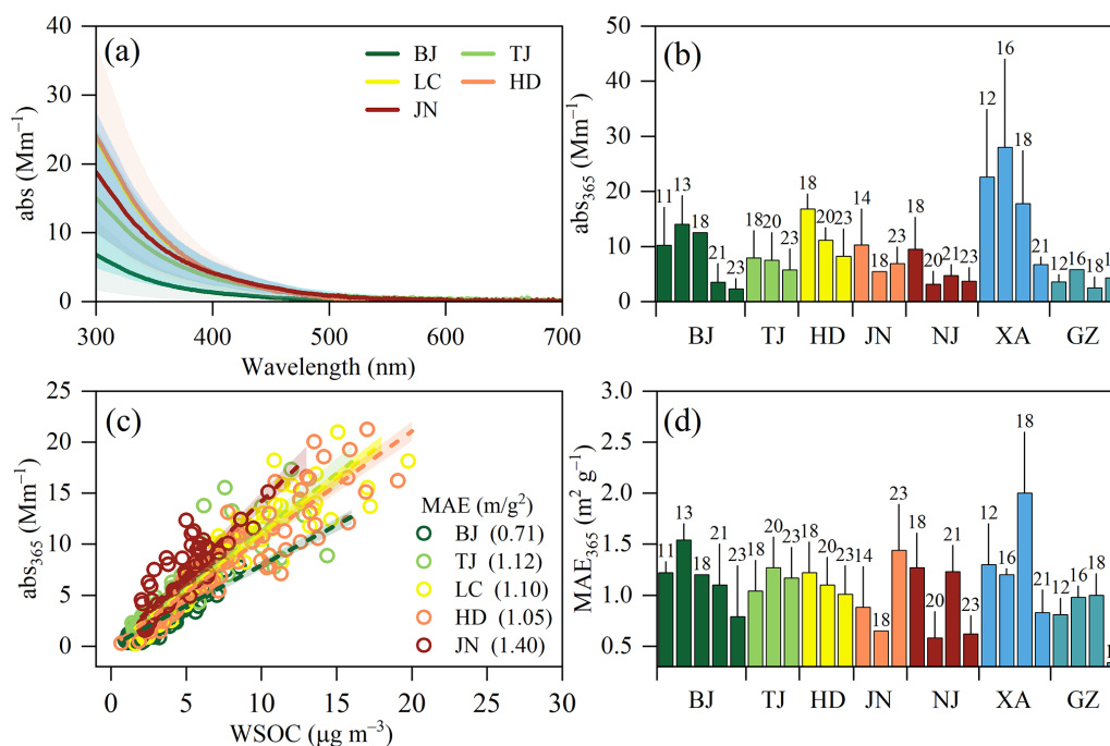
Figure 2. Optical properties of BrC at each sampling site. (a, c) Average absorption spectra and mass absorption coefficient of WSOC; (b, d) Comparison of \text{abs}_{365} and \text{MAE}_{365} in different cities of China (NJ, XA and GZ represent Nanjing, Xi'an and Guangzhou; Superscripts indicate the corresponding years, for instance, the superscript "11" refers to 2011. The datasets of (b) and (d) were derived from the literature, and given in Table S4).
