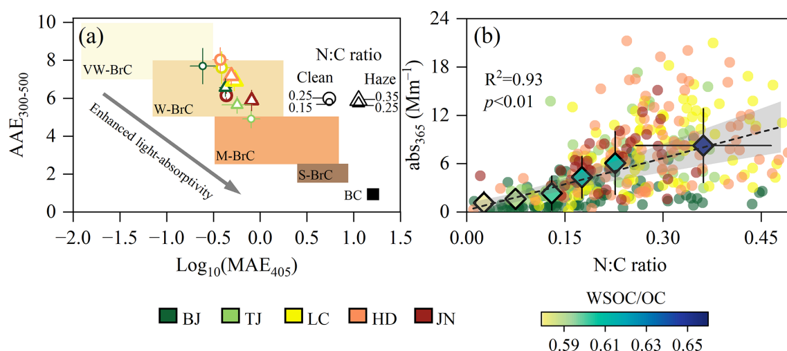
Figure 4. Graphical representation of optical-based BrC classes in \text{Log}_{10}(\text{MAE}_{405}) -AAE space (a). The shaded regions represent very weakly light-absorbing BrC (VW-BrC), weakly light-absorbing BrC (W-BrC), moderately light-absorbing BrC (M-BrC), strongly light-absorbing BrC (S-BrC), and absorbing BC, respectively. Panel (b) shows the linear fit regressions for \text{abs}_{365} with N : C ratio (Diamonds indicate the averaged \text{abs}_{365} and N : C ratio of all sites in each binned N : C interval, with bars representing standard deviations).
