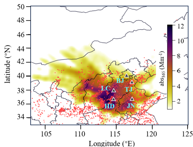
Figure 3. The CWT analysis of BrC at sampling sites along with fire hotspot. Fire hotspot data from Fire Information for Resource Management System (FIRMS) were applied to evaluate open biomass burning intensity during the campaign. The data were acquired from the Visible Infrared Imaging Radiometer Suite (VIIRS) sensor and processed using a fire detection algorithm to identify active fire hotspots.
