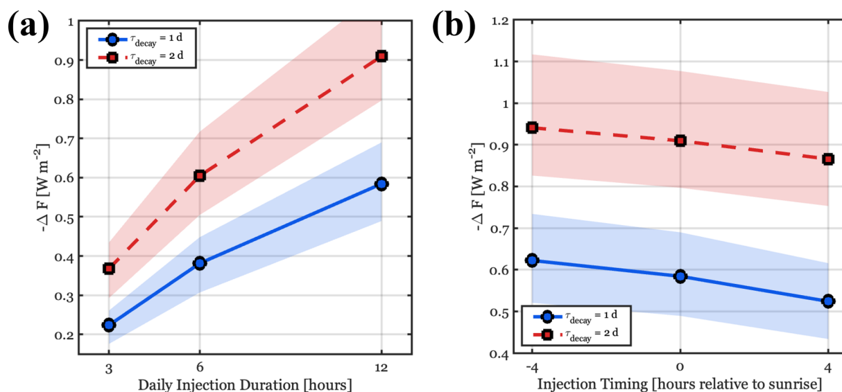
Figure 10. Ensemble-averaged global mean Twomey forcing as a function of (a) the daily injection duration for \tau_{\text{decay}} of 1 and 2 d and (b) the injection timing relative to sunrise, for a 12 h daily injection. Shading corresponds to the IQR of the ensemble. Sensitivity tests use N_{\text{sprayers}} = 4000 .
