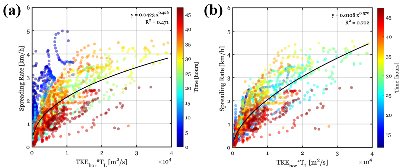
Figure 13. The statistical relationship between particle model-derived spreading rate and \text{TKE}_{\text{hor}} \times T_L for (a) all times and (b) all times excluding the first 10 h after injection. Colors change as a function of time since injection. Black lines indicate the power-law regression, with the equation and R^2 values provided in the upper right hand portion of the panels. All times from all cloudy LES ensemble members are shown.
