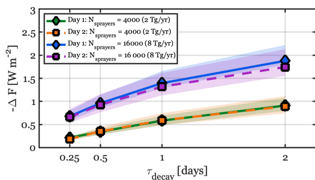
Figure 7. Global mean Twomey forcing ( \Delta F ) as a function of particle lifetime ( \tau_{\text{decay}} ). Green and orange markers correspond to the low-end MCB scenario with N_{\text{sprayers}} = 4000 and blue and purple markers correspond to the mid-range MCB scenario with N_{\text{sprayers}} = 16000 . Each marker represents the ensemble average global mean Twomey forcing and the shading represents the interquartile range (IQR) of the ensemble.
