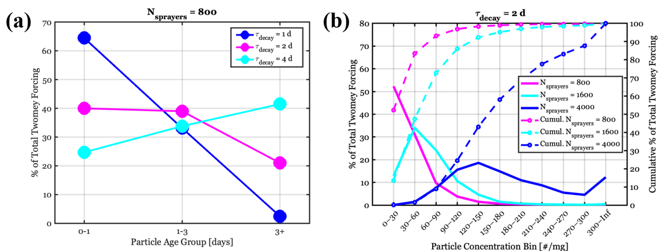
Figure 11. (a) The percent of Twomey forcing as a function of particle age for N_{\text{sprayers}} = 800 and \tau_{\text{decay}} of 1, 2, and 4 d. (b) The percent of Twomey forcing from each particle concentration bin for \tau_{\text{decay}} = 2 d. Bold lines represent the LES ensemble mean percentage of total Twomey forcing (left y axis) and the dashed lines correspond to the cumulative percentage of Twomey forcing going from left to right in the bin space (right y axis). Different colors are for different values of N_{\text{sprayers}} .
