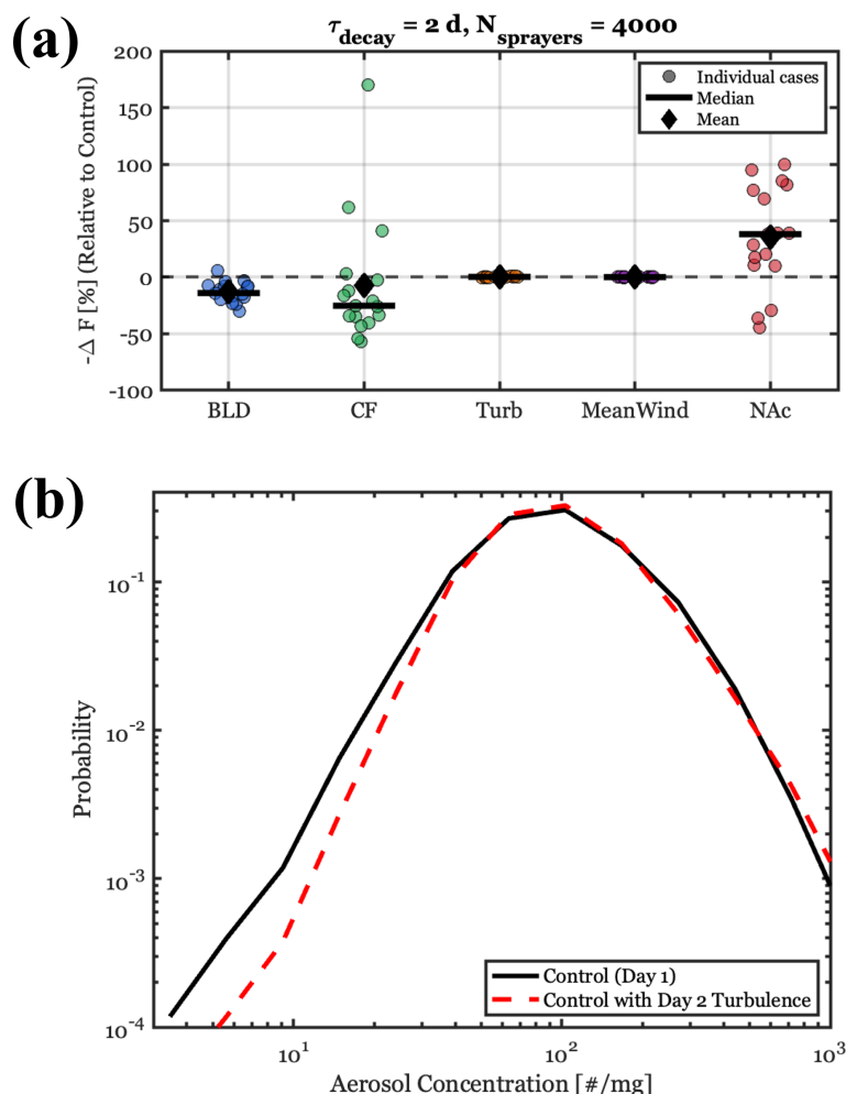
Figure 8. (a) Twomey forcing sensitivity analysis for \tau_{\text{decay}} = 2 \text{ d} and N_{\text{sprayers}} = 4000 , where BLD is the boundary layer depth, CF is the cloud fraction/cloud reflectance, Turb is the particle model turbulence forcing that controls the spreading rate, which includes the C_0 changes related to precipitation, MeanWind is the mean wind, and N_{\text{Ac}} is the background aerosol concentration. Positive percentages indicate that Day 2 values of a given variable act to increase Twomey forcing relative to Day 1 values. The circles represent each LPM simulation, the diamond is the ensemble mean, and the line is the ensemble median. (b) Average aerosol concentration probability distributions across all cases at local noon for the Control (Day 1 regime) and the Control run using Day 2 turbulence forcing in the particle model.
