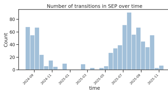
Figure 6. Number of closed-to-open cell transitions identified in the combined EarthCARE-GOES dataset as a function of time.
