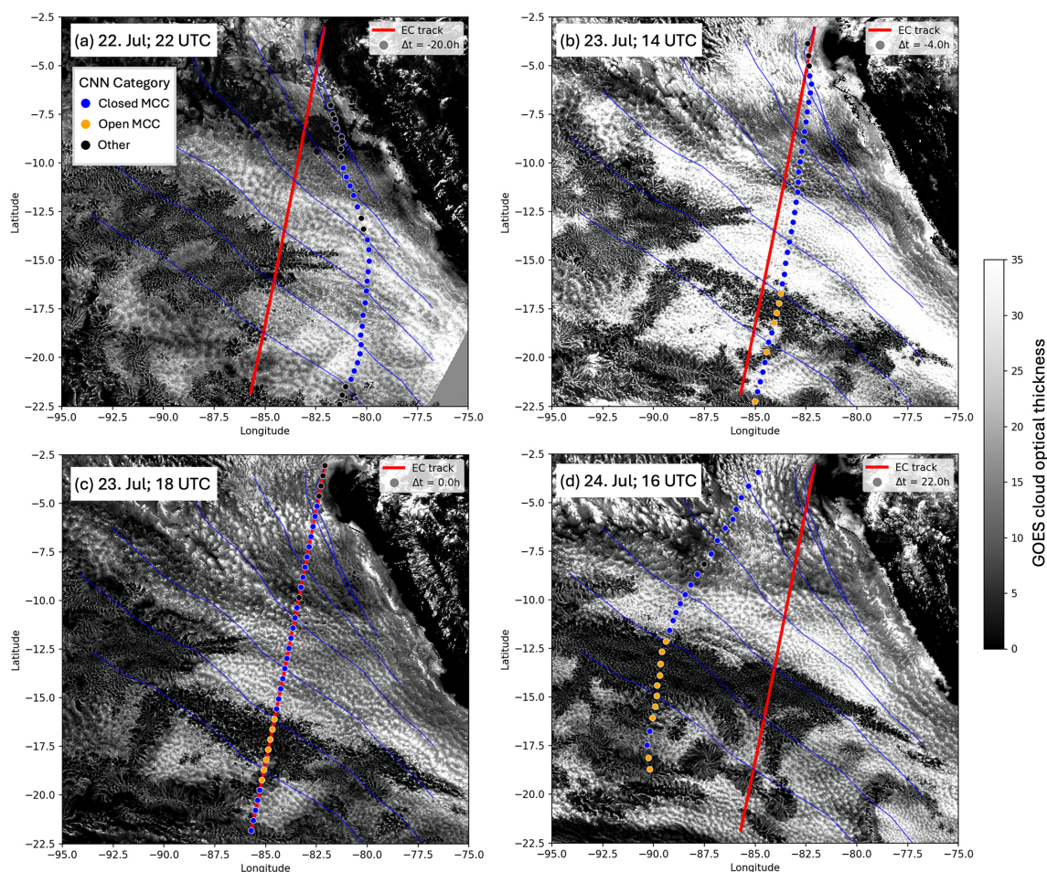
Figure 4. Example illustrating the method used to track cloud structure evolution along trajectories. The panels show GOES COT for four time steps between 22–24 July 2025. The red line shows the location of the EarthCARE overpass, which happened around 18:00 UTC on 23 July. Trajectories are initiated at the time of the EarthCARE overpass (c) and tracked backwards (a, b) and forwards (d) in time. The coloured dots represent the midpoints of each tracked cloud scene (128 km \times 128 km), with colours indicating the mesoscale cloud type retrieved by applying the CNN to the GOES imagery. Thin blue lines indicate the full trajectories for a subset of these scenes.
