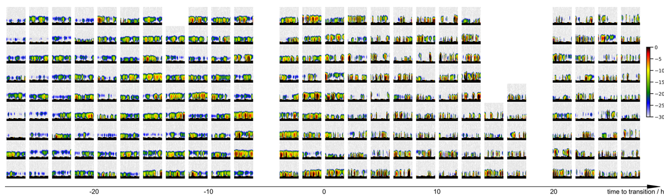
Figure D4. Same as Fig. D1, but for CPR reflectivity. The scenes correspond to the ones shown in Fig. D1.
