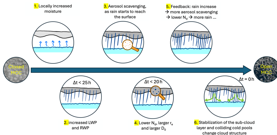
Figure 14. Hypothesised timeline for the processes leading to a transition from closed to open cells.
