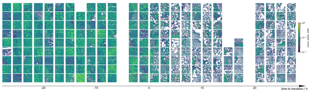
Figure D1. M-COP LWP for example cloud scenes for which closed-to-open cell transitions were identified. The scenes are ordered from left to right by their time to transition, using the same time-to-transition bins as in Figs. 11, 12 and 13. For each time to transition value, nine scenes were picked randomly. For some time-to-transition values less than nine scenes were found overall, and for time-to-transitions = −5 and 19 h no corresponding scenes were found (see Fig. 11a).
