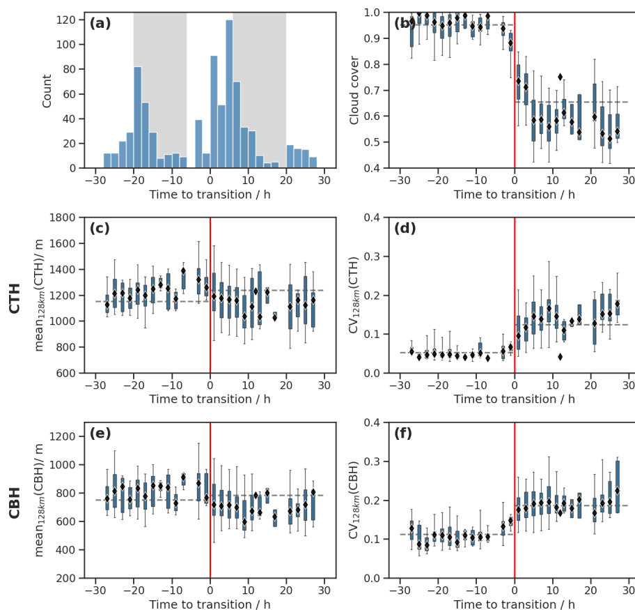
Figure 11. Cloud properties of all cloud scenes in which closed-to-open cell transitions were identified, as a function of their time to transition (=time of EarthCARE overpass – time of transition; determined from GOES morphology along trajectories). Negative time-to-transition values correspond to clouds that were still closed cells during the EarthCARE overpass and transitioned subsequently, while positive values correspond to scenes that had already transitioned prior to the overpass and could be traced back to an earlier transition time. (a) number of cloud scenes that were found for different time-to-transition values. Grey shading indicates that the transition happens during local nighttime. (b) cloud cover computed from M-COP; (c)–(f) cloud vertical structure from ACM-CAP. The box plots in (b)–(f) represent the distribution of \text{mean}_{128\text{km}} and \text{CV}_{128\text{km}} values of cloud parameters for all scenes with the same time-to-transition. Black diamonds indicate the medians of these distributions. The blue bars indicate the values between 25th and 75th percentile, whiskers are from 5th to 95th percentile. Horizontal dashed, grey lines indicate the “climatological” median values for closed and open cells, derived from the closed and open cell distributions in Fig. 8. These serve as a reference for comparing with the medians of the box plots (i.e. of the cloud scenes for which transitions were identified).
