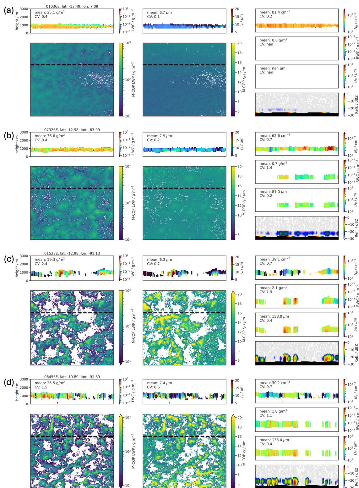
Figure 7. Examples of two typical closed-cell (a, b) and two typical open-cell (c, d) cloud scenes. Larger subplots show M-COP LWP and r_e for the four 128 km \times 128 km scenes. The smaller subplots show the corresponding ACM-CAP profiles along-track (black dashed line in M-COP images) for several cloud and rain variables, namely liquid water content, r_e , N_d , RWC and D_0 . The bottom right subplot shows the CPR reflectivity for each scene. The orbits and mid-points of the four scenes are specified in the titles. Numbers at the top left in ACM-CAP subplots are the mean and CV taken over the 128 km along-track scenes.
