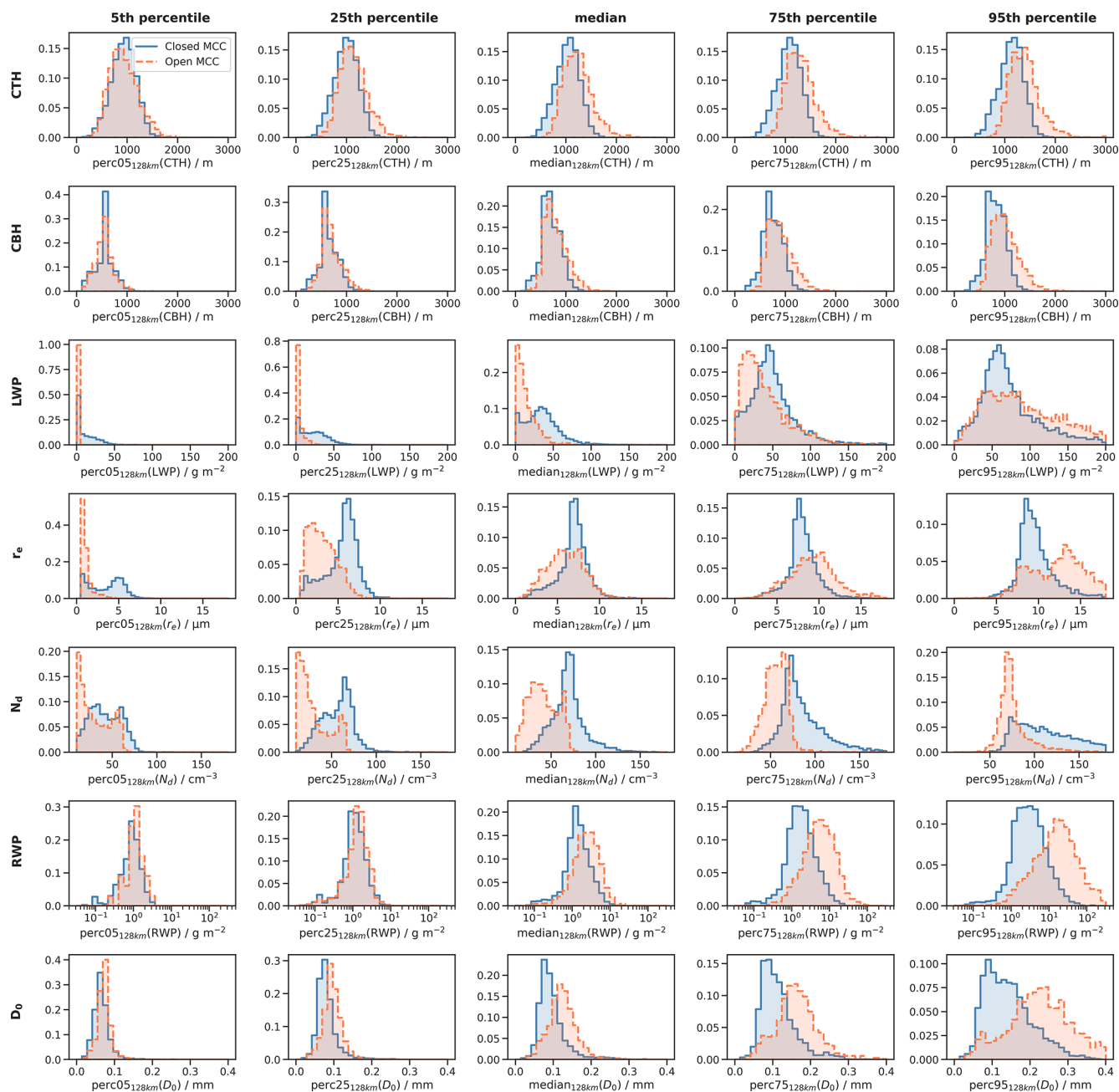
Figure B1. Same as Fig. 8, but for percentiles and median per cloud scene.
