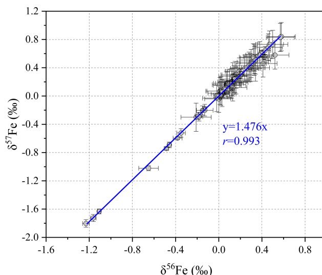
Figure 2. Comparison of \delta^{56}\text{Fe} versus \delta^{57}\text{Fe} values measured in our work. All the individual measurements (84 in total, including measurements of standards) conducted in this work are presented in this figure.
