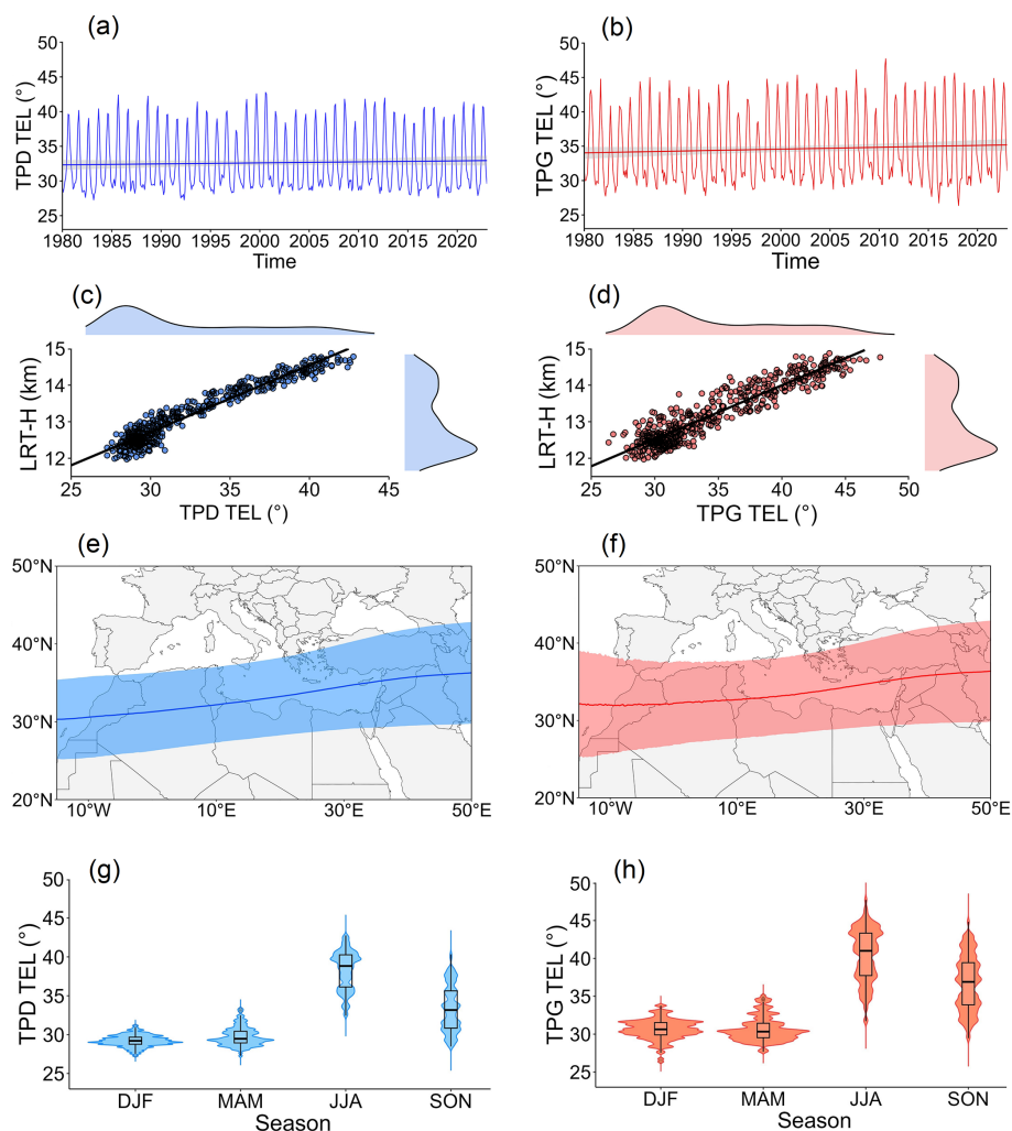
Figure 2. Monthly time series of the (a) TPD TEL method and (b) TPG TEL method, the shaded bands surrounding the trend lines denote the 95 % confidence intervals of the fitted trends. The linear regression model between TPD TEL and LRT-H (c) and the linear regression model between TPG TEL and LRT-H (d), the marginal probability density functions (PDFs) of the variables are shown above and to the right of each scatter plot. Longitudinal variation of TEL using both methods over the Mediterranean region is displayed. The blue line in (e) represents the mean TPD TEL at each longitude over the study period, while the blue shading depicts its SD. In (f), the red line represents the mean TPG TEL at each longitude over the study period, with the red shading indicating its SD. Seasonal variation of TPD TEL (g) and TPG TEL (h) shown as violin plots. The width of each violin represents the probability density of the seasonal TEL values. The central box indicates the interquartile range (25th–75th percentiles); the horizontal line inside the box marks the median.
