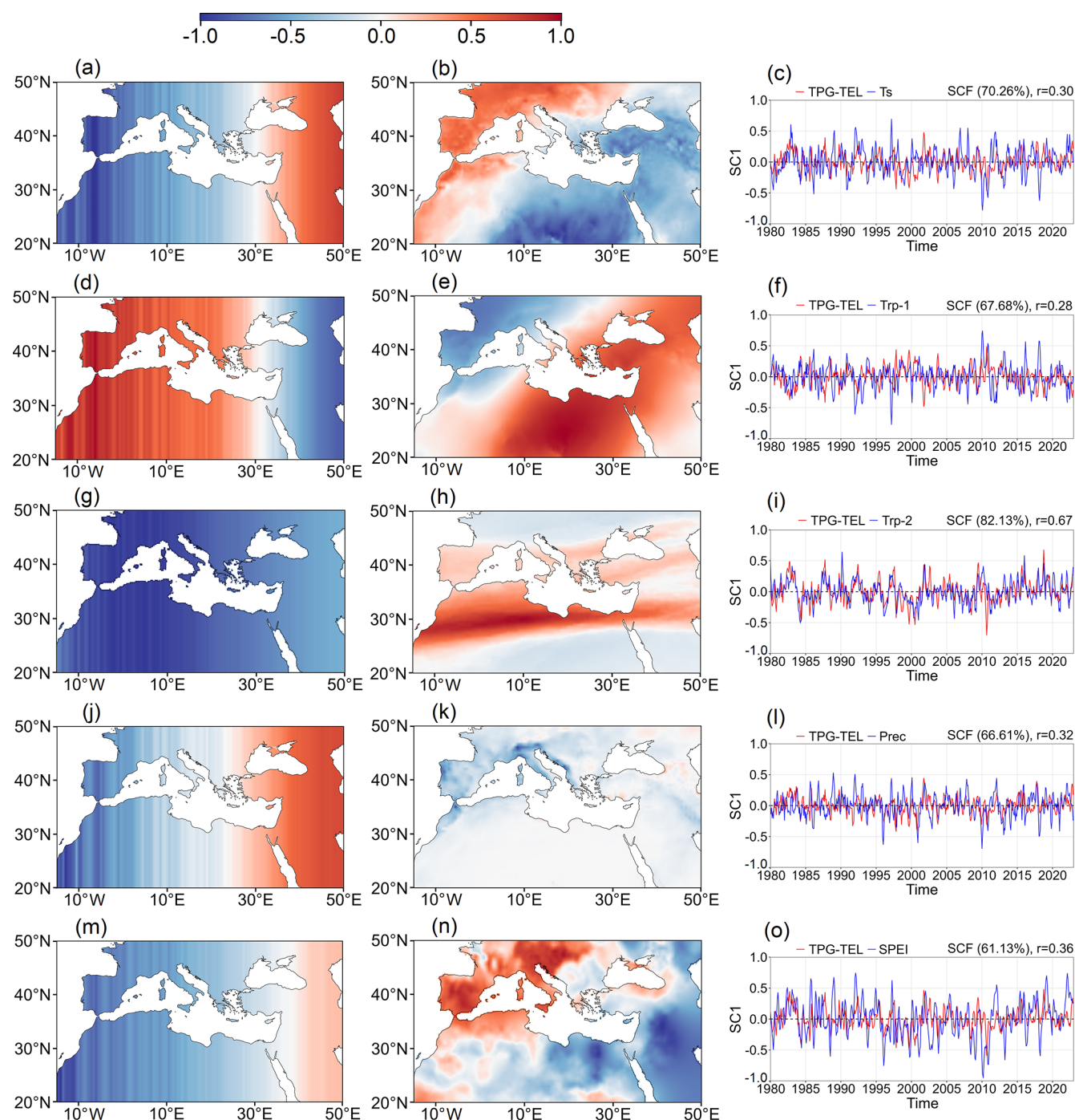
Figure 6. First leading mode of covariability as in Fig. 4, but for TPG TEL and the corresponding climatic parameters.
