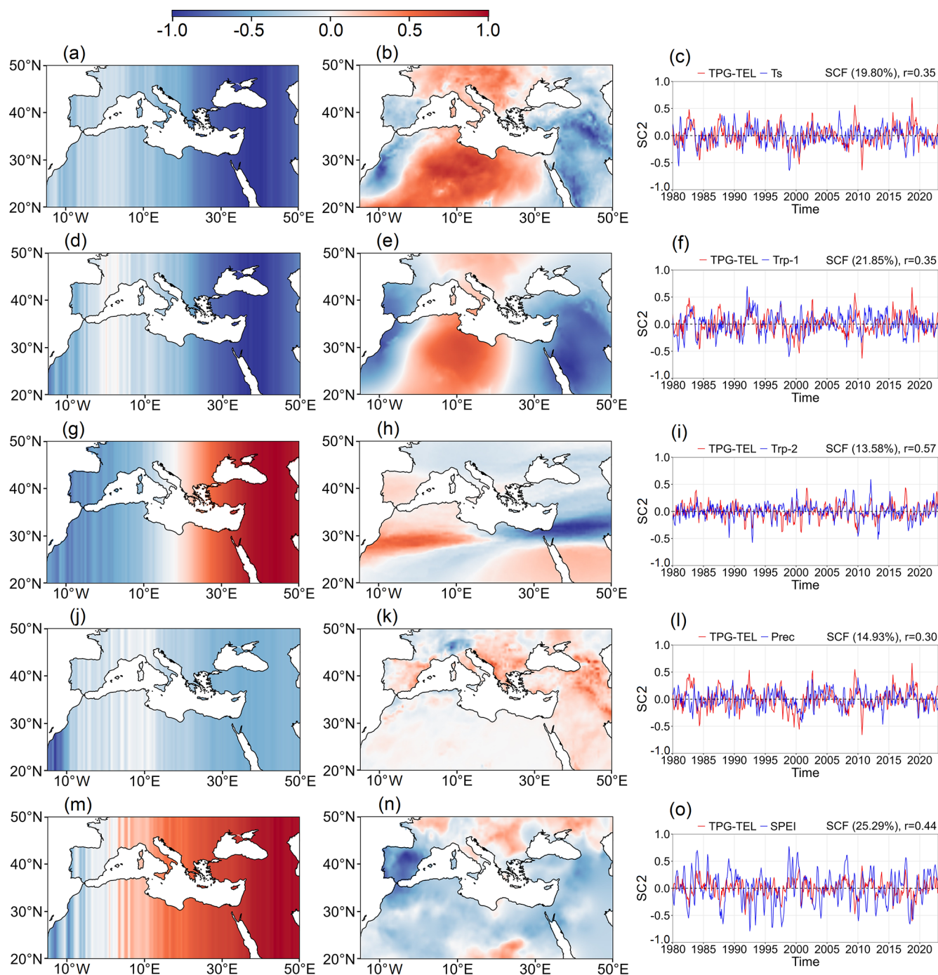
Figure 7. Second leading mode of covariability as in Fig. 5, but for TPG TEL and the corresponding climatic parameters.
