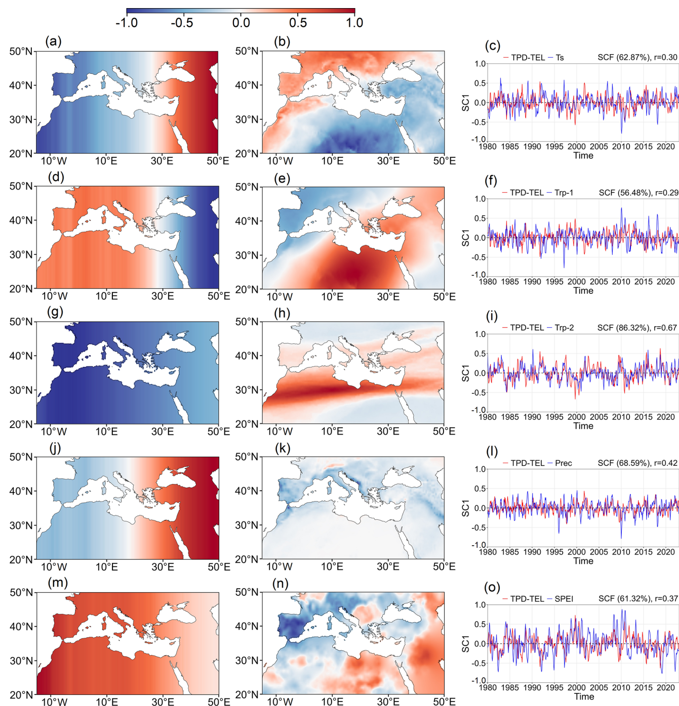
Figure 4. First leading mode of covariability for the coupled fields of TPD TEL and climatic parameters. TPD TEL and Ts ( a, b, c ), TPD TEL and Trp-1 ( d, e, f ), TPD TEL and Trp-2 ( g, h, i ), TPD TEL and precipitation ( j, k, l ), and TPD TEL and SPEI ( m, n, o ). The spatial patterns for the first paired mode of covariability (SVD1) of TPD TEL (left), climatic parameter SVD1 (middle), and the time series of expansion coefficients (SC1) for the paired mode of both TPD TEL and climatic parameters (right).
