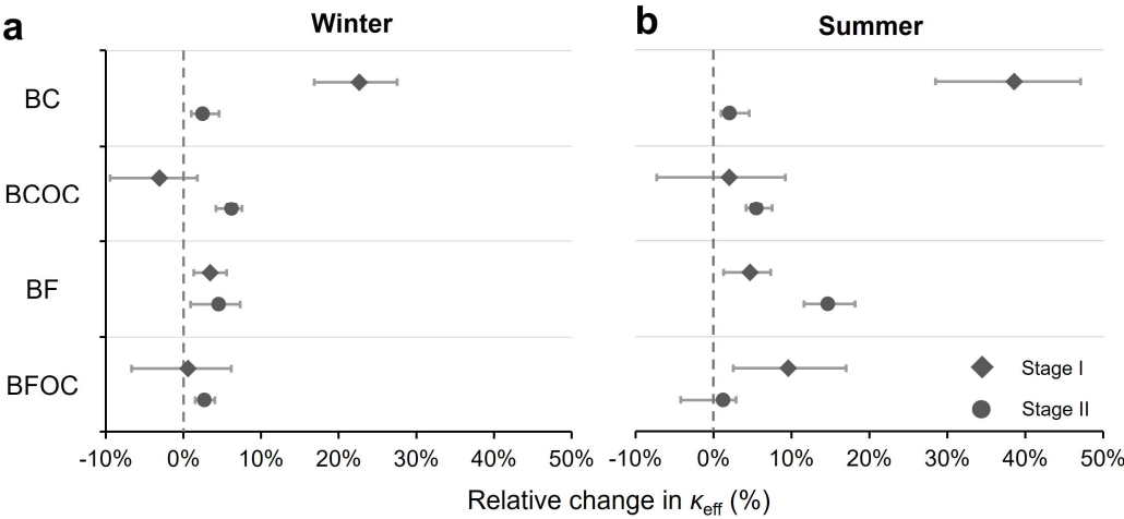
39 Figure S4. Sensitivity analysis of stage-specific relative changes in inferred effective 40 hygroscopicity parameter ( \kappa_{\text{eff}} ) for four particle classes in winter (a) and summer (b). 41 Diamonds and circles represent the baseline estimates for Stages I and II, respectively. 42 Horizontal bars show the ranges obtained from four combinations of the lower and 43 upper hygroscopicity values for ammonium sulfate and ammonium nitrate listed in 44 Table S3. The dashed line denotes zero change; ranges crossing zero indicate that the 45 direction of change was not consistent across the tested parameter combinations.
