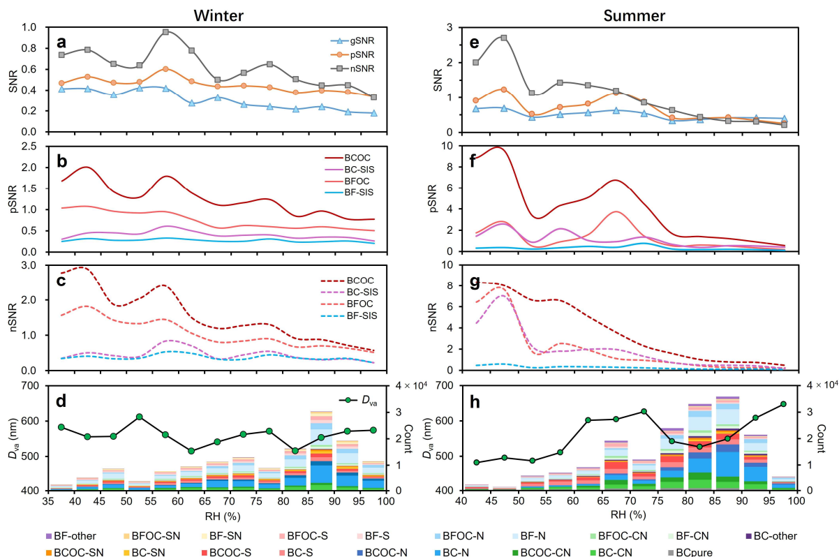
Figure S5. Variations in sulfur-to-nitrogen ratios (SNR) with relative humidity (RH) for different aerosol particle types during winter (a-d) and summer (e-h). (a, e) Trends of gas-phase (gSNR), particle-phase (pSNR), and number-based (nSNR) ratios across the RH gradient; (b, f) pSNR variations with RH for aged-like BC-containing and BC-free particle types; (c, g) nSNR trends across different aged-like particle types as a function of RH; (d, h) Corresponding changes in vacuum aerodynamic diameter ( D_{va} , green line, left axis) and number concentration (bars, right axis) of individual particle types with RH.
