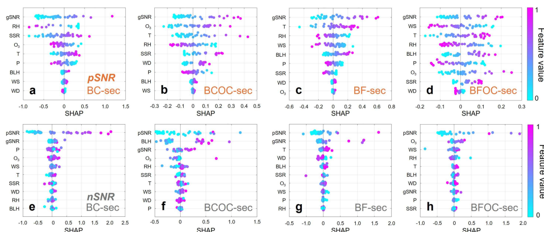
Figure S7. SHAP summary plots show the relative importance of predictors for particle-phase (pSNR; a-d) and number-based (nSNR; e-h) sulfur-to-nitrogen ratios.
