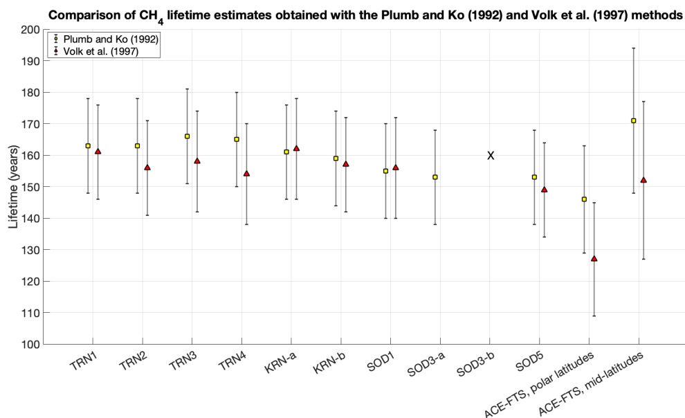
Figure 7. Calculated \text{CH}_4 lifetime for AirCore samples and ACE-FTS observations obtained following the methods of Plumb and Ko (1992) and Volk et al. (1997). The missing estimates for SOD3-b are marked as an “X”.
