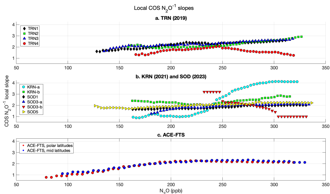
Figure 4. Local \text{COS N}_2\text{O}^{-1} slopes ( \text{ppt ppb}^{-1} ) obtained from AirCore and ACE-FTS profiles.
