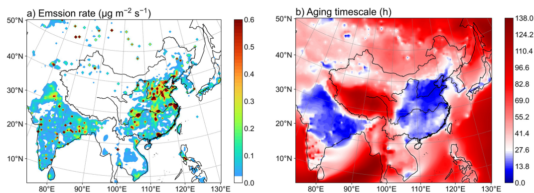
Figure 2. Spatial distributions of the aerosol precursor ( \text{SO}_2 + \text{OC} + \text{BC} ) emission rate ( a , \mu\text{g m}^{-2} \text{s}^{-1} ) and BC aging timescale ( b , h) over East Asia in summer during 2008–2021 in the Exp. 8.
