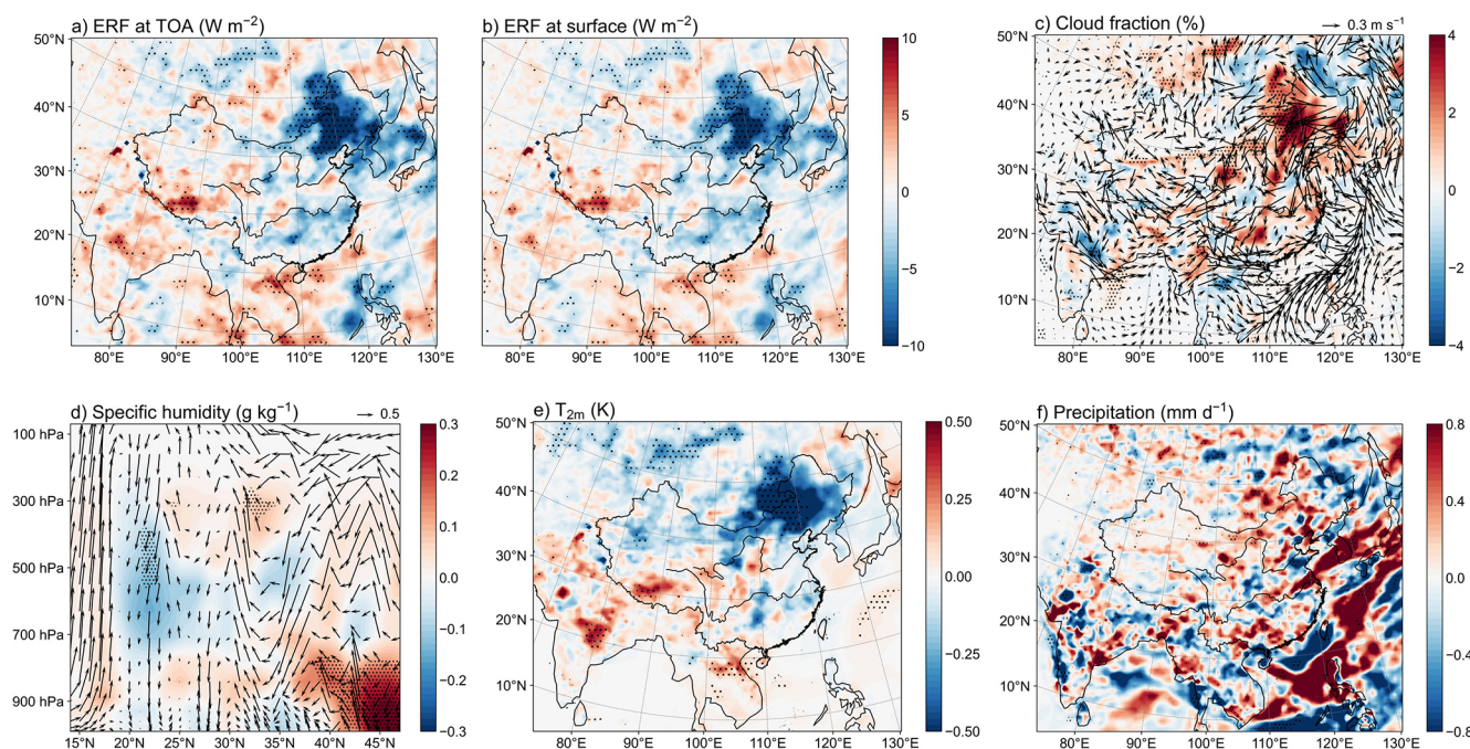
Figure 11. Spatial distributions of the nonlinear interaction term under the dynamic aging scheme (Dyn_I) for the BC effective radiative forcing (ERF) at TOA and surface (a, b, \text{W m}^{-2} ), wind field (arrow, \text{m s}^{-1} ) and cloud fraction (shaded, %) (c) near 850 hPa, meridional circulation (arrow) and specific humidity (shaded, \text{g kg}^{-1} ) (d) in the altitude–latitude section averaged from 112 to 122° E, surface temperature at 2 m ( T_{2m} ) (e, K) and precipitation (f, \text{mm d}^{-1} ) over East Asia in summer during 2008–2021. Black-dotted regions denote statistically significant differences at the 90 % confidence level based on a two-sided paired Student's t -test.
