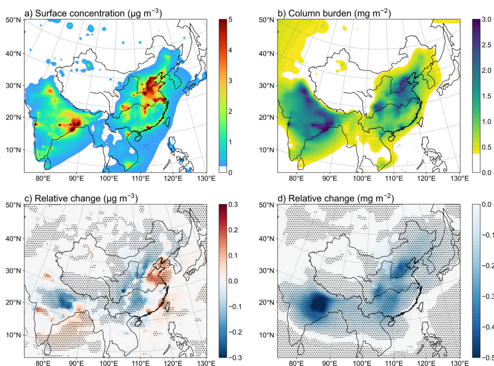
Figure 3. Spatial distributions of the BC surface concentration ( a , \mu\text{g m}^{-3} ) and column burden ( b , \text{mg m}^{-2} ) over East Asia in summer during 2008–2021 in the Exp. 8. Relative changes in the BC surface concentration ( c , \mu\text{g m}^{-3} ) and column burden ( d , \text{mg m}^{-2} ) over East Asia in summer during 2008–2021 between the Exps. 8 and 4. Black-dotted regions denote statistically significant differences at the 90 % confidence level based on a two-sided paired Student's t -test.
