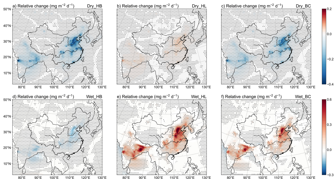
Figure 4. Relative changes in the dry deposition flux (a–c, \text{mg m}^{-2} \text{d}^{-1} ) and wet deposition flux (d–f, \text{mg m}^{-2} \text{d}^{-1} ) of hydrophobic BC (HB, left), hydrophilic BC (HL, center) and total BC (BC, right) over East Asia in summer during 2008–2021 between the Exps. 8 and 4. Black-dotted regions denote statistically significant differences at the 90 % confidence level based on a two-sided paired Student's t -test.
