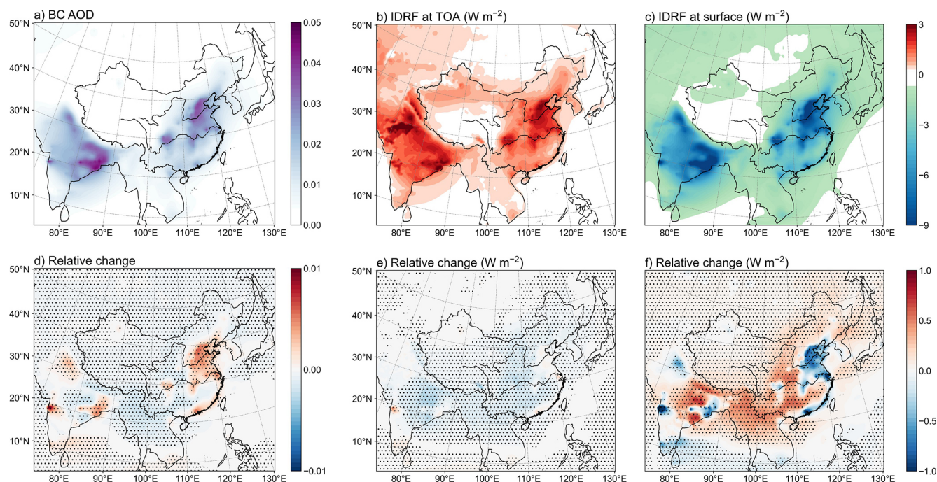
Figure 5. Spatial distributions of the BC aerosol optical depth (a), instantaneous direct radiative forcing (IDRF) at the TOA and surface (b, c, \text{W m}^{-2} ) over East Asia in summer during 2008–2021 in the Dyn_Dir experiment. Relative changes in the BC AOD (d), IDRF at the TOA and surface (e, f, \text{W m}^{-2} ) over East Asia in summer during 2008–2021 between the Dyn_Dir and Def_Dir experiments. Black-dotted regions denote statistically significant differences at the 90 % confidence level based on a two-sided paired Student's t -test.
