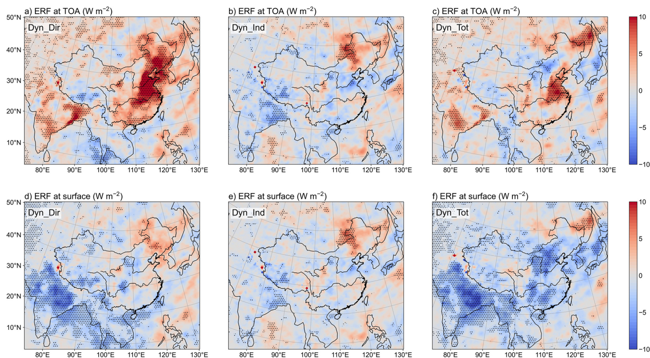
Figure 9. Spatial distributions of the BC effective radiative forcing (ERF) at the TOA and surface (a–c, d–f, \text{W m}^{-2} ) over East Asia in summer during 2008–2021 in the Dyn_Dir (left), Dyn_Ind (center) and Dyn_Tot (right) experiments. Black-dotted regions denote statistically significant differences at the 90 % confidence level based on a two-sided paired Student's t -test.
