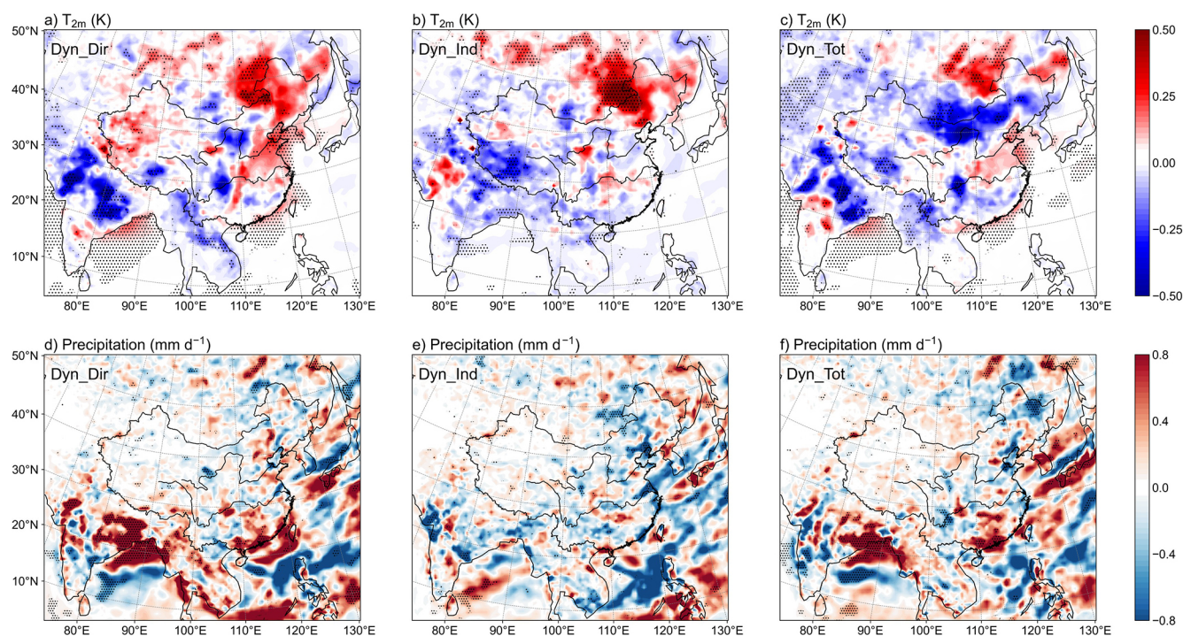
Figure 10. Changes in the surface air temperature at 2 m ( T_{2m} ) (a–c, K) and precipitation (d–f, \text{mm d}^{-1} ) over East Asia in summer during 2008–2021 in the Dyn_Dir (left), Dyn_Ind (center) and Dyn_Tot (right) experiments. Black-dotted regions denote statistically significant differences at the 90 % confidence level based on a two-sided paired Student's t -test.
