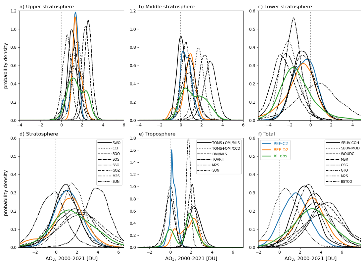
Figure 5. Kernel density estimates (KDEs) of DLM background trend change (2000–2021) in tropical ozone columns from observations (black lines for individual data sets, green lines for the multi-observational distributions), REF-C2 (blue), and REF-D2 (orange). Results from observational datasets starting in 2005 (i.e., OMI/MLS, SUNLIT, M2S) have been scaled to represent changes over the 2000–2021 period instead of the 2005–2021 period.
