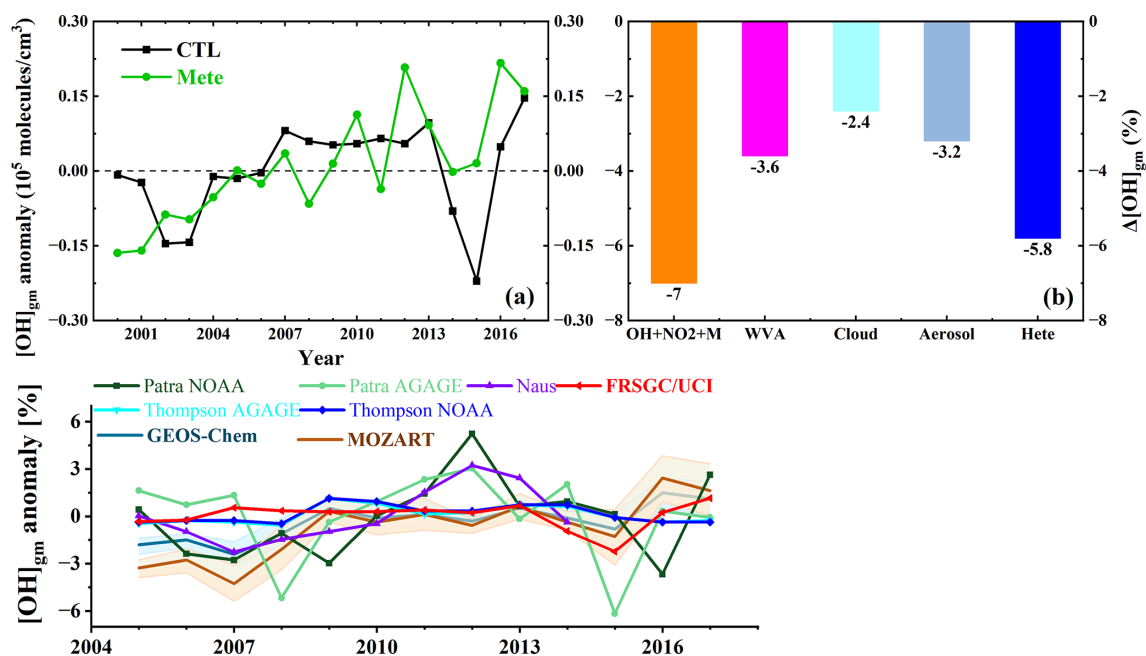
Figure 10. (a) The anomaly of [\text{OH}]_{\text{gm}} ( 10^5 \text{ molec. cm}^{-3} ) in the control run (CTL) and fixed emission run (labelled “Mete”), (b) the relative differences in annual mean [\text{OH}]_{\text{gm}} (%) between CTL and the respective sensitivity runs, averaged over 2000–2017, and (c) the relative [\text{OH}]_{\text{gm}} anomalies (%) from this work (FRSGC/UCI) and other studies. The labels in panel (b) match those in Fig. 7. Results based on the MOZART and GEOS-Chem chemical mechanisms in panel (c) are from Zhao et al. (2025), the MCF-based inversion estimates are from Patra et al. (2021) and Naus et al. (2019), and the HFC-based inversion estimates are from Thompson et al. (2024).
