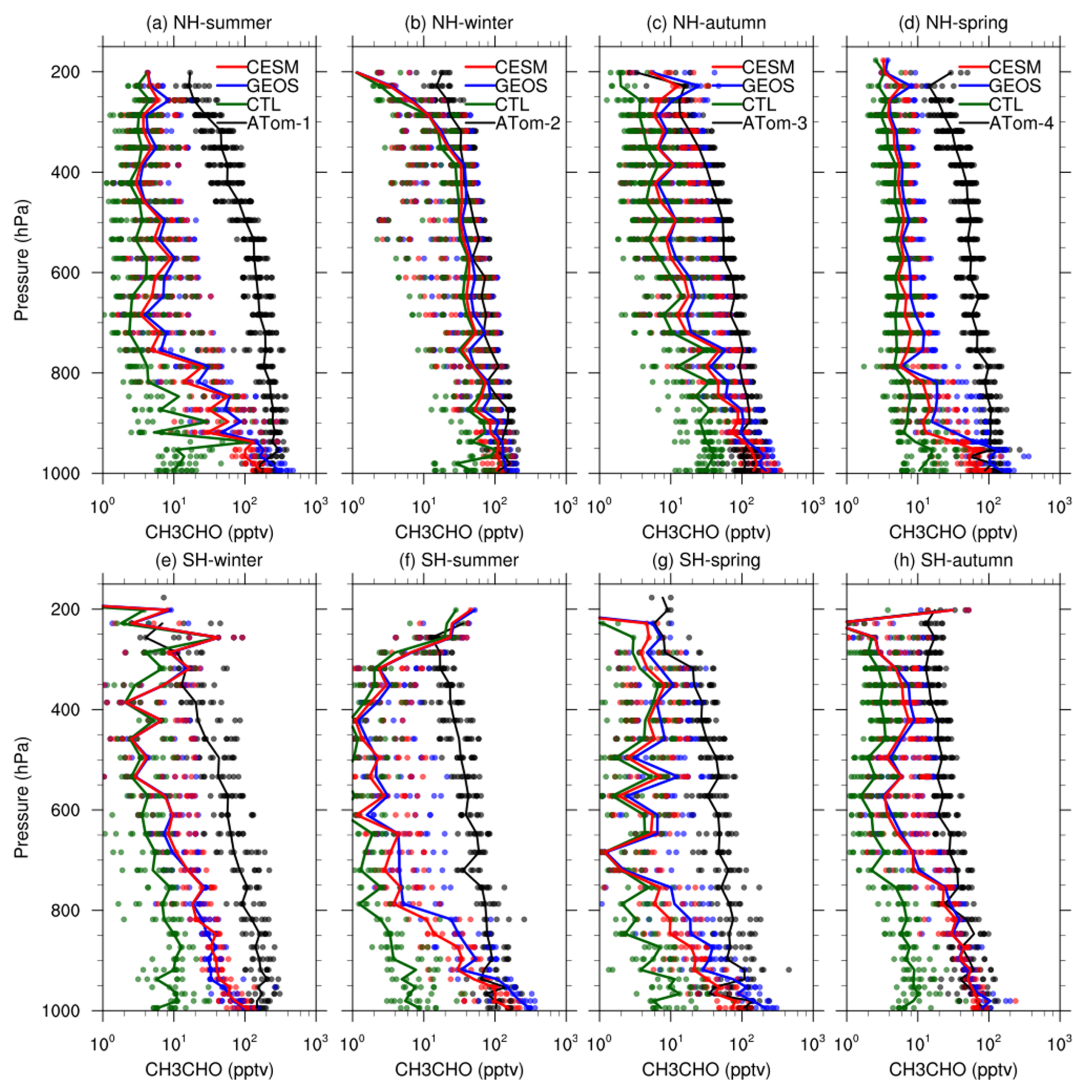
Figure 8. As Fig. 5, but for \text{CH}_3\text{CHO} (pptv). The model control run (CTL) is shown in green, with results from model runs using emissions from CESM and GEOS-Chem shown in red and blue respectively.
