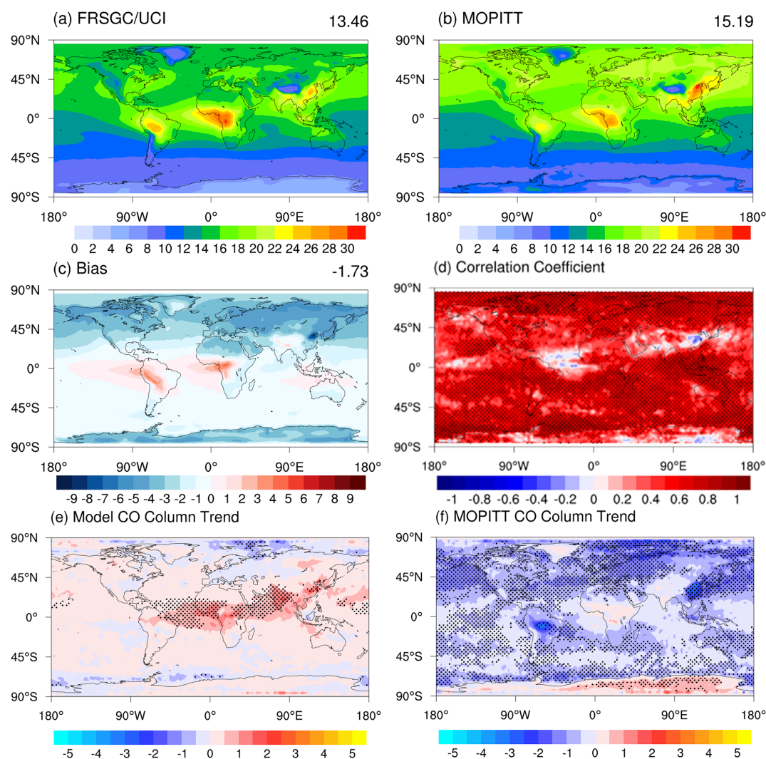
Figure 4. Same as Fig. 1, but for total CO column ( 10^{17} molec. \text{cm}^{-2} ) and annual mean total CO column trends ( 10^{16} molec. \text{cm}^{-2} \text{yr}^{-1} ).
