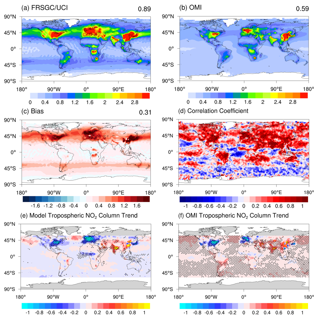
Figure 3. Same as Fig. 2, but for tropospheric NO 2 column ( 10^{15} molec. \text{cm}^{-2} ) and annual mean tropospheric NO 2 column trends ( 10^{14} molec. \text{cm}^{-2} yr -1 ).
