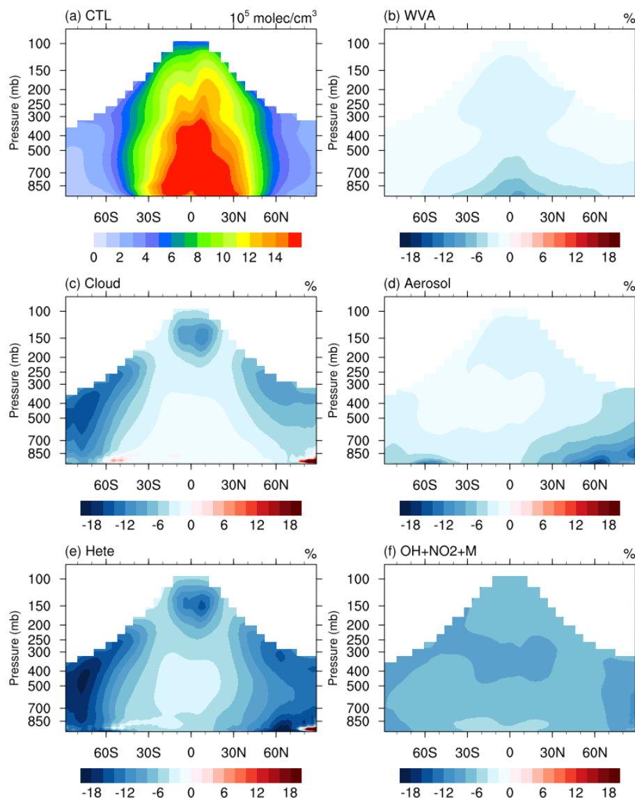
Figure 7. (a) Zonal mean (latitude–pressure) cross sections of annual mean OH concentration ( 10^5 \text{ molec. cm}^{-3} ) in the CTL run and the effects on tropospheric OH (in %) of (b) water vapor UV absorption (WVA), (c) cloud heterogeneous reactions (Cloud), (d) aerosol heterogeneous reactions (Aerosol), (e) all heterogeneous reactions (Hete), and (f) the updated OH + NO 2 reaction rate. Percentage differences are calculated as (\text{CTL} - \text{experiment})/\text{CTL} \times 100 \% . The troposphere was defined as the region below a climatological tropopause ( p = 300 - 215(\cos(\text{lat}))^2 ) following Lawrence et al. (2001).
