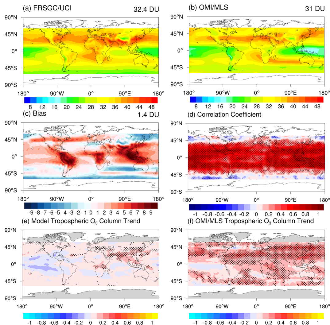
Figure 2. Multiyear average (2005–2017) tropospheric O 3 column (DU) from (a) the model control run and (b) OMI/MLS satellite observations. Panel (c) shows the corresponding mean bias of the tropospheric O 3 column (model minus observation), and (d) shows the correlation coefficient between annual mean modelled and OMI/MLS tropospheric O 3 column time series at each grid box. Annual mean tropospheric O 3 column trends (DU yr -1 ) are shown in (e) for the model and (f) for satellite observations over the 2005–2017 period. Global mean columns between 60° S–60° N are indicated in the upper right corner of panels (a)–(c). Shaded areas in (d) indicate regions where the correlation is statistically significant at the 95 % confidence level ( p < 0.05 ). Trends in panels (e) and (f) were calculated using the Theil–Sen method, and stippling indicates areas with significant trends at the 95 % confidence level according to the Mann–Kendall test.
