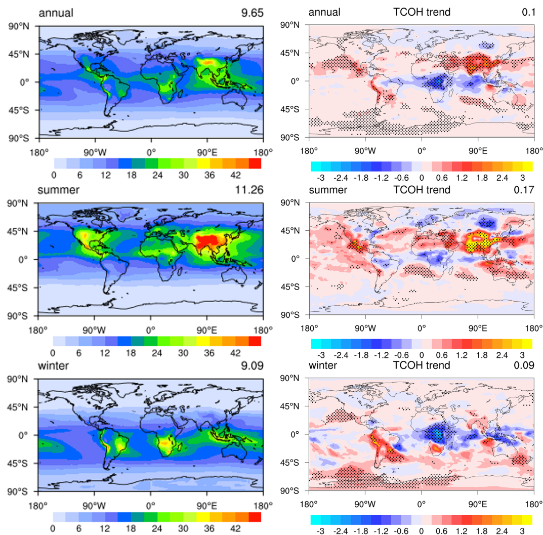
Figure 9. The tropospheric column of OH (TCOH, 10^{12} \text{ molec. cm}^{-2} , left panels) and the trend ( 10^{11} \text{ molec. cm}^{-2} \text{ yr}^{-1} , right panels) in annual, winter and summer from 2000 to 2017. The troposphere was defined as the region below a climatological tropopause ( p = 300 - 215(\cos(\text{lat}))^2 ) following Lawrence et al. (2001). Trends are calculated as in Fig. 2. The value in the right corner is the global average.
