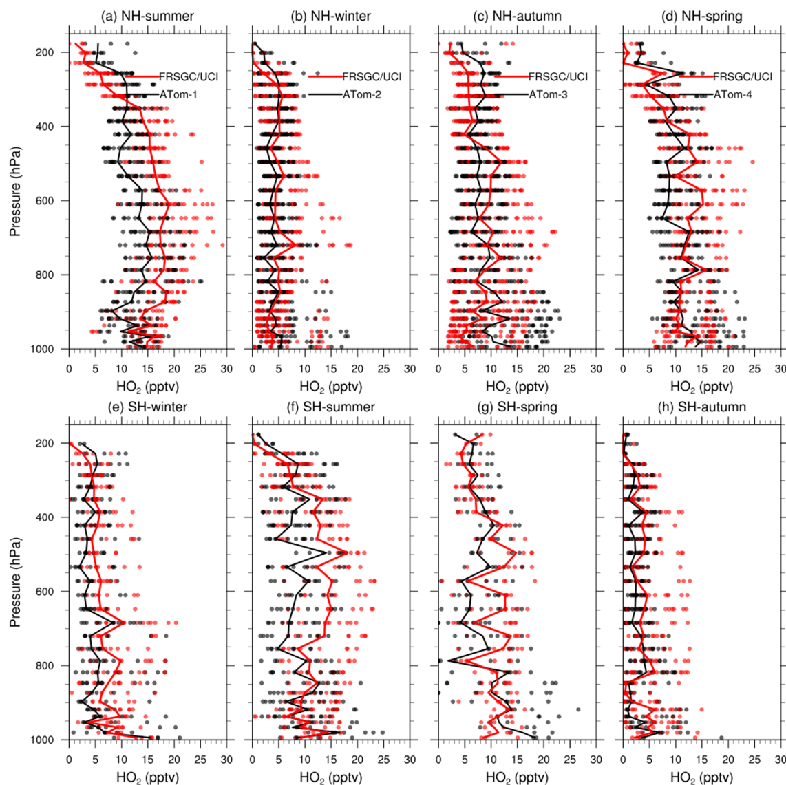
Figure 6. As Fig. 5, but for HO 2 (pptv).
