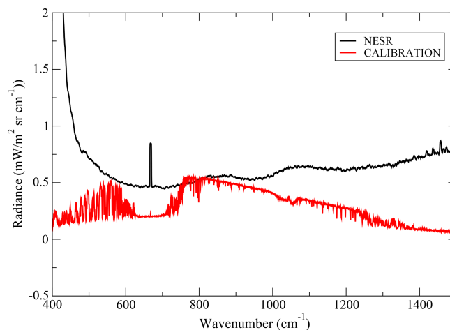
Figure 10. Comparison of the FINESSE Noise Equivalent Spectral Ratio (NESR, black curve) and the calibration systematic error (red curve).
