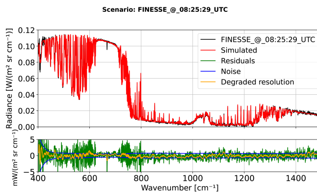
Figure 21. Upper panel: comparison of the simulated spectrum at the last retrieval algorithm iteration (red curve) with the FINESSE measured spectral radiance (black curve) at 30 329 s since midnight (08:25:29 UTC, scenario 4) on 17 February 2023. Lower panel: the residuals (green curve) are reported in comparison with the noise (blue curves), along with the degraded curve (orange).
