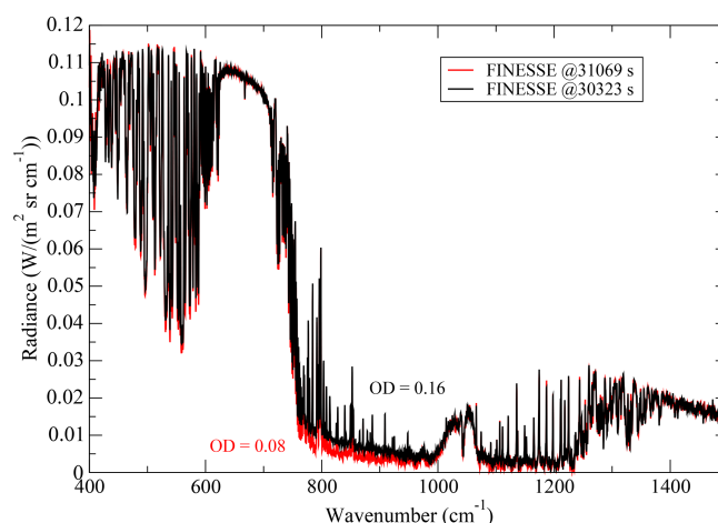
Figure 16. Spectra measured by FINESSE in the presence of cirrus at 30 323 and 31 069 s since midnight (08:25:23 and 08:37:49 UTC) on 17 February 2023. The associated retrieved cirrus optical depths are also provided.
