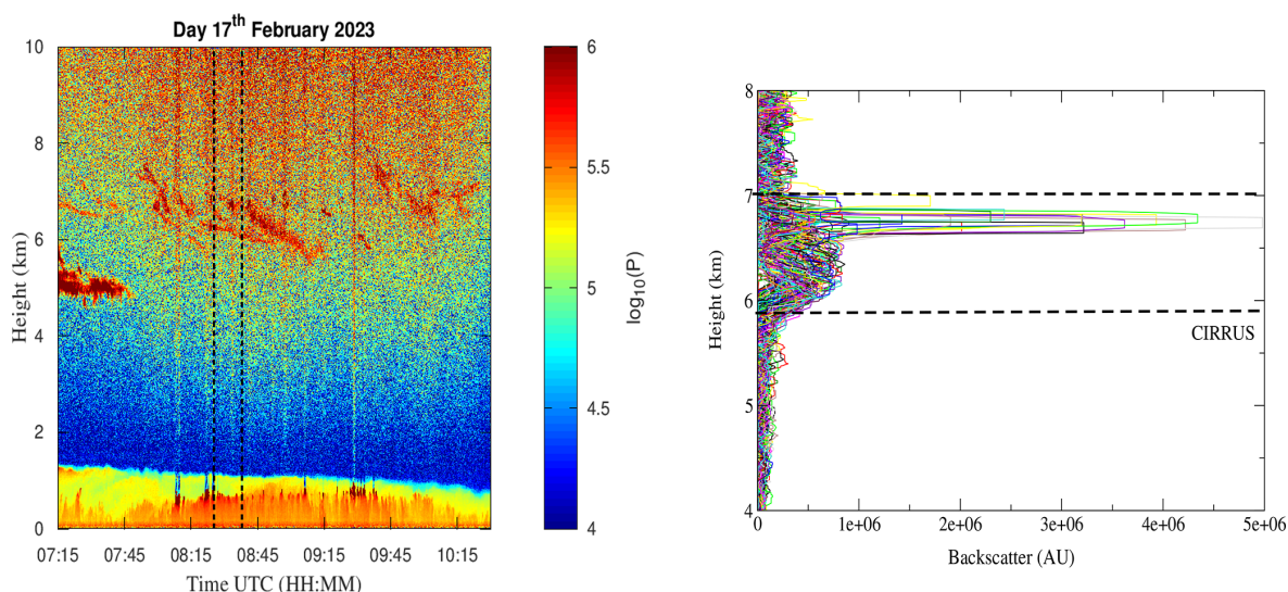
Figure 7. Left: Logarithmic backscattering signal ( P , in arbitrary unit (AU)) detected by the Met-Norway ceilometer on 17 February 2023 showing the passage of cirrus clouds between 07:15 and 10:30 UTC. The dashed vertical black dashed lines at 08:25 and 08:38 UTC delimit the time window of the FINESSE measurements selected for analysis. Right: Individual backscattering profiles obtained during the 08:25–08:38 UTC time window.
