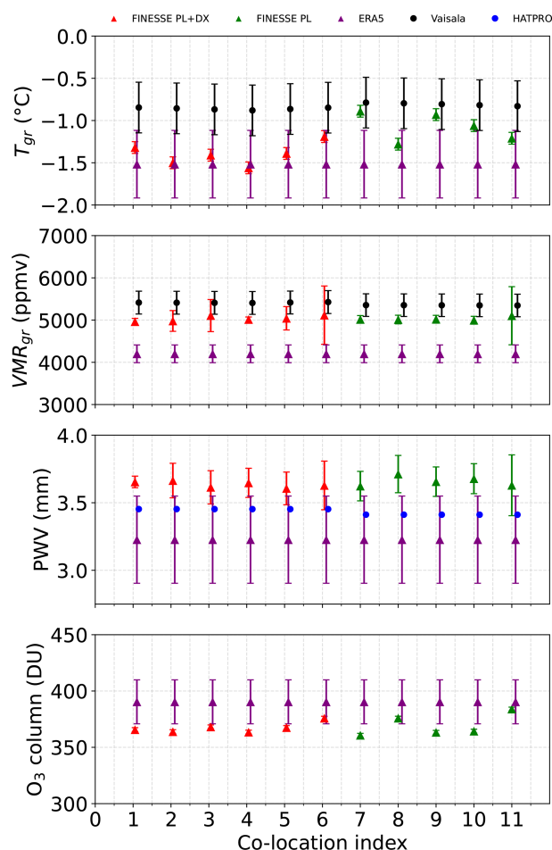
Figure 14. Top panel: comparison of the temperature at ground retrieved from FINESSE spectra (red and green triangles), measured by the Vaisala probe (black dots) and ERA5 (violet triangles) for each scenario. Second panel: same comparison as the temperature but for water vapour mixing ratio (VMR). Third panel: comparison of precipitable water vapour (PWV), retrieved from FINESSE (red and green triangles), from integrated HATPRO retrievals (blue dots) and from ERA5 (violet triangles). Bottom panel: comparison of the ozone total column retrieved from FINESSE and provided by ERA5.
