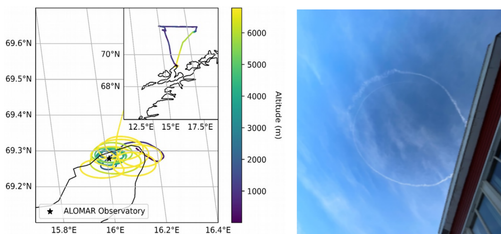
Figure 2. Left: Main image – Flight track of INCAS KA on 17 February 2023 over ALOMAR between 08:00–08:45 UTC. The colour shows the altitude of the INCAS KA. Inset – Trajectory of the entire science flight. Right: Sky conditions above FINESSE at 08:24 UTC during the INCAS KA overpass (credit Jonathan Murray).
