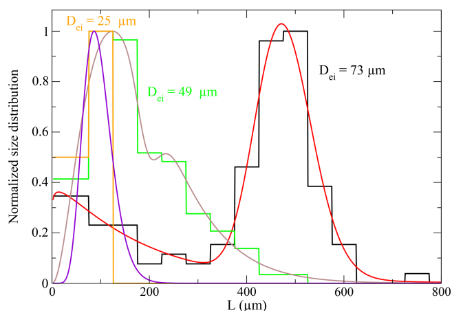
Figure 12. Three examples of PSDs normalized to the respective maxima measured by the INCAS KA (black, green and orange histograms) with the D_{ei} calculated assuming the habit distribution in Eq. (7) and the fitting functions (red, brown and violet curves).
