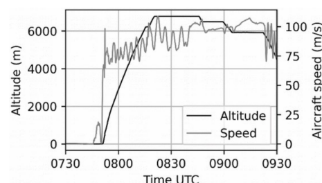
Figure 3. INCAS KA altitude and velocity as a function of time during 17 February 2023 flight. The INCAS KA was over ALOMAR between approximately 08:15–08:45 UTC as the aircraft contrail was clearly visible from the ground.
