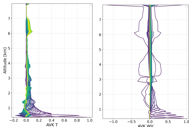
Figure 9. Left panel: vertical distribution of averaging kernels of temperature. Right panel: same for water vapour.
