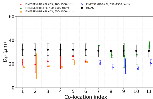
Figure 19. Comparison of the ice effective diameters derived from INCAS KA measurements (black dots) and those retrieved from FINESSSE spectra by using the whole spectral band between 400–1500 \text{cm}^{-1} (red and green solid triangles) and cutting the FIR portion below 650 \text{cm}^{-1} (orange and blue open triangles).
