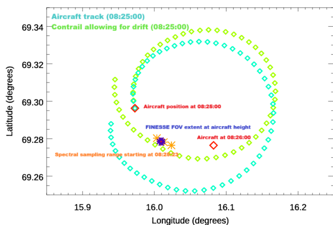
Figure 4. The turquoise diamonds map the aircraft track over the Alomar site up to 08:25:00 UTC, 30 s before the first overpass. We use photographs taken at this time and at 08:27:00 UTC, 30 s after the overpass to estimate the drift of the aircraft contrail, shown by the green diamonds. Extrapolating this to 08:26:30 UTC indicates that at the time of the overpass the contrail formed earlier in the flight, to the South-West, is directly over Alomar at the time of the overpass, this time also coincides with a distinct rise in radiance at 900\text{ cm}^{-1} , observed by FINESSE.
