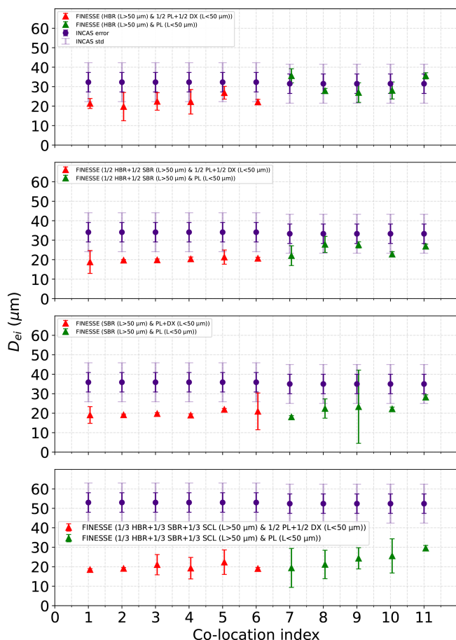
Figure 17. Top panel: comparison of the effective diameters calculated from INCAS KA data (violet dots) with the corresponding error and standard deviation between 08:19–09:00 UTC on 17 February 2023 and those retrieved from FINESSE (red and green triangles) between 08:25–08:38 UTC of the same day by assuming the habit distribution f_{1h} in Eq. (8). Second panel: same comparison but assuming f_{3h} from Eq. (10). Third panel: same comparison but assuming f_{2h} from Eq. (9). Bottom panel: same comparison but assuming f_{4h} from Eq. (11).
