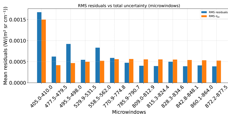
Figure 22. Histogram of the comparison between the root mean square (RMS) of the residuals (blue boxes) and the average noise over all scenarios (orange boxes, calculated Eq. 22) in the 13 selected microwindows.
