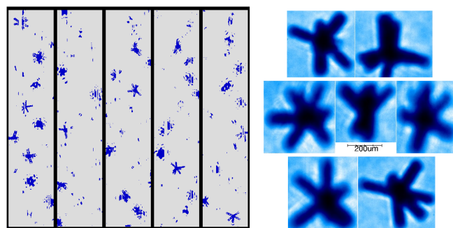
Figure 8. Examples of the ice crystals observed inside the cirrus layer by the INCAS KA on 17 February 2023 at 08:20 UTC. Images from the 10 \mu\text{m} -resolution channel of the 2D-S (left) where the width of each strip is 1280 \mu\text{m} and the CPI (right) are shown.
