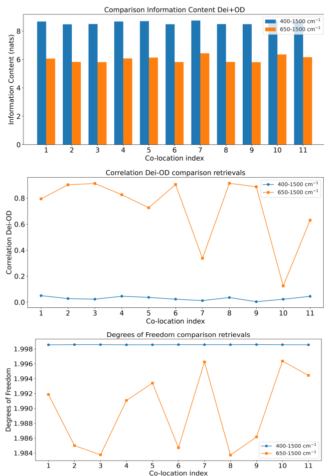
Figure 20. Upper panel: histogram of the information content (IC) after the first retrieval iteration in the full band and cutting the FIR. Middle panel: D_{\text{ei}} -OD correlations. Lower panel: cloud degrees of freedom (DOF).
