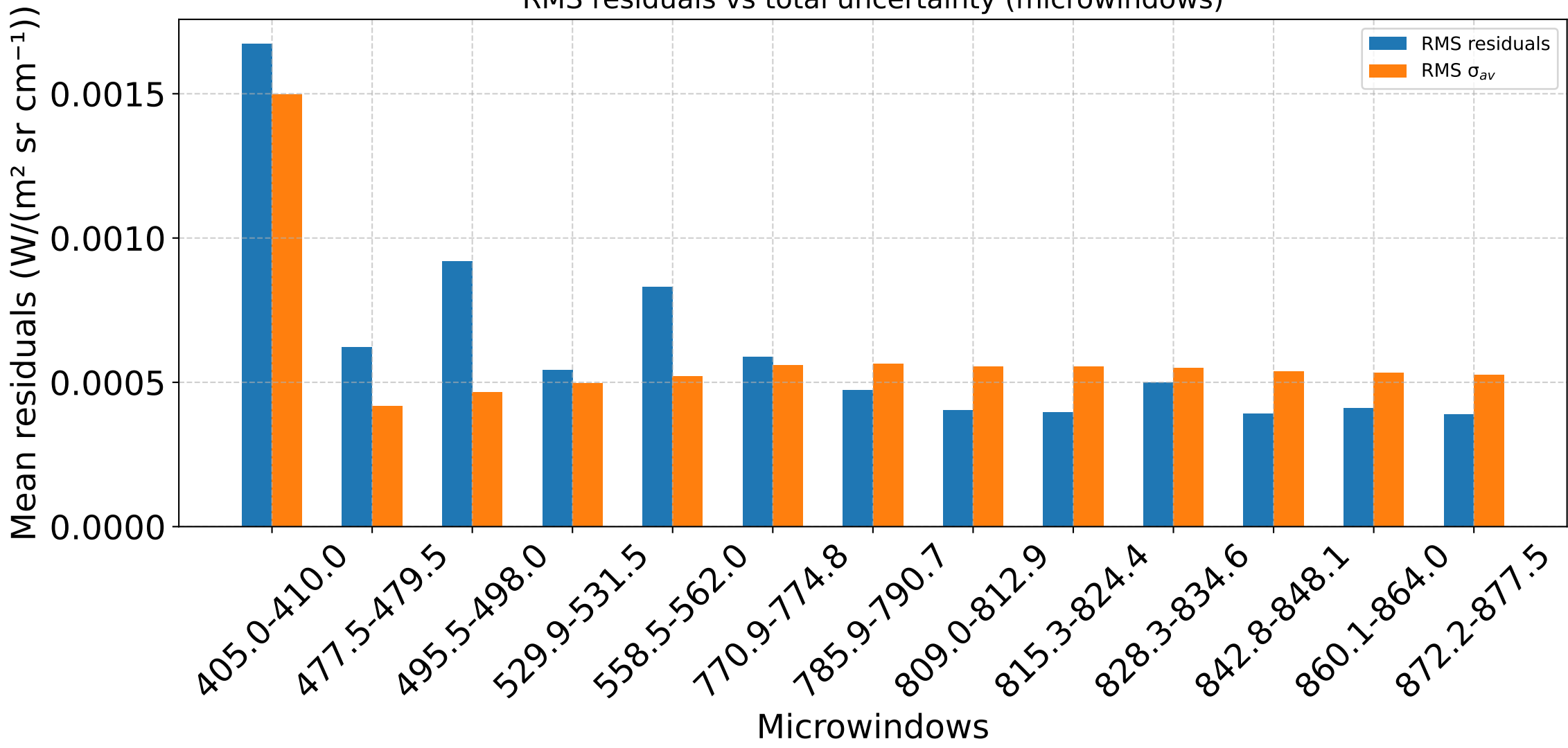
RMS residuals vs total uncertainty (microwindows)
