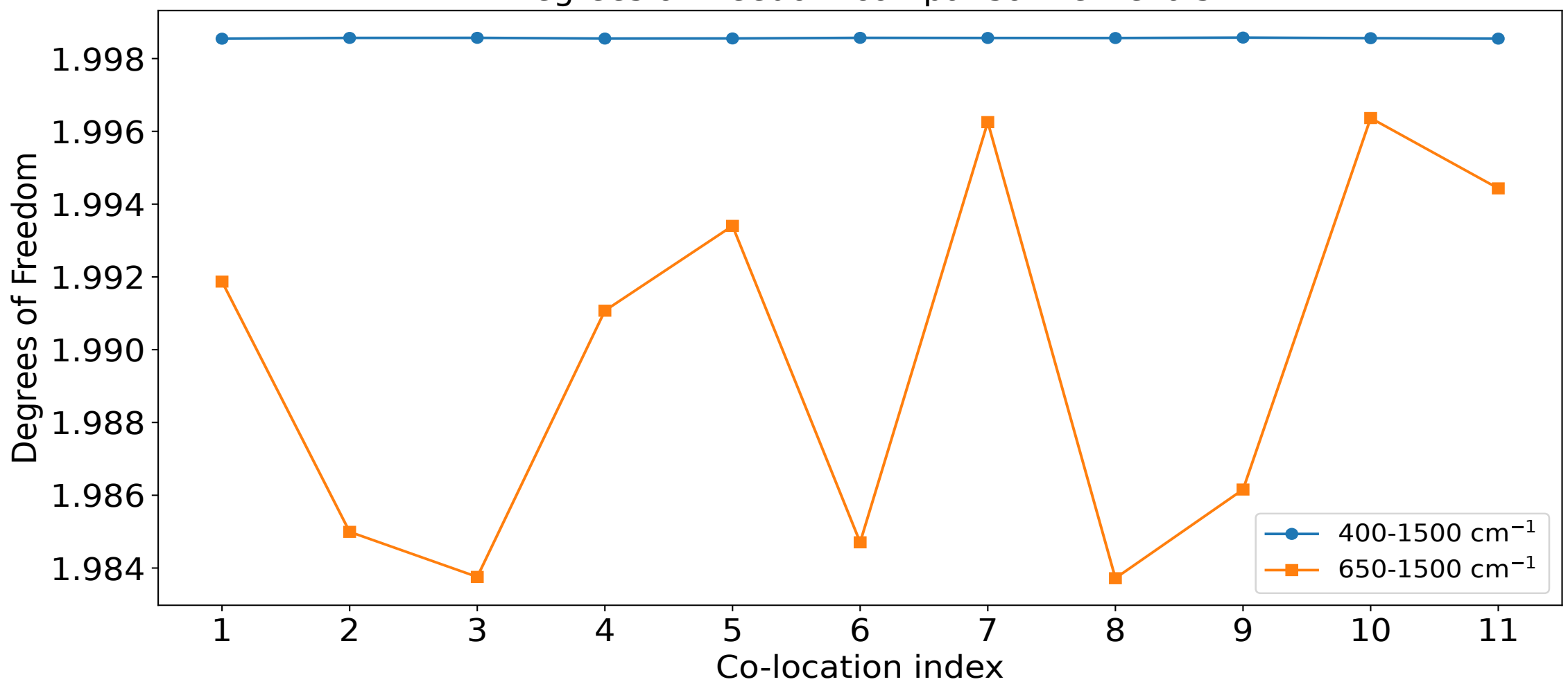
Degrees of Freedom comparison retrievals
