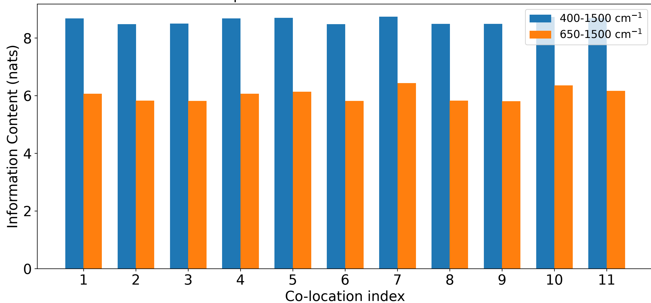
Comparison Information Content Dei+OD
