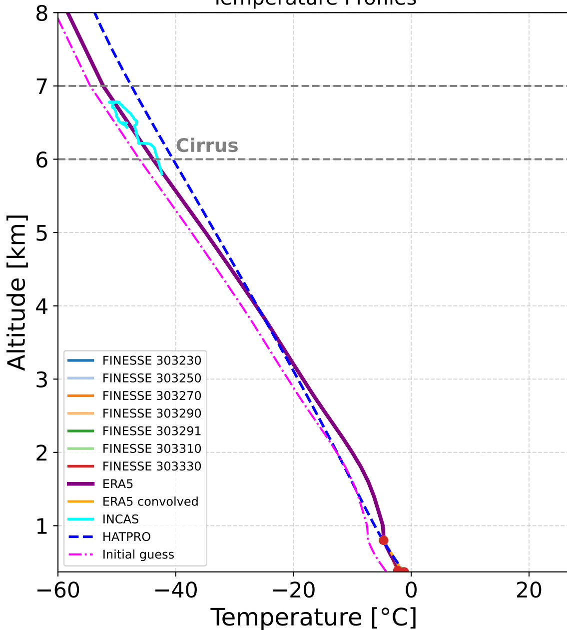
Temperature Profiles
