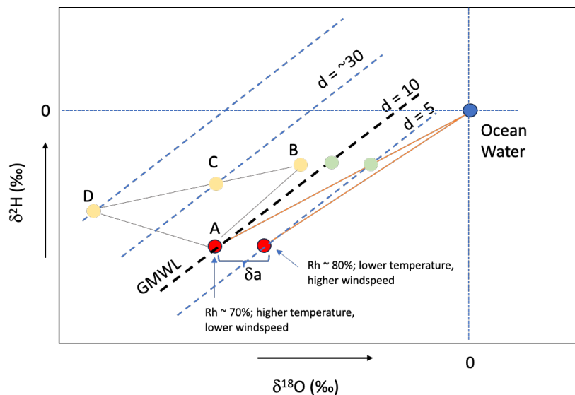
55 Fig. S1. Schematic diagram showing isotopic fractionation and d-excess change in evaporation and condensation (after Merlivat and Jouzel, 1979; Jouzel and Merlivat, 1984). The global meteoric water line (GMWL) is the global average isotopic composition of precipitation ( \delta^2\text{H} = 8\delta^{18}\text{O} + 10 ) with a d-excess (d) of +10. The isotopic composition of water vapor ( \delta a ) from the evaporation of ocean water (blue circle) would have different d-excess values (red circles) depending upon the 60 relative humidity, temperature and wind speed during evaporation. Condensation of water vapor in isotopic equilibrium would result in liquid water with the same d-excess as the vapor (green circles). Ice growth by deposition from a starting vapor at A would produce the solid phase (yellow circles) along the line B-D where the level of supersaturation with respect to ice increases towards D. Ice supersaturation is the ratio of ambient water pressure to vapor pressure at ice saturation. At B, the vapor pressure could be ~20% and at C ~100% greater than that at ice saturation. D represents pure diffusion where air flow is unaffected in the vicinity of ice crystals.
