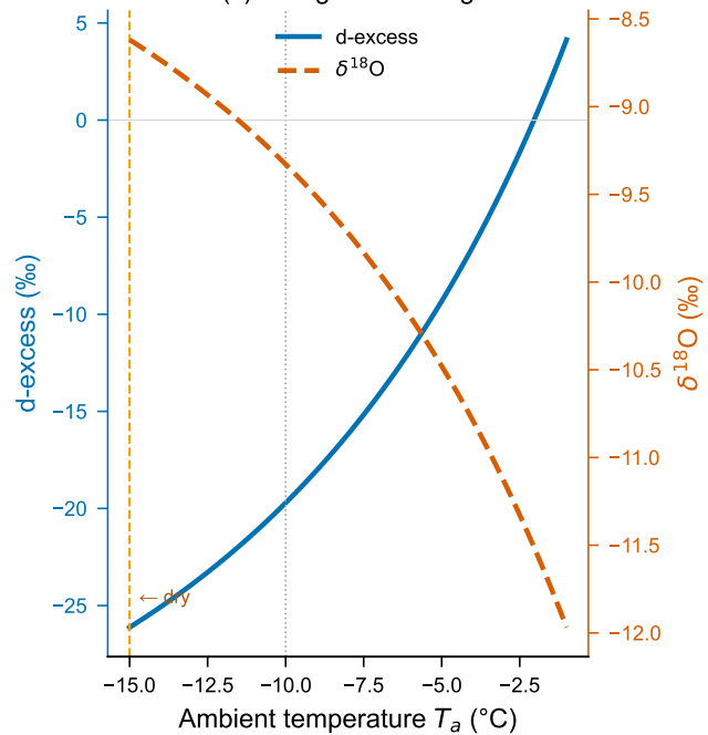
(c) Wet-growth riming
