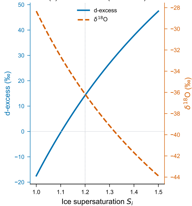
(b) Diamond dust ( T < -38^\circ\text{C} )
