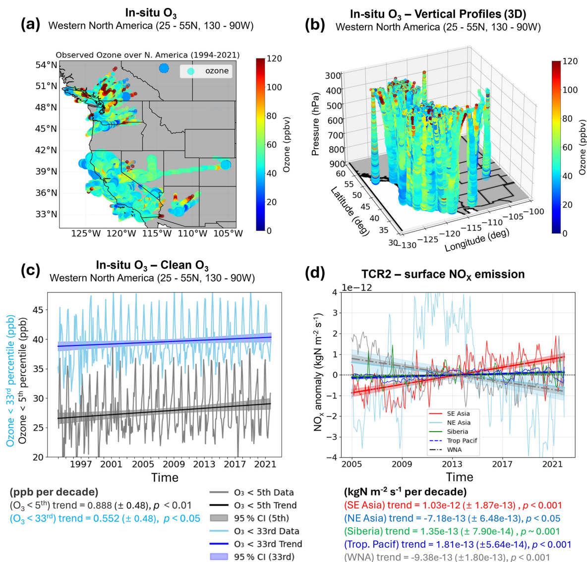
Figure 1. Trends and uncertainty in observed O_3 and chemical reanalysis NO_x emissions: (a, b) Map of 2-D horizontal and 3-D vertical distribution of observed O_3 (circle, ppb) over WNA used in this study (1994–2021). (c) Time series and trend (ppb per decade) of the low O_3 (<5th percentile (gray) and <33rd percentile (light blue)) from 1994 to 2021. (d) Time series of monthly anomalies and trends (ppb per decade) with uncertainty ( \pm 2 standard errors) in TCR-2 NO_x emissions over SE Asia (solid red), NE Asia (solid cyan), Siberia (solid green), the tropical Pacific (dashed blue), and WNA (gray dash-dotted) from 2005 to 2021. Shading in panels (c) and (d) denotes the 95 % confidence intervals of the trends.
