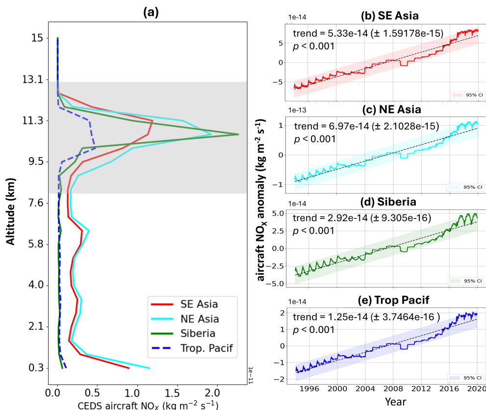
Figure 4. (a) Vertical profiles of CEDS aircraft NO x emission ( \text{kg m}^{-2} \text{s}^{-1} ) averaged over 1994–2019. (b–e) Time series of monthly anomaly and their linear trends (lines, \text{kg m}^{-2} \text{s}^{-1} per decade) with uncertainty ( \pm 2 standard errors) of the CEDS aircraft NO x emissions in the UTLS ( \sim 8 – 13 km) over the four source regions during 1994–2019. Shading in (b)–(e) denotes 95 % confidence intervals.
