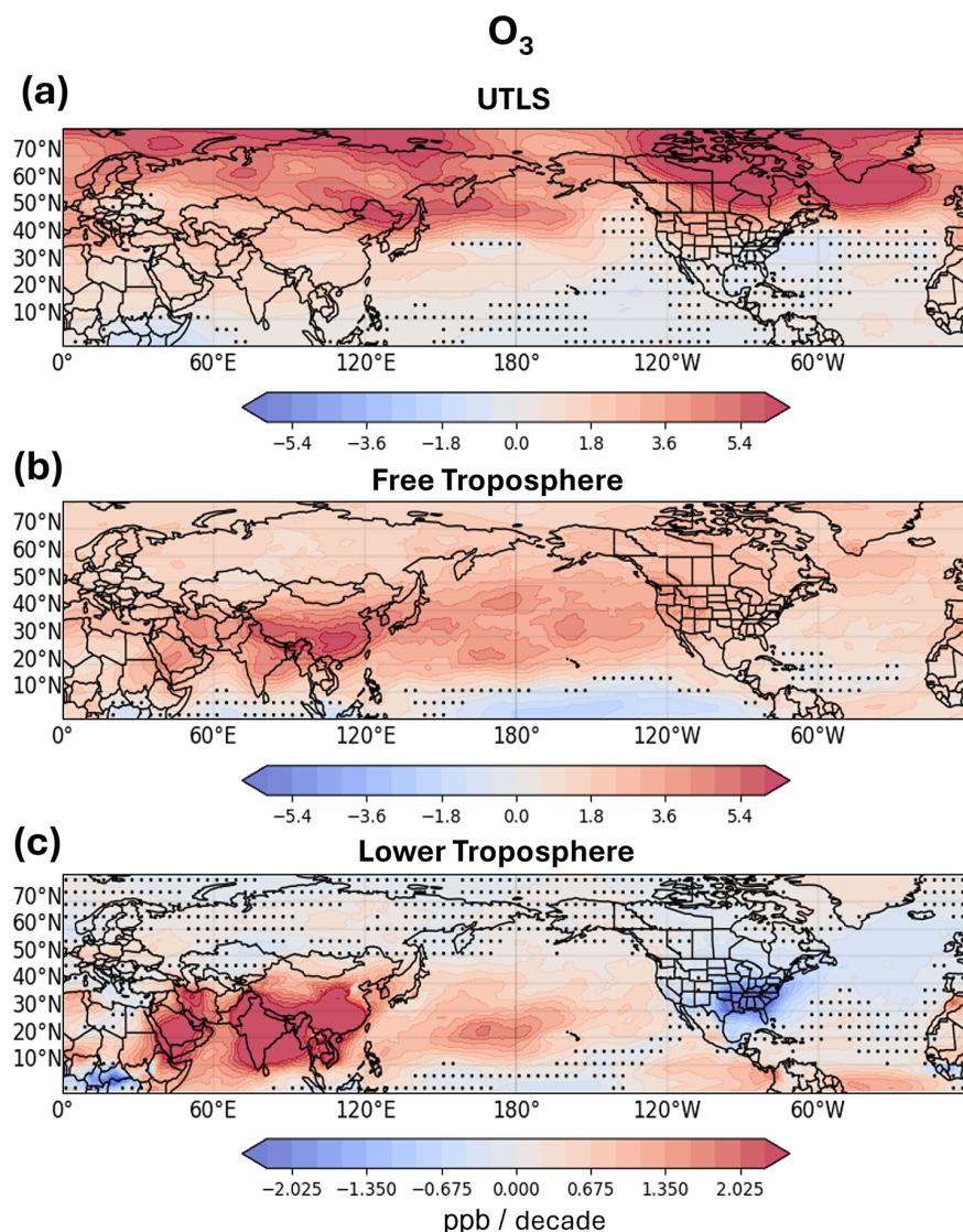
Figure 7. GMI O 3 trend (ppb per decade) in the (a) UTLS (244.88–176.93 hPa), (b) free troposphere (700–288.88 hPa), and (c) lower troposphere (725–985 hPa) calculated from 1994 and 2019. The dots on the maps represent the grid cells with a lower confidence value ( p -value \geq 0.05 ). The pressure shown here represents the midpoint of each GMI model level.
