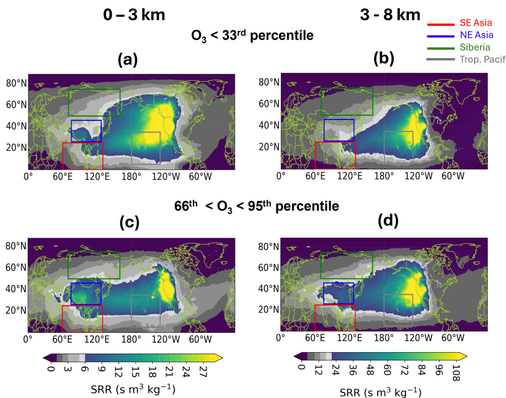
Figure 2. Maps of the source–receptor relationship (SRR): (top) low O_3 (< 33rd percentile), and (bottom) high O_3 (66th–95th percentile) over the WNA for (a) and (c), 0–3 km level and (b) and (d) 3–8 km. The red, blue, green, and gray boxes in (a) represent SE Asia (0–25° N, 60–130° E), NE Asia (26–46° N, 75–127° E), Siberia (50–75° N, 70–160° E), and Tropical Pacific (5–35° N, 180° E–130° W), respectively.
