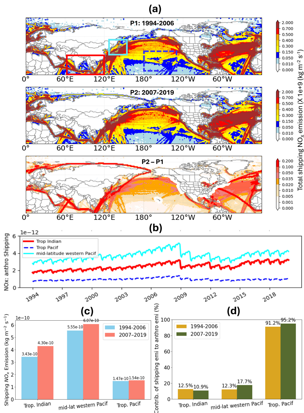
Figure 5. (a) Maps of CEDS anthropogenic shipping \text{NO}_x emissions ( \text{kg m}^{-2} \text{s}^{-1} ) for (top) P1 (1994–2006), (middle) P2 (2007–2019), and (bottom) the difference (P2 – P1). (b) Time series of shipping \text{NO}_x emissions for three source regions: the tropical Indian Ocean (0–30° N, 60–150° E; solid red), tropical Pacific (5–35° N, 180–130° W; dashed blue), and midlatitude western Pacific (30–55° N, 127–152° E; solid cyan). (c) Mean shipping emissions ( \text{kg m}^{-2} \text{s}^{-1} ) and (d) the contribution of shipping emissions to total anthropogenic emissions (%) over the three source regions during P1 and P2. The tropical Indian, tropical Pacific, and midlatitude western Pacific regions are indicated in red, blue, and cyan, respectively.
