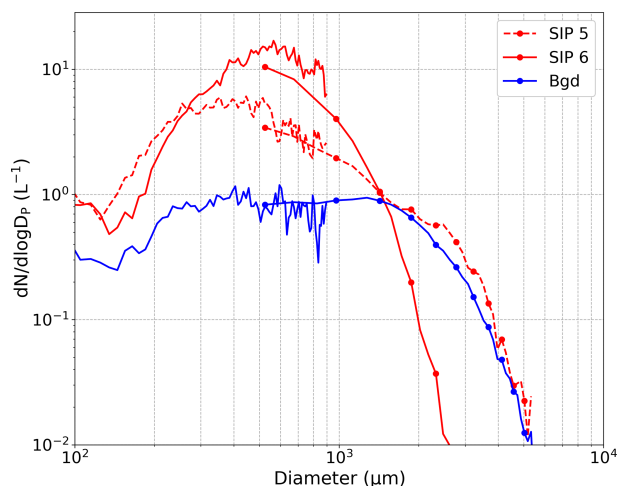
Figure 16. Mean composite (2D-S and HVPS) ice particle size distributions for SIP periods 5 (between 17:55:40 and 17:56:08 UTC) and 6 (between 19:34:40 and 19:35:10 UTC) (red lines) during flight C326 (28 October 2022), and all background ice periods (blue line). HVPS data shown by lines with markers for particle sizes > 600 \mu\text{m} .
