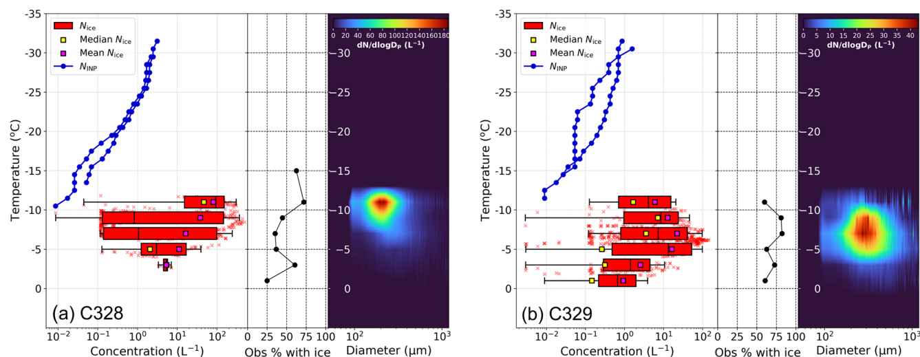
Figure 5. Measured total (2D-S + HVPS) ice crystal number concentrations ( N_{ice} ; red) as a function of local in-cloud temperature (1 Hz data) for flights (a) C328 (31 October 2022), and (b) C329 (1 November 2022). Boxplots (red) for N_{ice} above the instrument detection limit in 2 °C temperature bins are composed of centre lines, edges and whiskers representing the median, interquartile range (25th to 75th percentile) and nearest data points within 1.5 \times interquartile range of the lower and upper quartiles, respectively. Median N_{ice} (yellow squares) and mean N_{ice} (pink squares) are calculated from all data points, including N_{ice} below the instrument detection limit (i.e. where we have set N_{ice} to 0 \text{ L}^{-1} ). The percentage of ice concentration observations above 0 \text{ L}^{-1} within each temperature bin is also provided (black line). Measured INP concentrations ( N_{INP} ) derived from filter samples collected during both flights are shown in blue. Mean ice particle size distributions as a function of local in-cloud temperature for both flights are presented in the right panel of panels (a) and (b).
