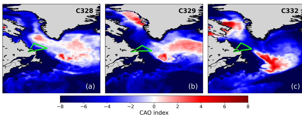
Figure B1. Mean CAO index values during M-Phase flights (a) C328, (b) C329, and (c) C332. Red and blue regions represent positive and negative index values, respectively. Flight tracks are overlaid (green lines).
