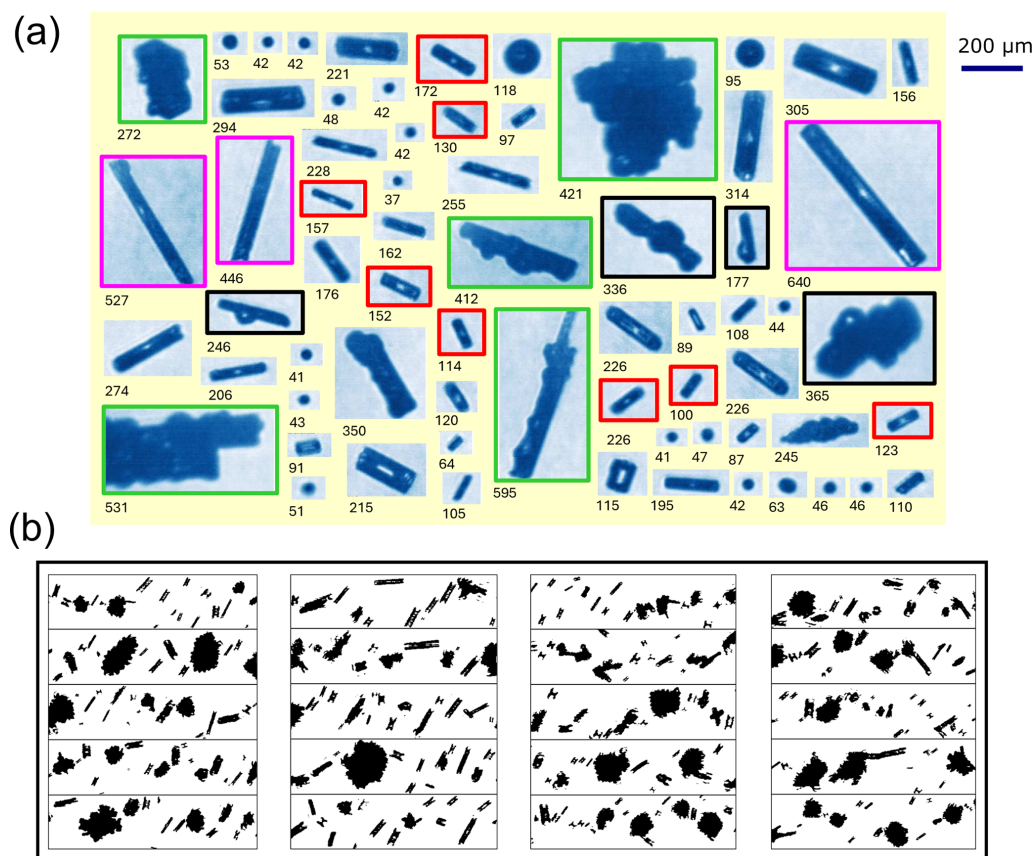
Figure 10. (a) Examples of cloud particles (ice crystals and liquid droplets) imaged with the CPI probe in SIP period 3 (between 13:26:45 and 13:29:18 UTC) during flight C329 (1 November 2022); subsets of small columnar ice of size < 200 \mu\text{m} (red frames), long columns (pink frames), rimed columns and plates (green frames), and columns with frozen droplets attached (black frames) are highlighted; numbers below images indicate the maximum dimension length ( D_p ) of each particle. (b) 2D-S images of highly irregular particles captured in SIP 3; the height of each strip corresponds to the 2D-S array width of 1280 \mu\text{m} .
