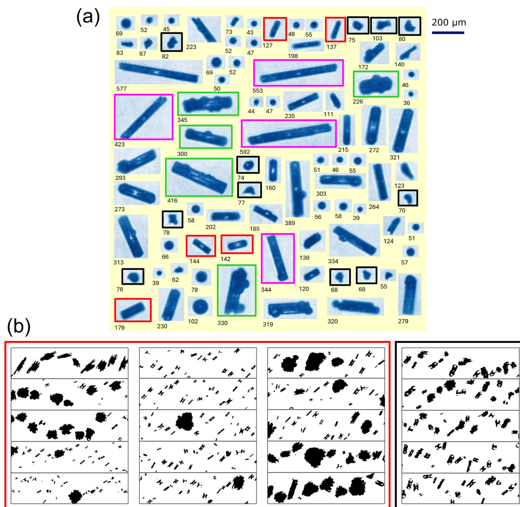
Figure 7. (a) Examples of cloud particles (ice crystals and liquid droplets) imaged with the CPI probe in SIP period 1 (between 16:27:00 and 16:29:45 UTC) during flight C328 (31 October 2022); subsets of small columnar ice of size < 200\ \mu\text{m} (red frames), long columns (pink frames), rimed columns (green frames), and possible frozen droplets and fragments of shattered droplets (black frames) are highlighted; numbers below images indicate the maximum dimension length ( D_p ) of each particle. (b) 2D-S images of highly irregular particles captured in SIP 1; the height of each strip corresponds to the 2D-S array width of 1280\ \mu\text{m} .
