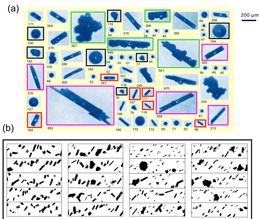
Figure C3. (a) Examples of cloud particles (ice crystals and liquid droplets) imaged with the CPI probe in SIP period 4 (between 14:11:25 and 14:13:03 UTC) during flight C329 (1 November 2022); subsets of small columnar ice of size < 200 \mu\text{m} (red frames), long columns (pink frames), rimed columns (green frames), and possible frozen droplets and fragments of shattered droplets (black frames) are highlighted; numbers below images indicate the maximum dimension length ( D_p ) of each particle. (b) 2D-S images of highly irregular particles captured in SIP 4; the height of each strip corresponds to the 2D-S array width of 1280 \mu\text{m} .
