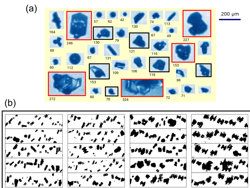
Figure C2. (a) Examples of cloud particles (ice crystals and liquid droplets) imaged with the CPI probe in SIP period 2 (between 16:19:45 and 16:20:30 UTC) during flight C328 (31 October 2022); subsets of plate-like crystals (red frames), and possible frozen droplets and fragments of shattered droplets (black frames) are highlighted; numbers below images indicate the maximum dimension length ( D_p ) of each particle. (b) 2D-S images of highly irregular particles captured in SIP 2; the height of each strip corresponds to the 2D-S array width of 1280 \mu\text{m} .
