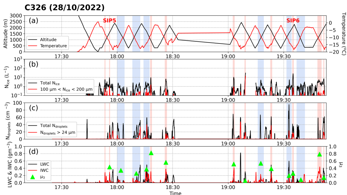
Figure 15. Time series of cloud microphysical properties (10 s averages) measured during flight C326 on 28 October 2022 (transit leg data excluded), including (a) temperature (red line) and altitude (black line), (b) total ice crystal number concentration ( N_{\text{ice}} ; black line) and concentration of ice particles with diameter > 100 and < 200 \mu\text{m} (red line), (c) total cloud droplet concentration ( N_{\text{droplets}} ; black line) and concentration of cloud droplets with diameter > 24 \mu\text{m} (red line), and (d) liquid water content (LWC) and ice water content (IWC). SIP and background ice regions are shaded in red and blue, respectively. Mean ice mass fraction ( \mu_3 ) values for SIP and background ice periods are also marked in panel (d) (green triangles).
