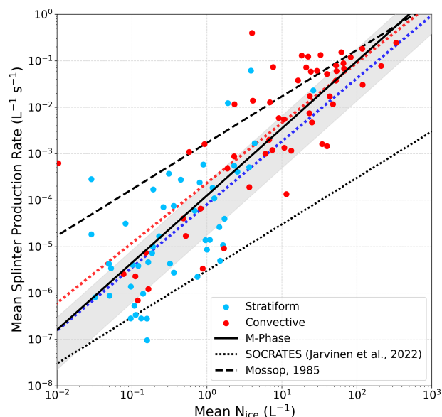
Figure 13. Mean splinter production rate ( \frac{dN_{\text{ice}}}{dt} ), calculated following Willis and Hallett (1991), as a function of mean measured ice particle concentrations for individual stratiform (blue) and convective (red) cloud segments with in-cloud temperatures within the H–M range of -3 to -8 °C. The solid black line represents the fit through the M-Phase data; the shaded region covers the area between fitting functions determined from maximum and minimum splinter production rates based on the overall relative uncertainty of \pm 86\% . The dashed and dotted black lines represent the relationships estimated by Mossop (1985c) (wintertime cumulus clouds over Australia) and Järvinen et al. (2022) (summertime CAO clouds over Southern Ocean), respectively.
