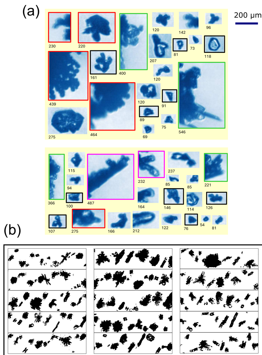
Figure 17. (a) Examples of cloud particles (ice crystals and liquid droplets) imaged with the CPI probe in two cloud segments (cloud top temperature \sim -18^\circ\text{C} ) during flight C326 (28 October 2022); subsets of large rimed crystals with fragile branches (red frames), aggregates (green frames), large crystals with plate-like extensions (pink frames), and small, irregular ice fragments (black frames) are highlighted; numbers below images indicate the maximum dimension length ( D_p ) of each particle. (b) 2D-S images of highly irregular particles captured in both cloud segments; the height of each strip corresponds to the 2D-S array width of 1280\ \mu\text{m} .
