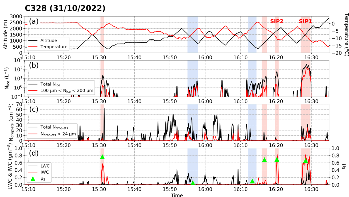
Figure 6. Time series of cloud microphysical properties (10 s averages) measured during flight C328 on 31 October 2022 (transit leg data excluded), including (a) temperature (red line) and altitude (black line), (b) total ice crystal number concentration ( N_{ice} ; black line) and concentration of ice particles with diameter > 100 and < 200 \mu\text{m} (red line), (c) total cloud droplet concentration ( N_{droplets} ; black line) and concentration of cloud droplets with diameter > 24 \mu\text{m} (red line), and (d) liquid water content (LWC) and ice water content (IWC). SIP and background ice regions are shaded in red and blue, respectively. Mean ice mass fraction ( \mu_3 ) values for SIP and background ice periods are also marked in panel (d) (green triangles).
