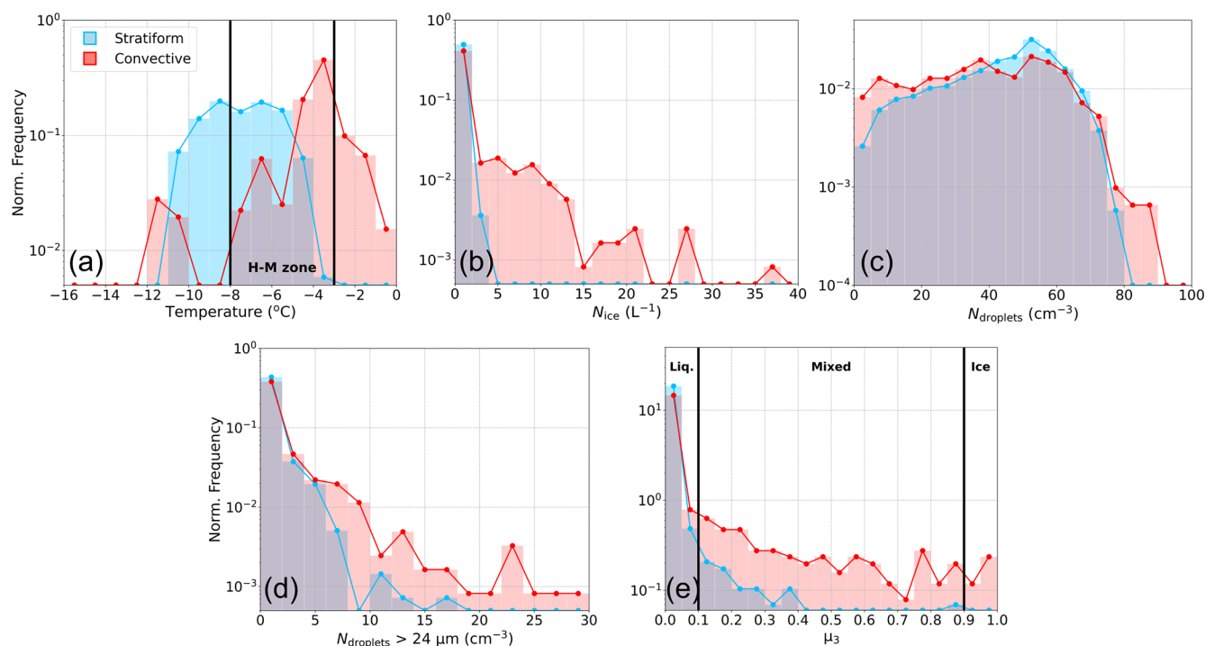
Figure C1. Relative frequency histograms of cloud microphysical properties (1 Hz data) measured within the stratiform (blue) and convective (red) regimes during flights C322 and C323, including (a) local in-cloud temperature (H–M zone marked), (b) ice crystal number concentration ( N_{ice} ), (c) total cloud droplet concentration ( N_{droplets} ), (d) concentration of cloud droplets with diameter > 24 \mu\text{m} , and (e) ice mass fraction ( \mu_3 ) with thresholds for liquid, mixed and ice phase cloud regions marked. Panels (b) to (e) only include data coinciding with in-cloud temperatures within H–M range ( -3 to -8^\circ\text{C} ). Data is normalised so that area under both stratiform and convective histograms integrates to 1.
