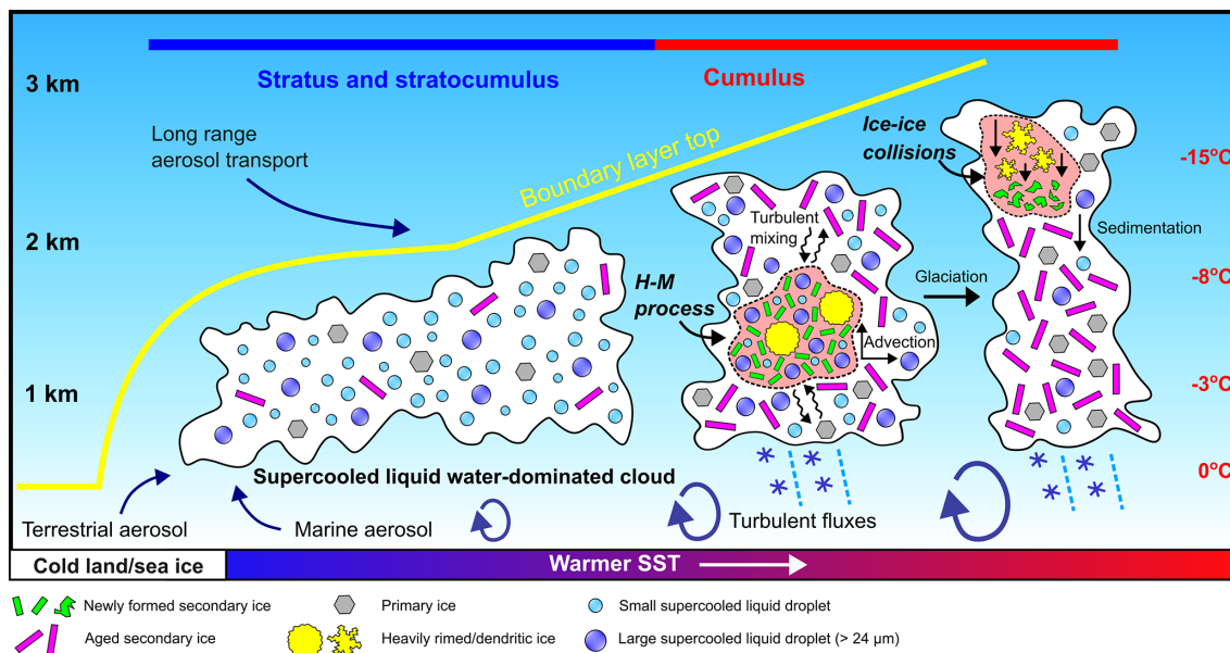
Figure 19. A schematic diagram summarising the evolution of cloud morphology and microphysical properties within CAOs, moving downwind from the stratiform to the convective regime, over the Labrador Sea during the M-Phase campaign. Red regions within cumulus cloud segments contain representations of the dominant SIP mechanisms, inferred from in-situ airborne observations.
