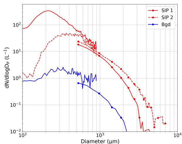
Figure 8. Mean composite (2D-S and HVPS) ice particle size distributions for SIP periods 1 (between 16:27:00 and 16:29:45 UTC) and 2 (between 16:19:45 and 16:20:30 UTC) (red lines) during flight C328 (31 October 2022), and two background ice periods (blue line). HVPS data shown by lines with markers for particle sizes > 600 \mu\text{m} .
