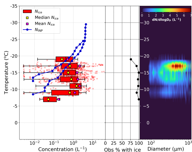
Figure 14. Measured total (2D-S + HVPS) ice crystal number concentrations ( N_{\text{ice}} ; red) as a function of local in-cloud temperature (1 Hz data) for flight C326 (28 October 2022). Boxplots (red) for N_{\text{ice}} above the instrument detection limit in 2 °C temperature bins are composed of centre lines, edges and whiskers representing the median, interquartile range (25th to 75th percentile) and nearest data points within 1.5 \times interquartile range of the lower and upper quartiles, respectively. Median N_{\text{ice}} (yellow squares) and mean N_{\text{ice}} (pink squares) are calculated from all data points, including N_{\text{ice}} below the instrument detection limit (i.e. where we have set N_{\text{ice}} to 0 \text{ L}^{-1} ). The percentage of ice concentration observations above 0 \text{ L}^{-1} within each temperature bin is also provided (black line). Measured INP concentrations ( N_{\text{INP}} ) derived from filter samples collected during flight C326 are shown in blue. Mean ice particle size distributions as a function of local in-cloud temperature are presented in the right panel.
