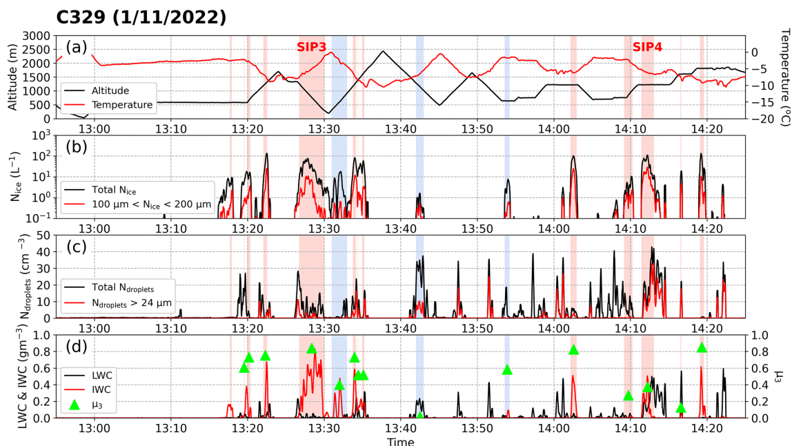
Figure 9. Time series of cloud microphysical properties (10 s averages) measured during flight C329 on 1 November 2022 (transit leg data excluded), including (a) local temperature (red line) and altitude (black line), (b) total ice crystal number concentration ( N_{\text{ice}} ; black line) and concentration of ice particles with diameter > 100 and < 200 \mu\text{m} (red line), (c) total cloud droplet concentration ( N_{\text{droplets}} ; black line) and concentration of cloud droplets with diameter > 24 \mu\text{m} (red line), and (d) liquid water content (LWC) and ice water content (IWC). SIP and background ice regions are shaded in red and blue, respectively. Mean ice mass fraction ( \mu_3 ) values for SIP and background ice periods are also marked in panel (d) (green triangles).
