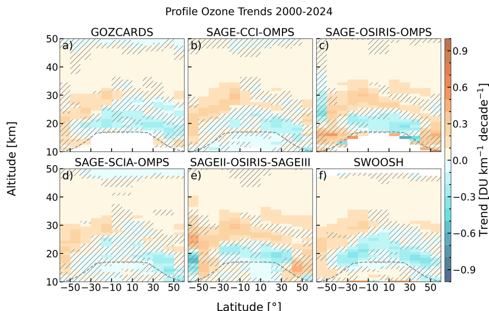
Figure 9. Profile ozone trends in \text{DU km}^{-1} per decade from 2000 to 2024 from the six merged ozone datasets as a function of latitude and altitude: (a) GOZCARDS, (b) SAGE-CCI-OMPS, (c) SAGE-OSIRIS-OMPS, (d) SAGE-SCIA-OMPS, (e) SAGEII-OSIRIS-SAGEIII, and (f) SWOOSH. Hatched areas indicate regions of no significance ( 2\sigma ). Dashed lines are the climatological thermal tropopause derived from ERA5.
