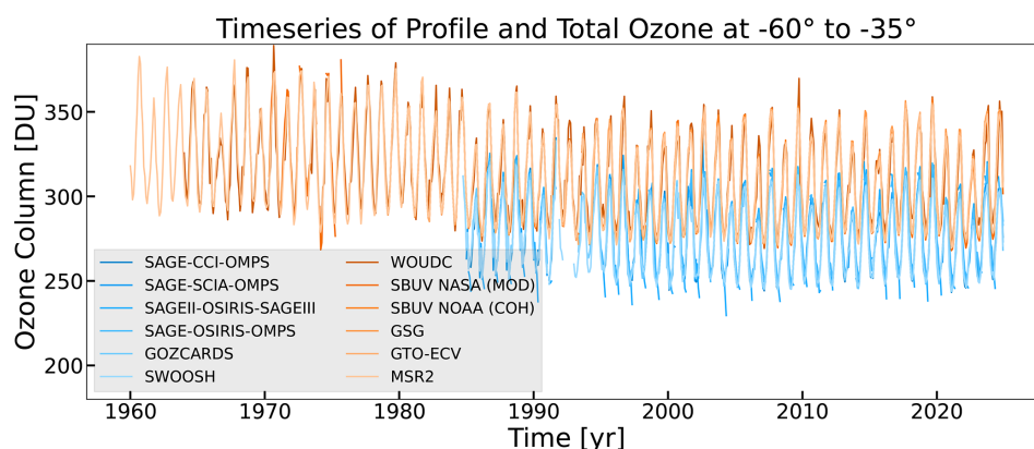
Figure 11. Observed zonal debiased mean stratospheric (blue) and total (orange) ozone columns in the 35 to 60° S latitude band.
