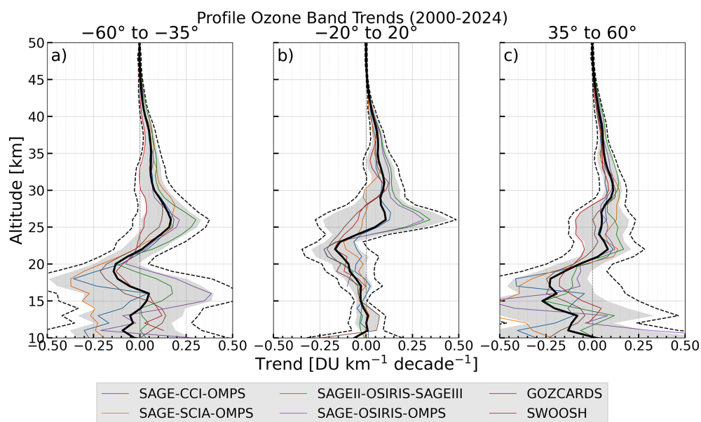
Figure A9. Ozone trends with the LOTUS Model from 2000 to 2024 in three distinct latitude bands ((a) 35–60° S, (b) 20° S–20° N, (c) 35–60° N) in DU km -1 per decade for the six merged ozone profile datasets: GOZCARDS, SAGE-CCI-OMPS, SAGE-OSIRIS-OMPS, SAGEII-OSIRIS-SAGEIII, SAGE-SCIA-OMPS, and SWOOSH. Shaded area indicates the 2 \sigma uncertainties, calculated using the LOTUS (Eq. 7) and the dashed line indicates the J-Distribution uncertainty (Eq. 9) of the mean trends (black line). Same as Fig. 10, but using the LOTUS setup in the MLR.
