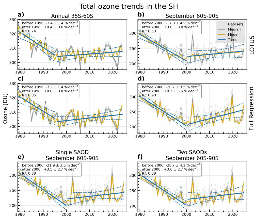
Figure 8. 35–60° S annual mean (a, c) and 60–90° S September (b, d, e, f) MLR results using the LOTUS setup (top row) and the full regression model (second row) applied to the total ozone median from six merged datasets. Different SAOD setups are shown for the September SH polar region: (e) single AOD proxy from 1979 to 2024, (f) two AOD proxies: from 1979 to 1989 and from 1990 to 2024 and (d) three AOD proxies: from 1979 to 1989 (El Chichon period), from 1990 to 1999 (Pinatubo period), and from 2000 to 2024 (HTHH and smaller eruption period). Thick grey line: median of observations; yellow line: MLR regression; thin grey lines: individual merged datasets; solid blue lines: trend lines before and after 2000; dashed blue lines: 2\sigma uncertainty of the trend lines.
