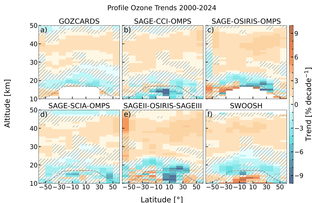
Figure A5. Profile ozone trends in % per decade from 2000 to 2024 using the LOTUS setup for the six profile ozone datasets (a) GOZCARDS, (b) SAGE-CCI-OMPS, (c) SAGE-OSIRIS-OMPS, (d) SAGE-SCIA-OMPS, (e) SAGEII-OSIRIS-SAGEIII, and (f) SWOOSH. Hatches indicate regions of no significance ( 2\sigma ). Same as Fig. 9, but using the LOTUS setup in the MLR and trend units of % per decade.
