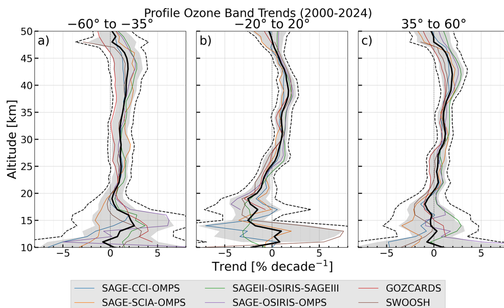
Figure A7. Ozone trends with the Full Regression Model from 2000 to 2024 in three distinct latitude bands ((a) 35–60° S, (b) 20° S–20° N, (c) 35–60° N) in % per decade for the six merged ozone profile datasets: GOZCARDS, SAGE-CCI-OMPS, SAGE-OSIRIS-OMPS, SAGEII-OSIRIS-SAGEIII, SAGE-SCIA-OMPS, and SWOOSH. Shaded area indicates the 2 \sigma uncertainties, calculated using the LOTUS (Eq. 7) and the dashed line indicates the J-Distribution uncertainty (Eq. 9) of the mean trends (black line). Same as Fig. 10, but trends in units of % per decade.
