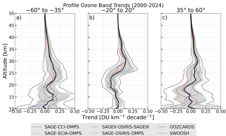
Figure 10. Ozone trends from 2000 to 2024 in three latitude bands ((a) 35^{\circ} – 60^{\circ} S, (b) 20^{\circ} S– 20^{\circ} N, (c) 35^{\circ} – 60^{\circ} N) in \text{DU km}^{-1} per decade for the six merged ozone profile datasets: GOZCARDS, SAGE-CCI-OMPS, SAGE-OSIRIS-OMPS, SAGEII-OSIRIS-SAGEIII, SAGE-SCIA-OMPS, and SWOOSH. Shaded area indicates the 2\sigma uncertainties of the mean trends (black line), calculated using the LOTUS uncertainty estimate described in Eq. (7) and the dashed line indicates the J-Distribution uncertainty described by Eq. (9).
