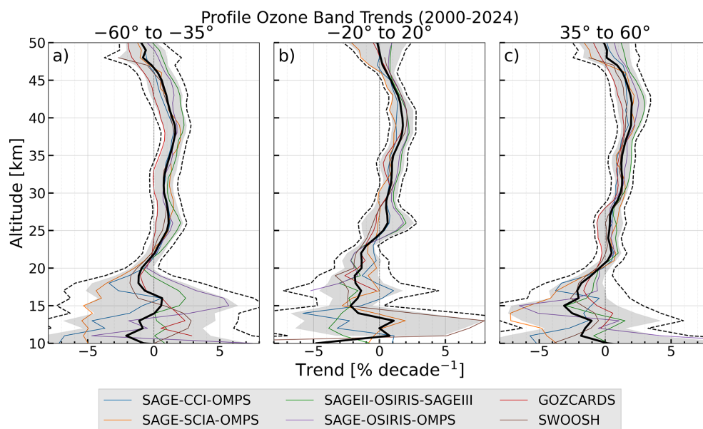
Figure A8. Ozone trends with the LOTUS Model from 2000 to 2024 in three distinct latitude bands ((a) 35–60° S, (b) 20° S–20° N, (c) 35–60° N) in % per decade for the six merged ozone profile datasets: GOZCARDS, SAGE-CCI-OMPS, SAGE-OSIRIS-OMPS, SAGEII-OSIRIS-SAGEIII, SAGE-SCIA-OMPS, and SWOOSH. Shaded area indicates the 2 \sigma uncertainties, calculated using the LOTUS (Eq. 7) and the dashed line indicates the J-Distribution uncertainty (Eq. 9) of the mean trends (black line). Same as Fig. 10, but using the LOTUS setup in the MLR and trend units of % per decade.
