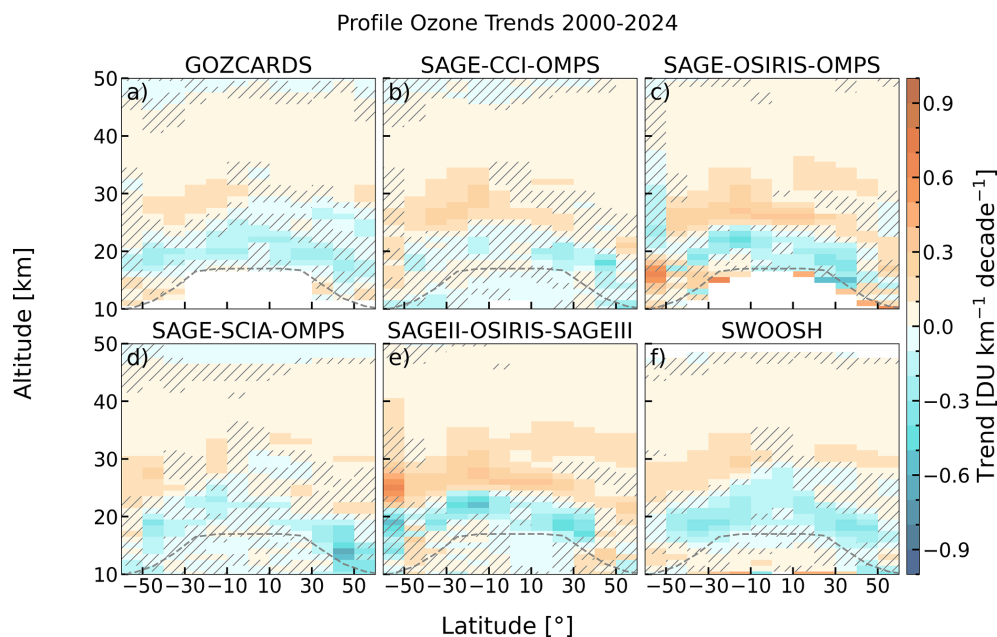
Figure A4. Profile ozone trends (LOTUS model) in \text{DU km}^{-1} per decade from 2000 to 2024 for the six profile ozone datasets (a) GOZCARDS, (b) SAGE-CCI-OMPS, (c) SAGE-OSIRIS-OMPS, (d) SAGE-SCIA-OMPS, (e) SAGEII-OSIRIS-SAGEIII, and (f) SWOOSH. Hatches indicate regions of no significance ( 2\sigma ). Same as Fig. 9, but using the LOTUS setup in the MLR.
