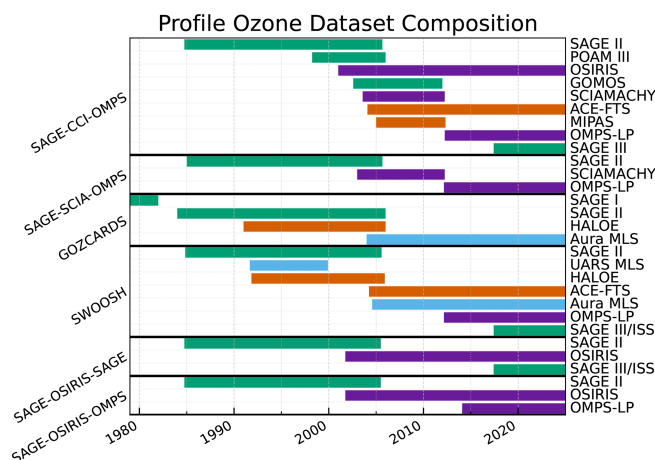
Figure 1. Satellite missions contributing to each of the six merged ozone profile datasets. The instruments shown in light blue measure in the microwave region, those shown in green measure in the UV/visible region, those shown in orange measure in the thermal infrared region, and those shown in violet measure UV/visible limb scatter.
