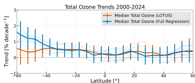
Figure A2. Total ozone trends in % per decade from 2000 to 2024 for the six total ozone datasets WOUDC, SBUV NASA (MOD), SBUV NOAA (COH), GSG, GTO-ECV, and MSR2 (thin lines) and the median and its 2\sigma uncertainty (thick line and error bars). Shown in blue are the MLR results with additional dynamical and SAOD proxies and in orange the LOTUS model setup. Same as Fig. 7, but with ozone trend units of % per decade.
