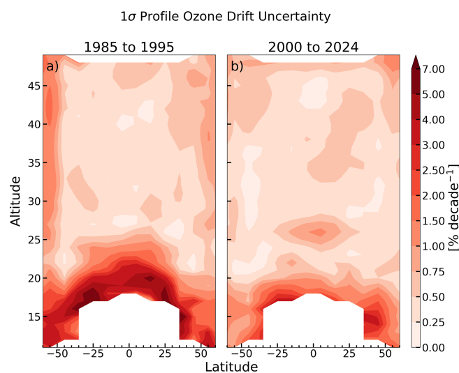
Figure 4. Standard deviation (1σ) of the drifts relative to the multi-instrument mean derived from GOZCARDS, SAGE-CCI-OMPS, SAGE-SCIA-OMPS, SAGE-OSIRIS-OMPS, SAGEII-OSIRIS-SAGEIII and SWOOSH profile data for the periods (a) 1985 to 1995 and (b) 2000 to 2024 as a function of latitude and altitude.
