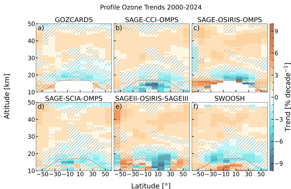
Figure A3. Profile ozone trends in % per decade from 2000 to 2024 for the six profile ozone datasets (a) GOZCARDS, (b) SAGE-CCI-OMPS, (c) SAGE-OSIRIS-OMPS, (d) SAGE-SCIA-OMPS, (e) SAGEII-OSIRIS-SAGEIII, and (f) SWOOSH. Hatches indicate regions of no significance ( 2\sigma ). Same as Fig. 9, but in units of % per decade.
