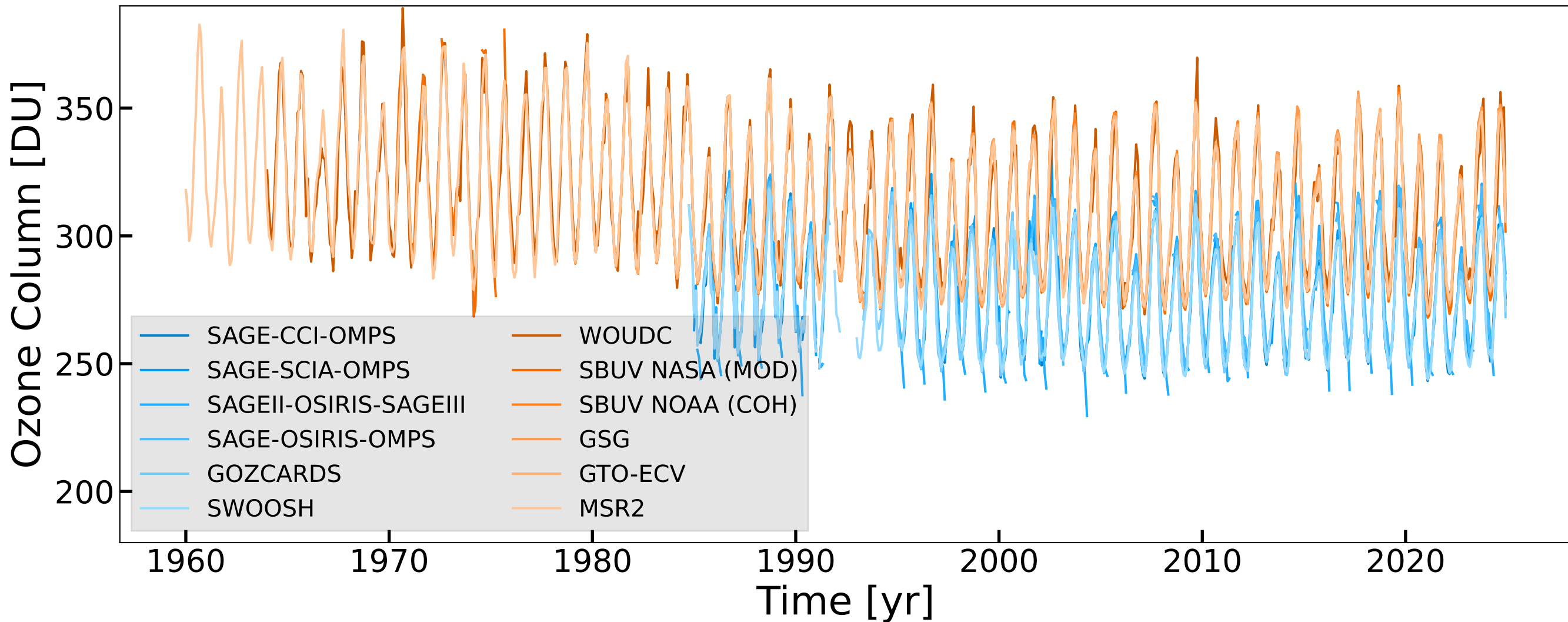
Timeseries of Profile and Total Ozone at -60^{\circ} to -35^{\circ}
