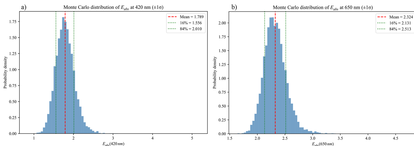
Figure 7. Probability distribution of E_{\text{abs}} at 420 nm (a) and 650 nm (b) on 19 February 2023. The \pm 1\sigma range (68 % probability) is used to represent uncertainty.
