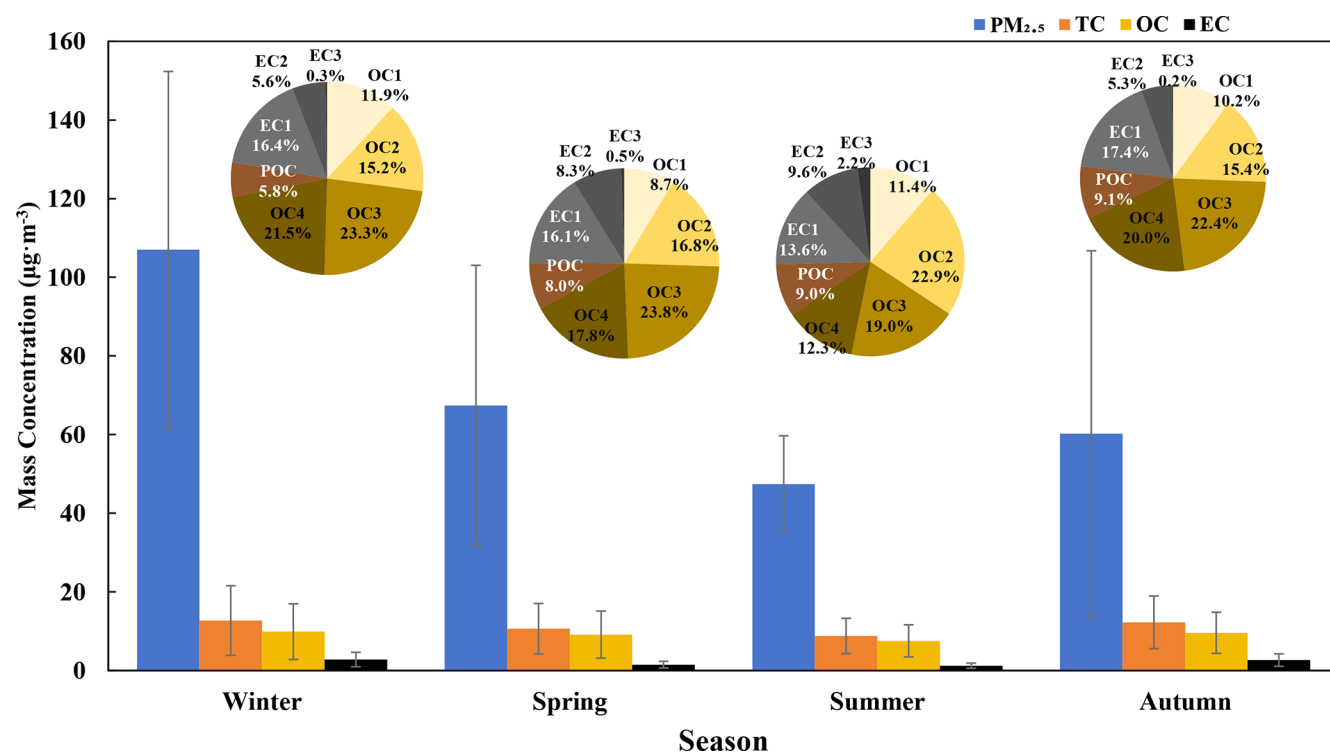
Figure 2. Aerosol loadings and compositions in 2023.
