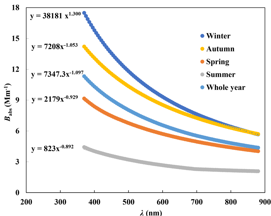
Figure 3. Total absorption of coated aerosol.
