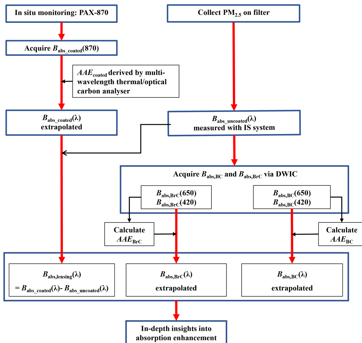
Figure 1. Methodological architecture. Note: The \lambda ranges from 370 to 880 nm.
