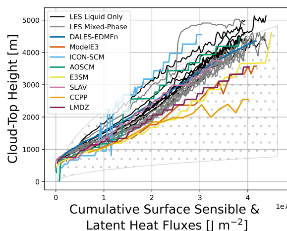
Figure 9. Relationship between cumulative surface heat (sensible and latent) fluxes and cloud-top height. LES Liquid Only and LES Mixed-Phase simulations are shown in the black and gray lines respectively, with each line representing results from a single model, while the SCMs are colored according to the legend. Stippling in the background shows theoretical expectations assuming surface-only forcing (Eq. 11.2.2f in Stull, 1988) under weakest and strongest conditions.
