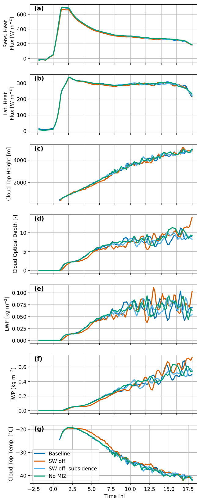
Figure C1. DHARMA LES output using various physics options.
