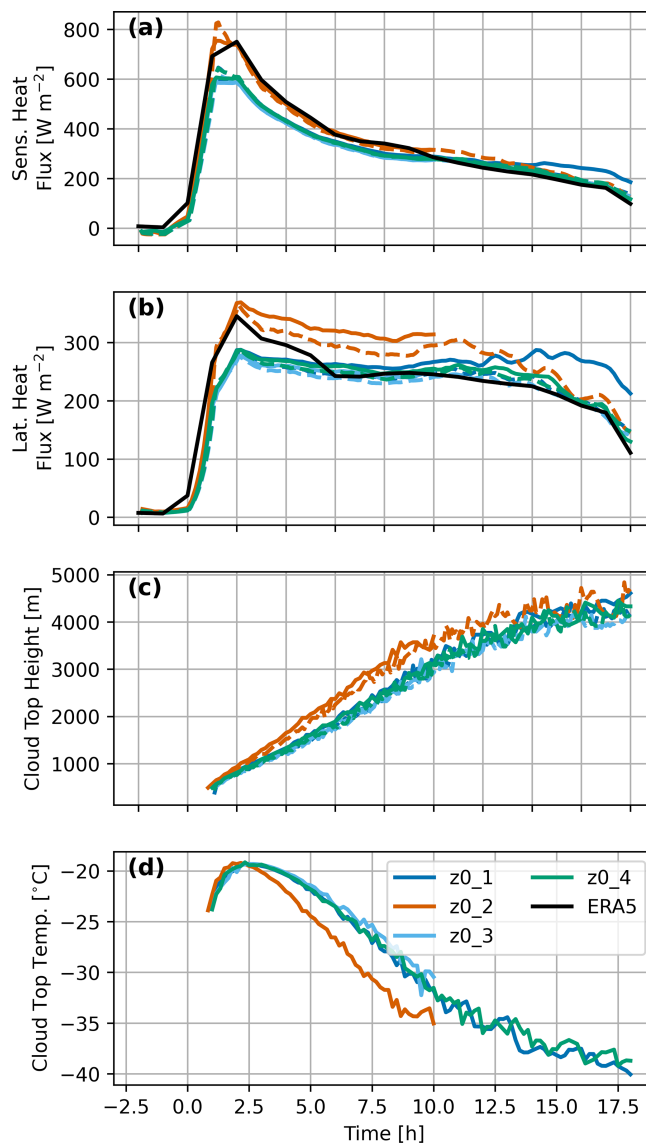
Figure B1. LES output using various surface roughness length configurations for DHARMA (solid lines) and WRF (dashed lines).
