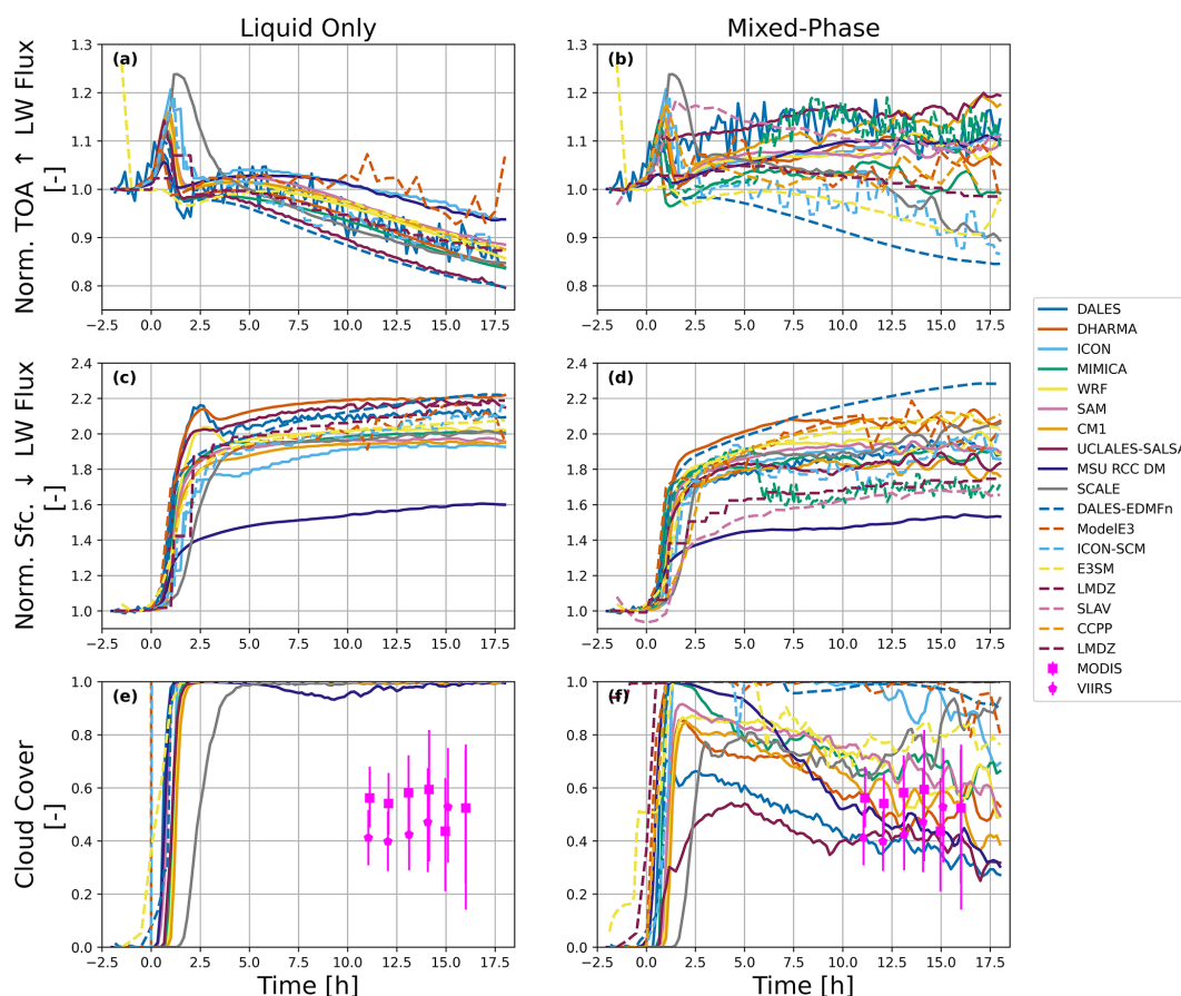
Figure 11. As in Fig. 10, except showing only model results that are normalized by the pre-cloud ( t = -1 h) values. In the bottom-most row, we also show the modeled cloud cover together with observational targets, inferred from satellites carrying the MODIS and VIIRS instruments. Identical to LES, cloud cover is computed as the portion of pixels with a cloud optical depth greater than 2.0.
