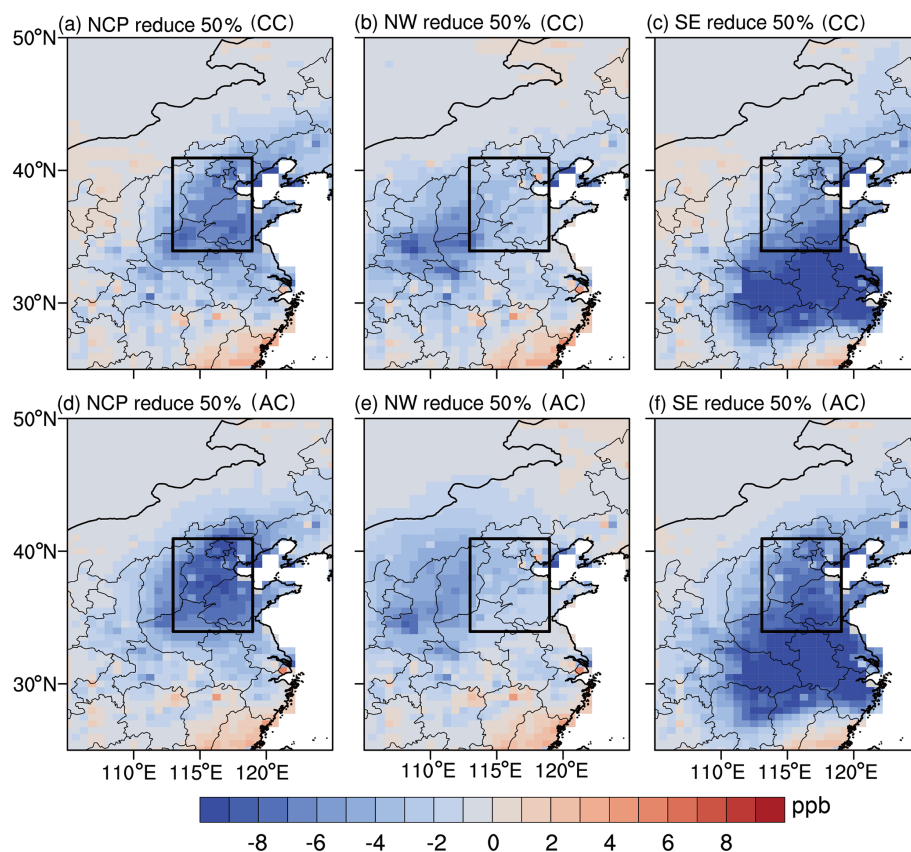
Figure 8. Response of MDA8 ozone concentration to 50 % reductions in both \text{NO}_x and VOCs emissions in the (a, d) NCP, (b, e) NW, and (c, f) SE regions under cyclonic-like circulation (upper panel) and anticyclonic circulation (lower panel). The black rectangles denote the NCP. The NW and SE regions are indicated in Fig. S1.
