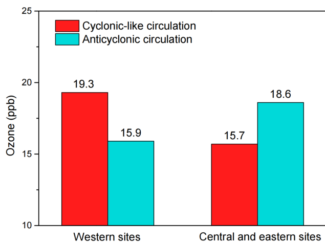
Figure 5. Ozone concentration anomalies at two types of stations under cyclonic-like and anticyclonic circulations relative to the summer mean during 2017–2022. The western sites are located along the leeward foothills of the Taihang Mountains, including XT, HD, AY, HB, XX and ZZ. The central and eastern sites include BJ, BD, TJ, CZ, HS, DZ, BZ, JN and ZB, which are situated over the central and eastern plains. The locations of these stations are shown in Fig. 1.
