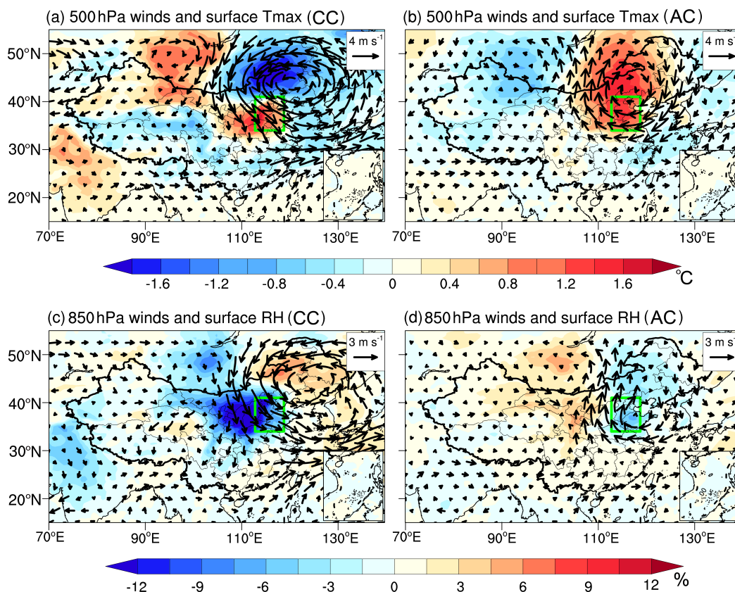
Figure 2. Spatial patterns of cyclonic-like circulation (CC, left) and anticyclonic circulation (AC, right) associated with ozone pollution days during the summers of 2017–2022. (a, b) Anomalous 500 hPa winds (vectors) and surface maximum temperature (filled colors) under CC and AC conditions. (c, d) Anomalous 850 hPa winds (vectors) and surface relative humidity (filled colors) under CC and AC conditions. Anomalies are calculated by subtracting the corresponding multi-year mean for June, July, and August, respectively. The green rectangles denote the NCP.
