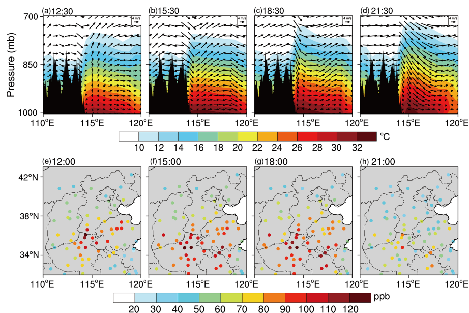
Figure 6. Vertical cross-sections of temperature and wind vectors along 37° N from 110 to 120° E (upper panel) and spatial pattern of surface ozone concentration (lower panel) on 5 June 2022 at (a, e) 12:30 and 12:00, (b, f) 15:30 and 15:00, (c, g) 18:30 and 18:00, (d, h) 21:30 and 21:00 (time zone is BJT = UTC+8). The vertical cross-sections of temperature and wind vectors are obtained from MERRA-2 data, while the surface O 3 concentrations are from hourly observations, with a 30 min time offset between the two datasets.
