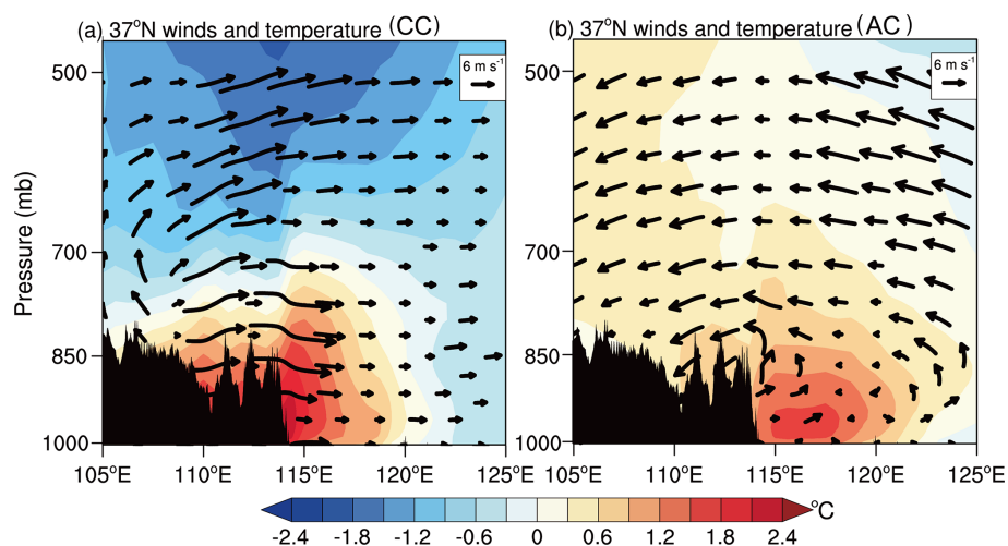
Figure 3. Vertical cross-sections of anomalous temperature and wind vectors along 37° N from 105 to 125° E under (a) cyclonic-like circulation and (b) anticyclonic circulation. The vertical wind component is multiplied by a factor of 300 when plotting the wind vector fields. Anomalies are calculated by subtracting the corresponding multi-year mean for June, July, and August, respectively.
