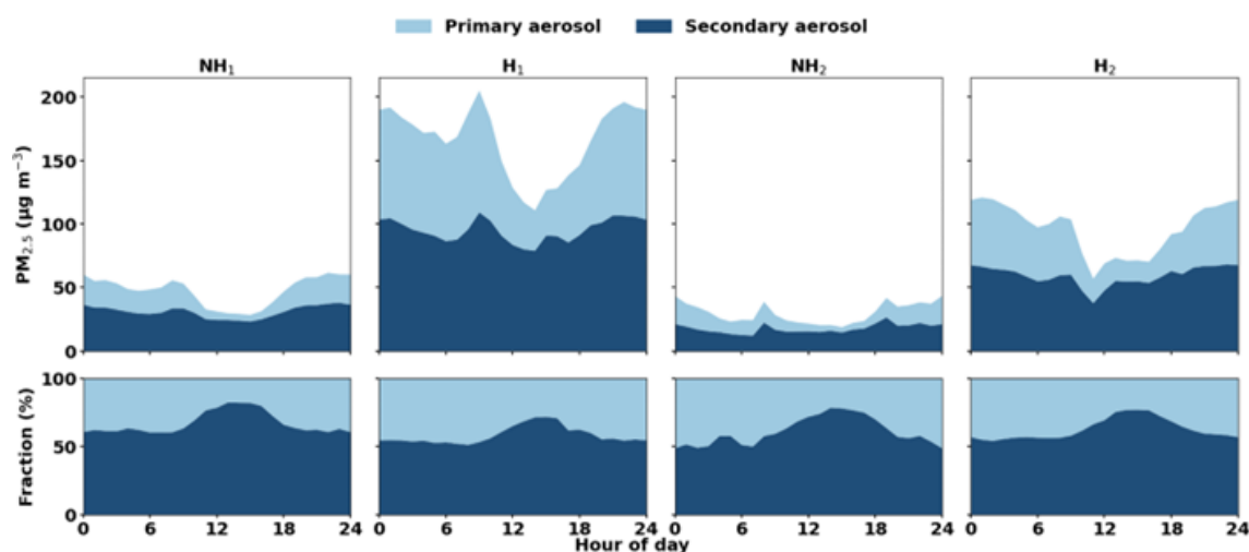
Figure 7. Average diurnal variation of mass concentrations and mass fractions of primary and secondary C-PM 2.5 by different haze periods. Data is for the full period from 25 October to 15 November 2023.
