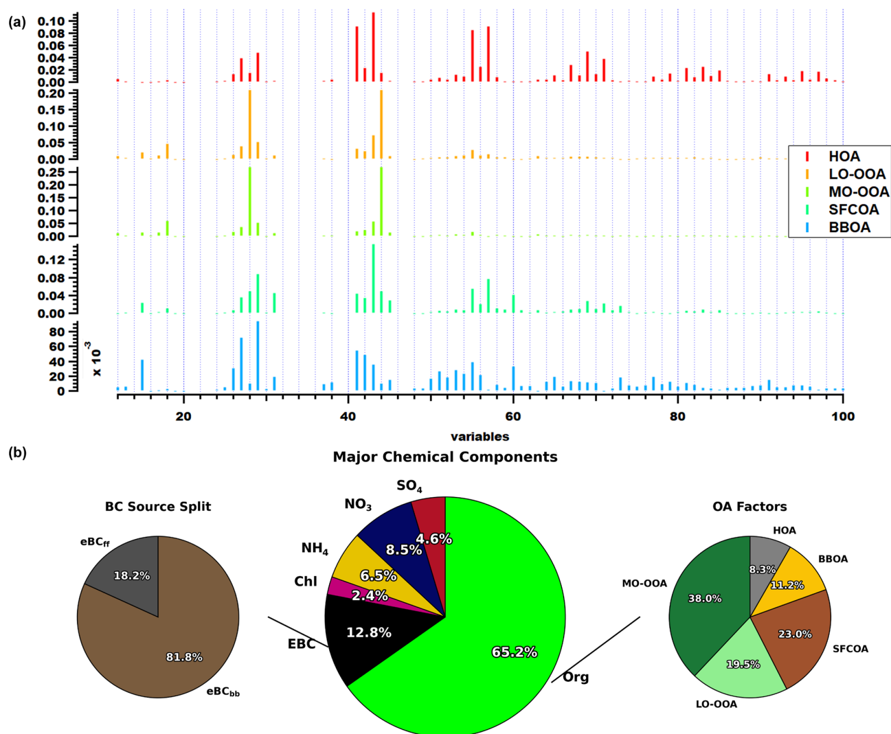
Figure 2. (a) Mass spectra of the OA factors (HOA, LO-OOA, MO-OOA, SFCOA and BBOA) resolved by PMF and, (b) Species contribution to C-PM 2.5 (NH 4 + , SO 4 2- , NO 3 - , Org, Cl - and BC) (center pie chart), Relative contribution of OA factors to total OA (right pie chart) and Relative contribution of BC factors (left pie chart).
