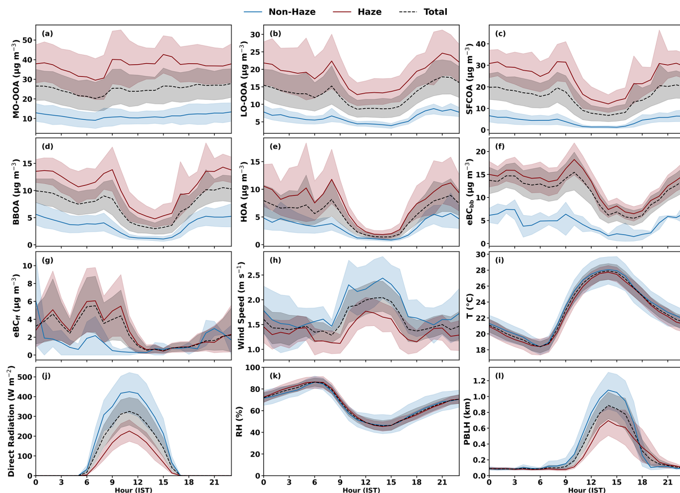
Figure 5. Diurnal variations of PMF factors: HOA, LO-OOA, MO-OOA, SFCOA and BBOA; 2 resolved BC factors: eBC bb and eBC fr ; meteorological parameters: Wind Speed, Temperature, Direct Radiation, Relative Humidity, PBLH during Haze (H1 + H2), Non-Haze (NH1 + NH2) and study period (Total) from 25 October to 15 November 2023.
