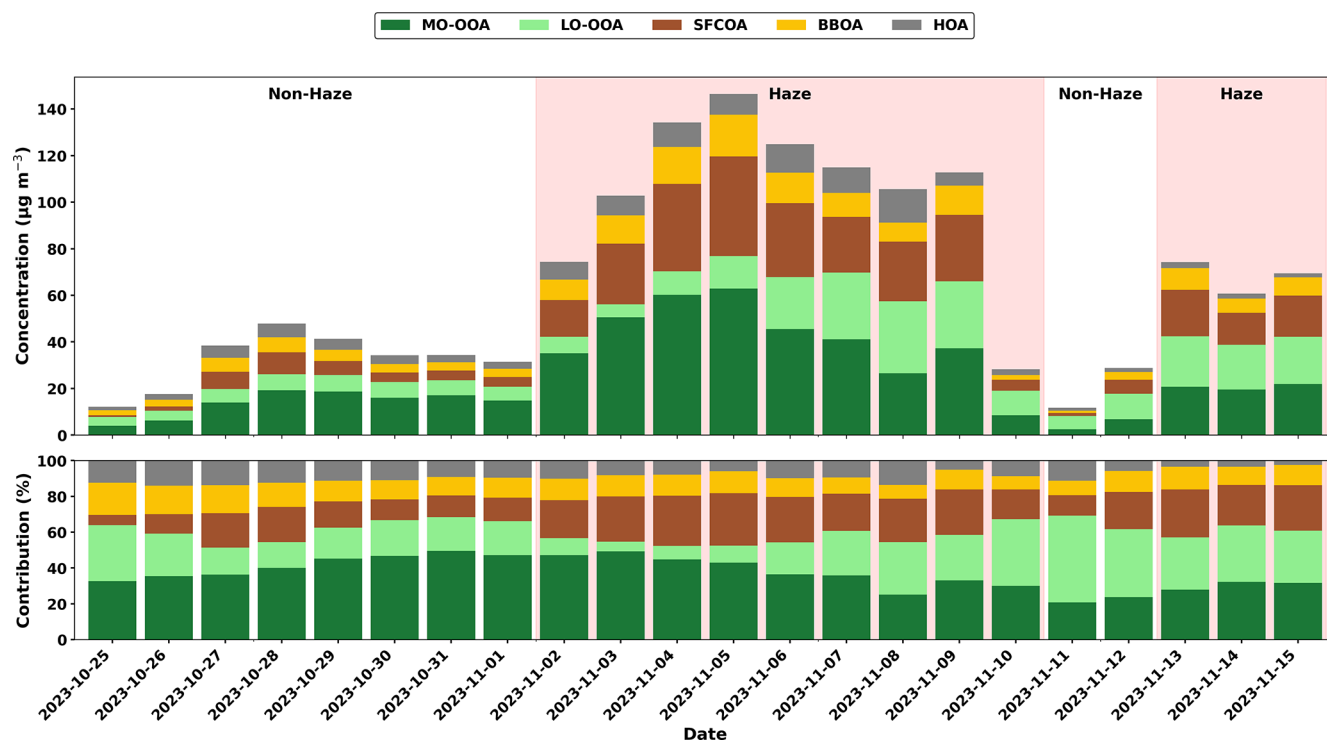
Figure 4. Daily organic aerosol (OA) source contributions during haze and non-haze periods from 25 October to 15 November 2023. The upper panel shows absolute concentrations ( \mu\text{g m}^{-3} ) of OA factors, including low-volatility oxygenated OA (MO-OOA), semi-volatile oxygenated OA (LO-OOA), solid fuel combustion OA (SFCOA), biomass burning OA (BBOA), and hydrocarbon-like OA (HOA). The lower panel presents the corresponding relative contributions (%) of each OA factor to total OA. Shaded regions indicate haze periods, while unshaded regions represent non-haze conditions.
