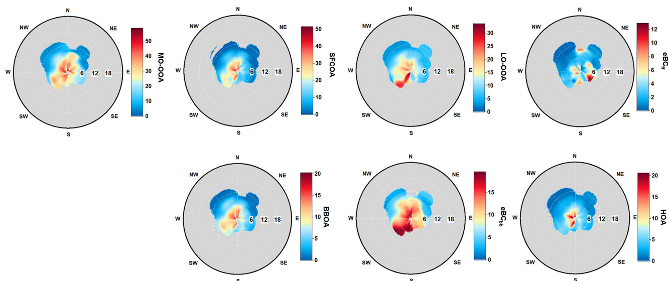
Figure 8. Estimation of source regions using NWR approach around the site using wind speed and wind direction for organics and black carbon factors during full period from 25 October to 15 November 2023.
