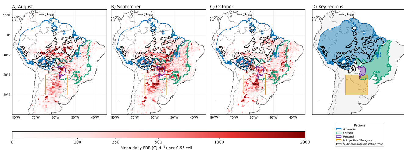
Figure 3. Monthly mean daily Fire Radiative Energy (FRE) over South America on a 0.5° grid. Panels (A)–(C) show August, September, and October 2020, respectively. The colour scale gives mean daily FRE in GJ d -1 per 0.5° cell, ranging from white (no detected FRE) to dark red (high FRE). Panel (D) shows the geographical context of main regions. The outlines of these regions, together with the South Amazonia deforestation front, are also overlaid on Panels (A)–(C).
