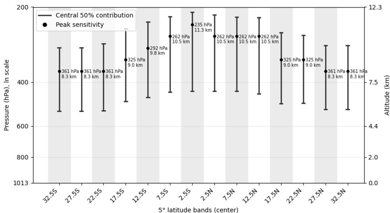
Figure 1. IASI MT-CO 2 vertical sensitivity expressed as pressure and altitude for 5° latitude bands (centered from 32.5°S to 32.5°N). For each band, the vertical black line with end caps shows the central 50 % of the column that contributes most to the IASI CO 2 retrieval (from the 25th to the 75th percentile of the weighting-function contribution). The black dot marks the pressure of maximum sensitivity (“peak sensitivity”), and the annotation gives both the peak pressure (hPa) and its approximate tropical altitude (km) derived from a simple hydrostatic tropical profile.
