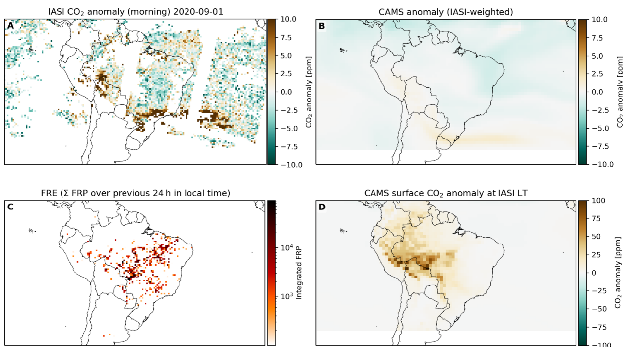
Figure 7. Spatial comparison of satellite- and model-based CO 2 anomalies and fire activity over South America for 1 September 2020 (morning overpass; \sim 09:30 local solar time). (A) Gridded IASI mid-tropospheric CO 2 anomaly (ppm). (B) CAMS CO 2 anomaly for the IASI-weighted partial column, sampled at the IASI local overpass time and expressed on the same anomaly scale as (A) (ppm). (C) Fire Radiative Energy proxy computed as the sum of GOES-16 Fire Radiative Power (FRP) accumulated over the 24 h preceding the overpass in local time, aggregated on a 0.5° grid and displayed on a logarithmic scale. (D) CAMS surface CO 2 anomaly at the IASI local overpass time (ppm).
