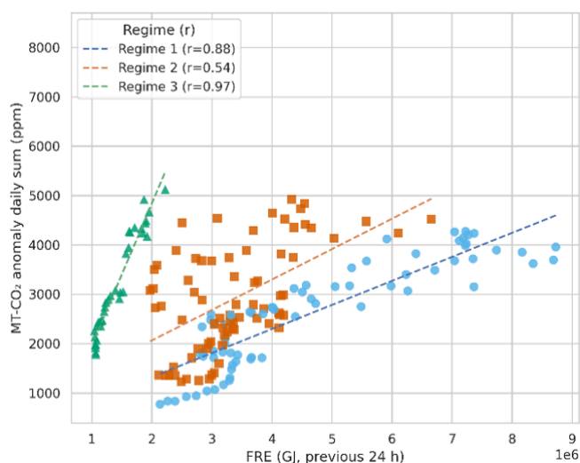
Figure 6. Daily sum of mid-tropospheric CO 2 anomalies (ppm) vs. Fire Radiative Energy (FRE, GJ) for three transport regimes: longitudinal transport (blue), circular transport (orange), and combined transport (green). Pearson correlation coefficients “ r ” are indicated for each transport regime.
