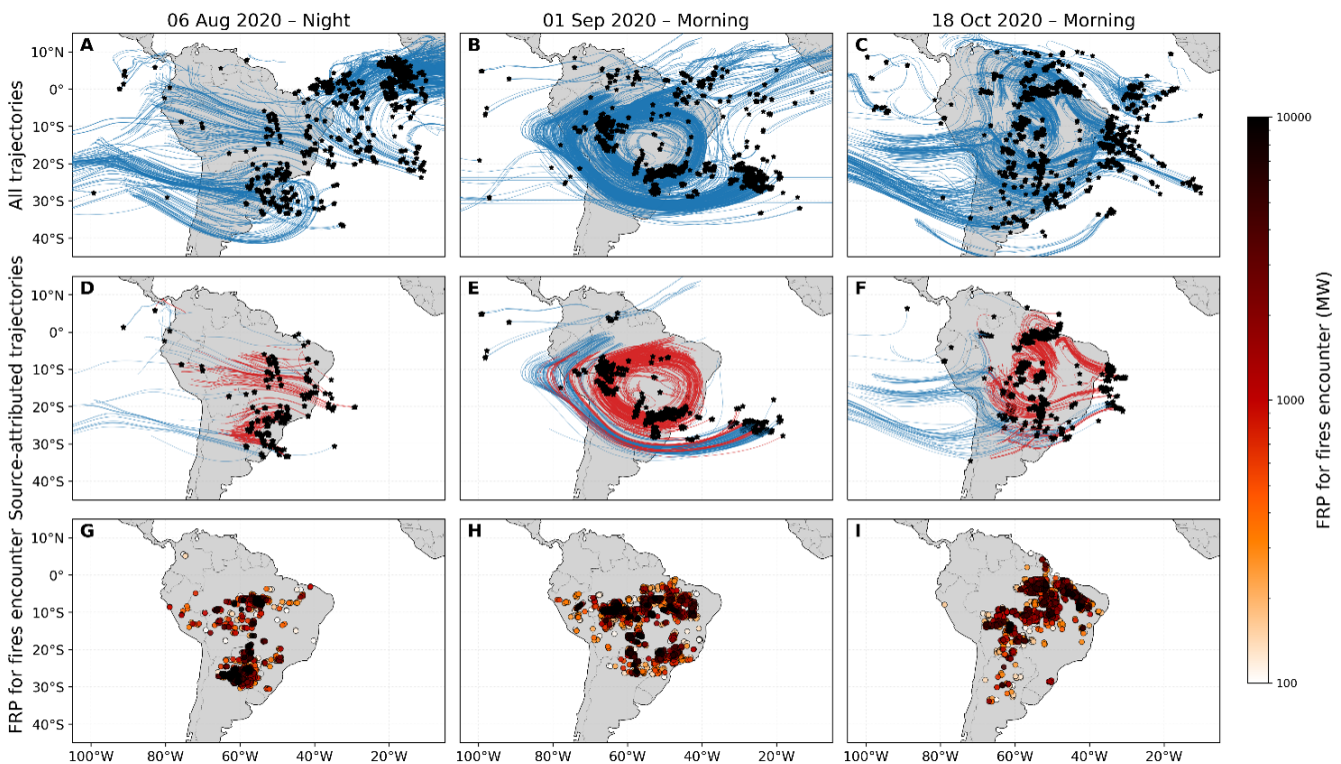
Figure 4. Case studies of mid-tropospheric CO 2 anomalies linked to South American fires. Each column shows one case study (6 August 2020 – night, 1 September 2020 – morning, 18 October 2020 – morning), and each row shows a different stage of the source-attribution procedure. Panels (A)–(C) display all backward trajectories started from the selected CO 2 anomalies for each case (blue lines), with the anomaly locations indicated by black stars. Panels (D)–(F) show only the “source-attributed” subset, i.e. trajectories that fulfil the filtering criteria and encounter at least one fire along their path; red segments mark the part of the trajectory up to the last 1° × 1° hourly aggregation of fire encounter, while blue segments correspond to trajectories with no detected fires, and black stars again mark the anomaly locations. Panels (G)–(I) display only the locations of the last fire encountered by each source-attributed trajectory. Coloured circles denote fire pixels, with marker size and colour proportional to the Fire Radiative Power (FRP) at the last encounter.
