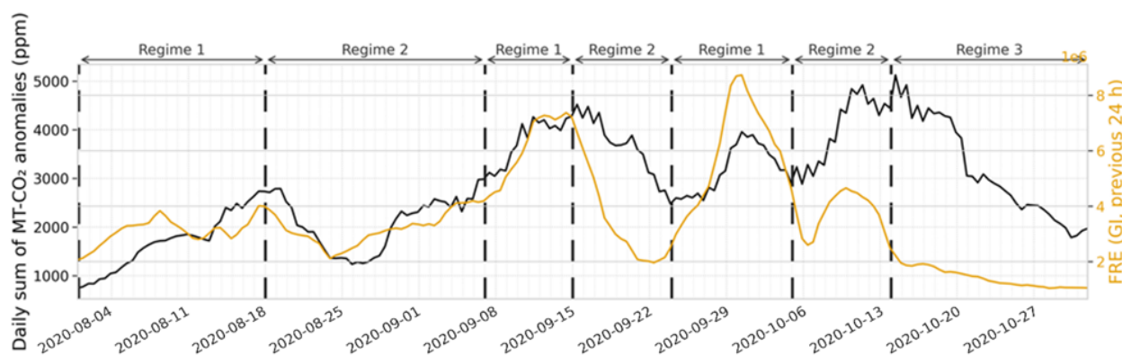
Figure 5. Time series, smoothed using a 72 h window, of the daily sum of mid-tropospheric CO 2 anomalies derived from IASI morning and evening overpasses (black), over South America during the 2020 fire season and of total FRE (orange) from GOES-16 observations, integrated over South America and computed 24 h prior to each IASI observation to account for transport time. The “Regime” delimiters highlight three representative atmospheric transport regimes periods: Regime 1 for longitudinal regime, Regime 2 for circular regime, and Regime 3 for combined regime.
