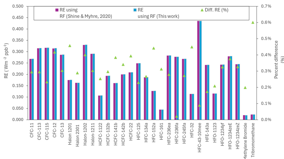
Figure 4. REs ( \text{W m}^{-2} \text{ppb}^{-1} , left axis scale) determined using the updated Pinnock Curve (blue bars) and that of Shine and Myhre (2020) (purple bars) for 30 halocarbons. The percentage differences between the two sets of REs are also reported (green triangles, right axis scale). Values presented here use QC calculations of absorption cross-section over the entire 0\text{--}3000 \text{ cm}^{-1} spectral region.
