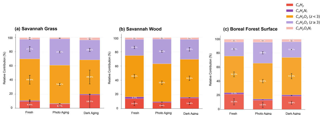
Figure 5. Stacked bar plots showing the mean relative contribution (%) of compound classes ( C_xH_y , C_xH_yO_z ( z < 3 ), C_xH_yO_z ( z \geq 3 ), C_xH_yN_i and C_xH_yO_zN_i ) to the total mean mixing ratio (ppbv) for (a) savannah grass, (b) savannah wood and (c) boreal forest surface under fresh, photochemical aging and dark aging conditions. Error bars indicate the standard deviation; n = 9 , 7 and 2 (savannah grass); n = 7 , 4 and 3 (savannah wood) and n = 4 , 2 and 2 (boreal forest surface) for fresh, photo aging and dark aging conditions.
