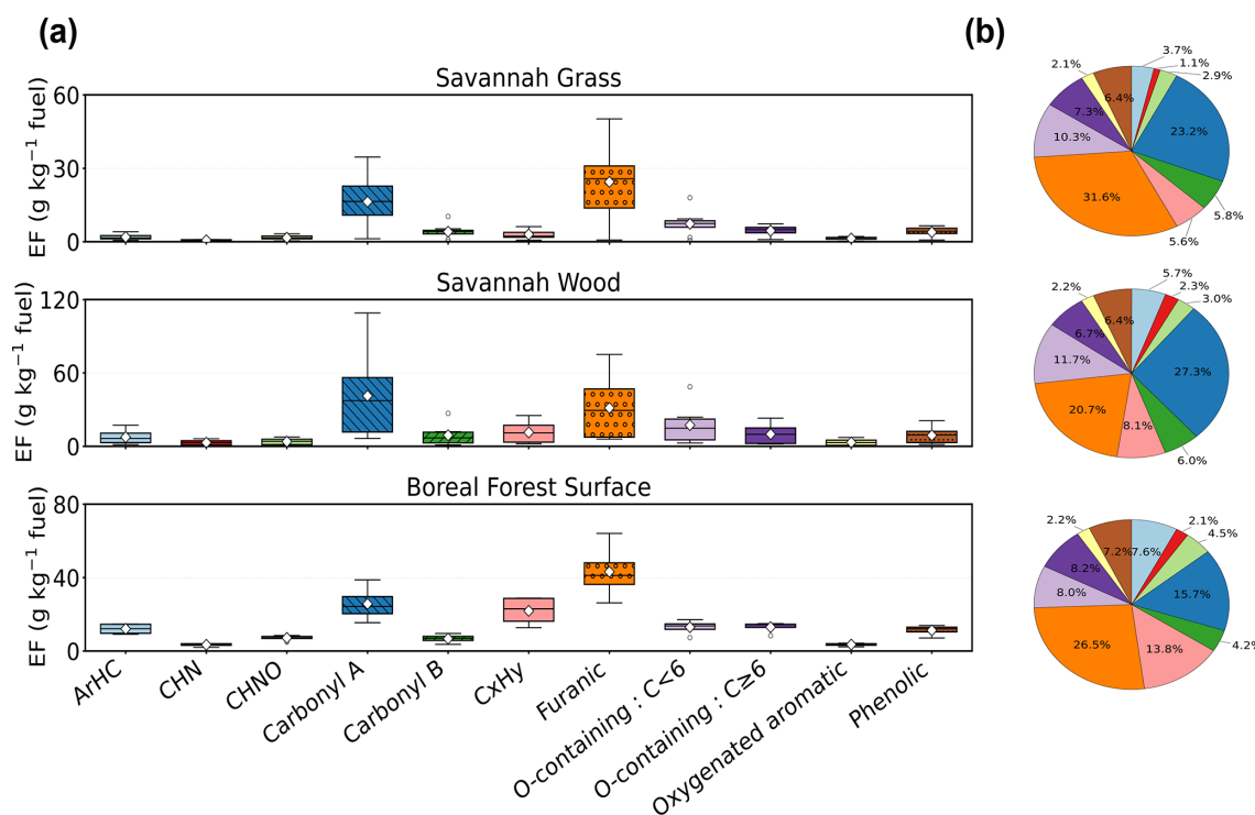
Figure 1. (a) Fresh emission factor (EF) distributions by compound class for savannah grass, savannah wood, and boreal forest surface. For each fuel, boxplots show the variability across experiment days of class-averaged EFs ( \text{g kg}^{-1} fuel). Boxes are colored by class (ArHC, CHN, CHNO, carbonyl A, carbonyl B, C x H y , furanic, O-cont.: C < 6, O-cont.: C ≥ 6, oxygenated aromatic, phenolic). Boxplots use 1.5 \times \text{IQR} (Interquartile Range) whiskers; hollow circles = outliers; white diamonds = mean. Note that different y-axis scales are used for the three biomass fuels. (b) Companion pie charts showing the mean fractional contribution (%) of each class to the total fresh EF for the same biomass fuels.
