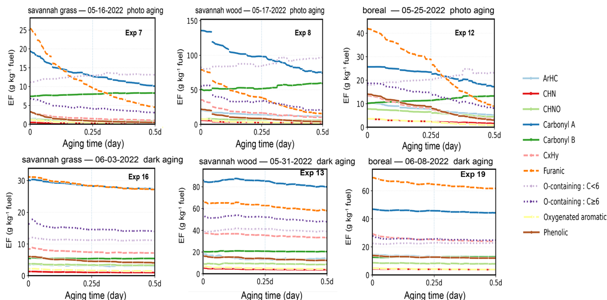
Figure 2. Chemical evolution of organic vapors categorized by functional groups during aging in the smog chamber. The x axis shows equivalent aging time up to 0.5 eqv. day, and y axis represents emission factors (EFs; \text{g kg}^{-1} dry fuel). One selected photochemical aging experiment and one selected dark aging experiment are shown for each biomass fuel and the remaining experiments are provided in Fig. S4. Aging time t = 0 represents when UV light was switched on for photochemical aging experiments or when \text{O}_3 was injected for dark aging experiments.
