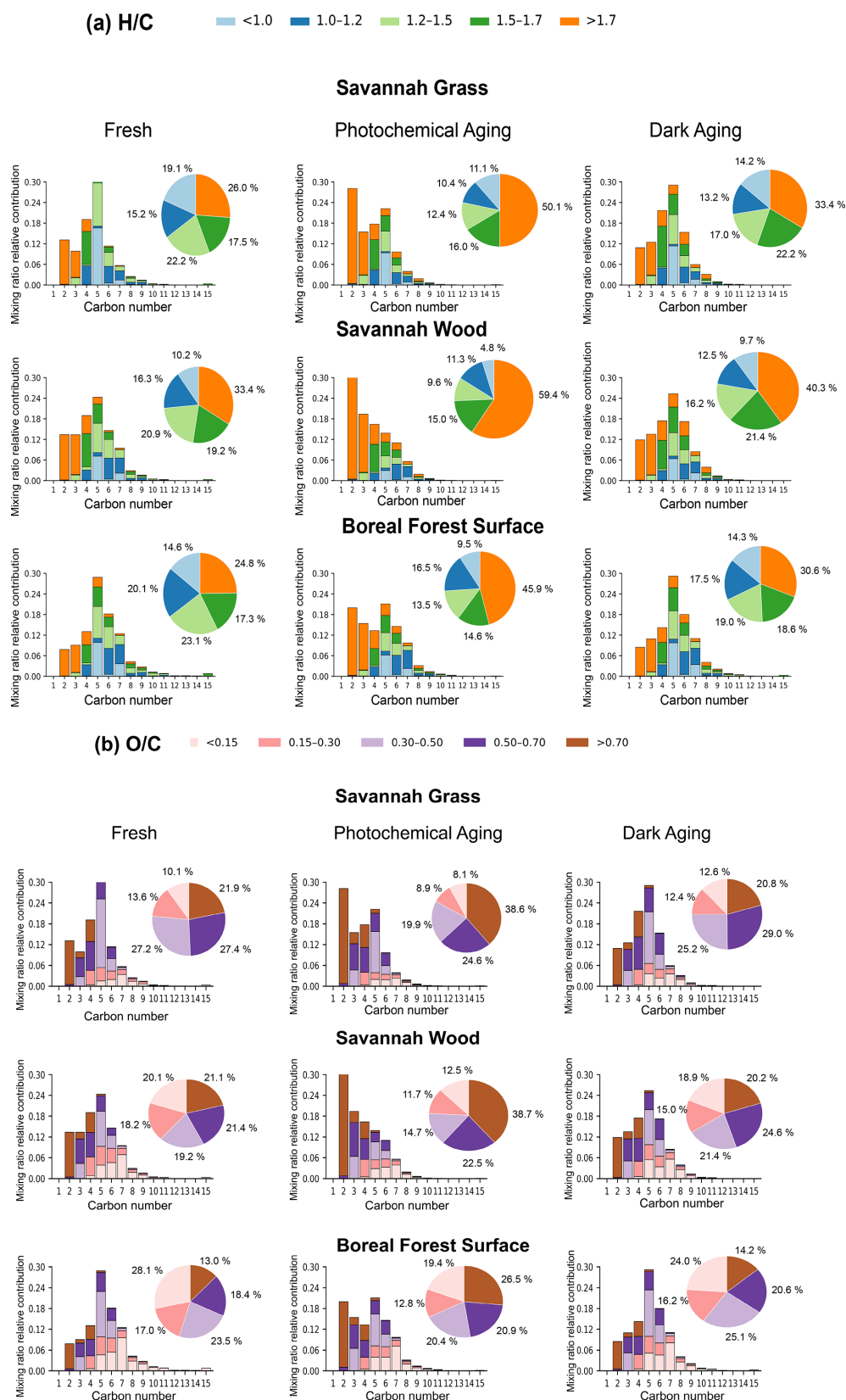
Figure 4. The average carbon distribution for savannah grass, savannah wood and boreal forest surface across fresh, photochemical aging conditions and dark aging colored by (a) H/C and (b) O/C. The pie charts show the corresponding contributions by H/C and O/C ratios for each regime.
