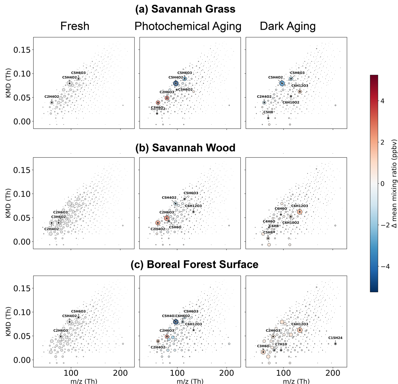
Figure 6. Kendrick mass defect (KMD) plots for savannah grass, savannah wood and boreal forest surface across fresh, dark aging ( \Delta\text{O}_3 ) and photochemical aging ( \text{UV} + \Delta\text{O}_3 ). In fresh panel, marker size \propto to mean mixing ratio (ppbv), normalized within each biomass. In aging panels, marker size \propto |\Delta| = \text{ppbv}_{\text{aged}} - \text{ppbv}_{\text{fresh}} . Colors in aged panels encode the signed change on a global, symmetric scale: red = increase, blue = decrease (color intensity scales with |\Delta| ). Top-changing species are indicated by black star markers and bold labels with a white outline.
