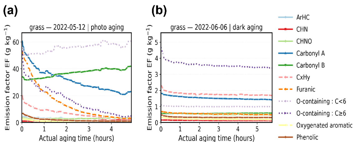
Figure S2. Representative time series of one photochemical and one dark aging experiment for savannah grass biomass fuel.
