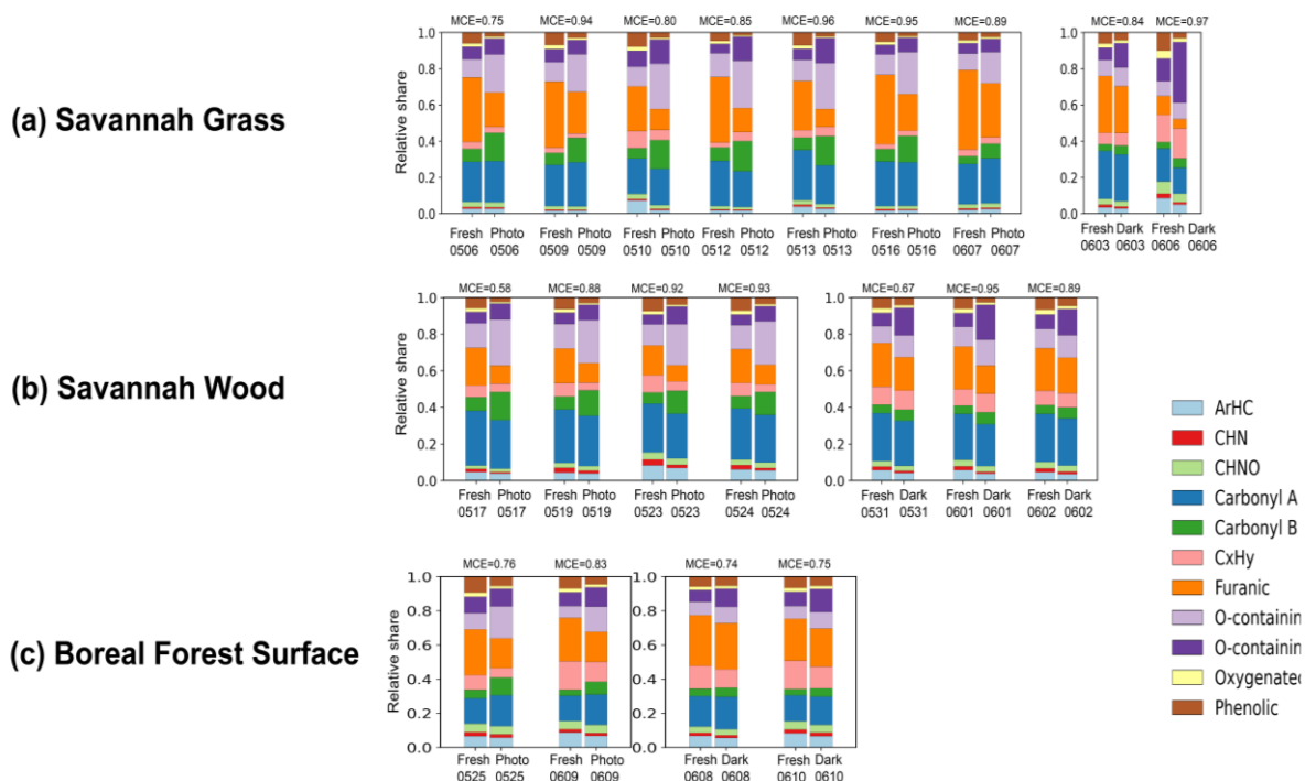
Figure S5. Relative share of organic vapor classes in the BB emissions measured by Vocus PTR-MS for photoaging and dark aging experiments for (a) savannah grass (b) savannah wood and (c) boreal forest surface.
