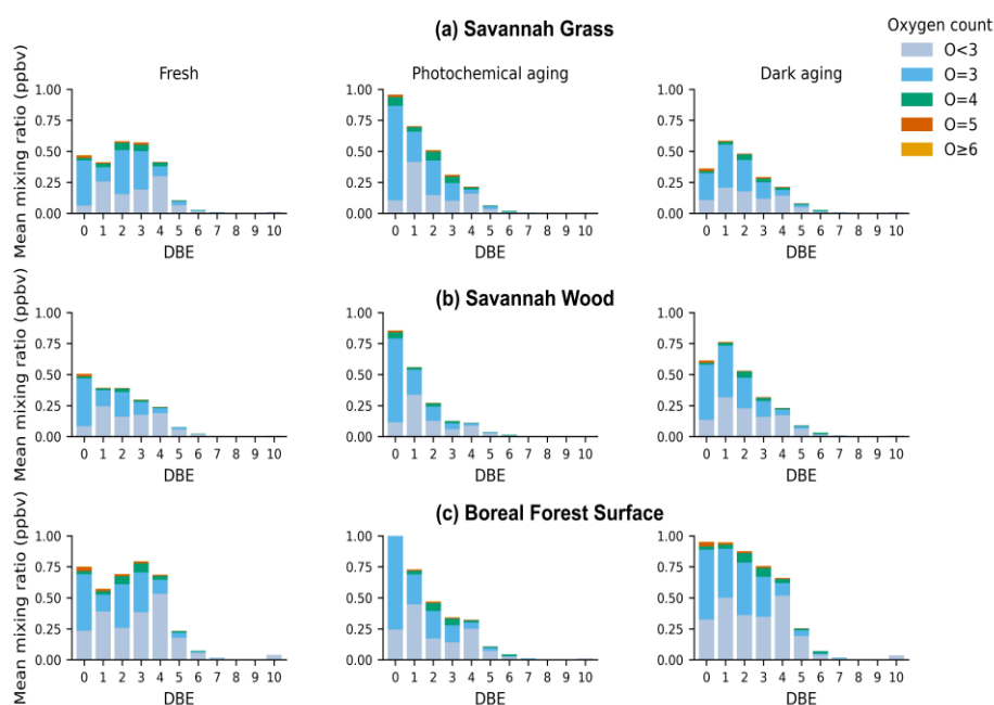
Figure S6. Mean mixing ratio distribution of DBE for (a) savannah grass (b) savannah wood and (c) boreal forest surface. Bar colors represent compounds with different oxygen content.
