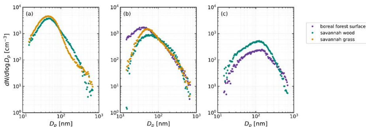
Figure S3. The median primary size distributions grouped according to MCE ranges for savannah grass, savannah wood and boreal forest surface.
