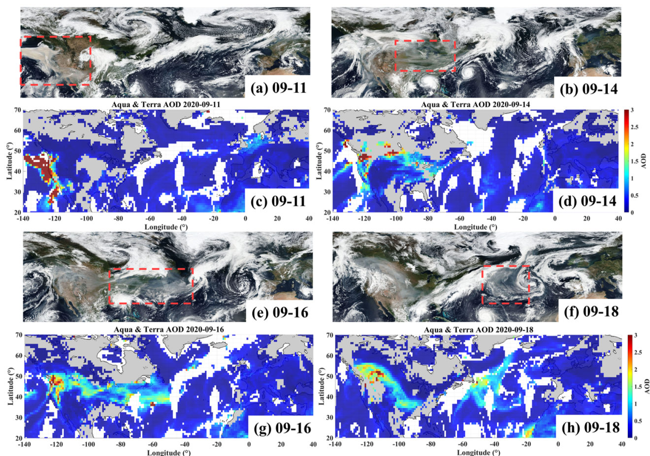
Figure 1. Observations of spaceborne passive instruments in the spatial range of 140° W to 40° E and 20 to 70° N. True-color images from VIIRS on (a) 11, (b) 14, (e) 16, (f) 18 September 2020, acquired on the Worldview ( https://worldview.earthdata.nasa.gov , last access: 23 July 2026). Averaged AOD from both Aqua and Terra on (c) 11, (d) 14, (g) 16, (h) 18 September 2020. In the AOD maps, the grey and white parts indicate the land and the invalid data, respectively. Satellite imagery © NASA Earthdata/Worldview.
