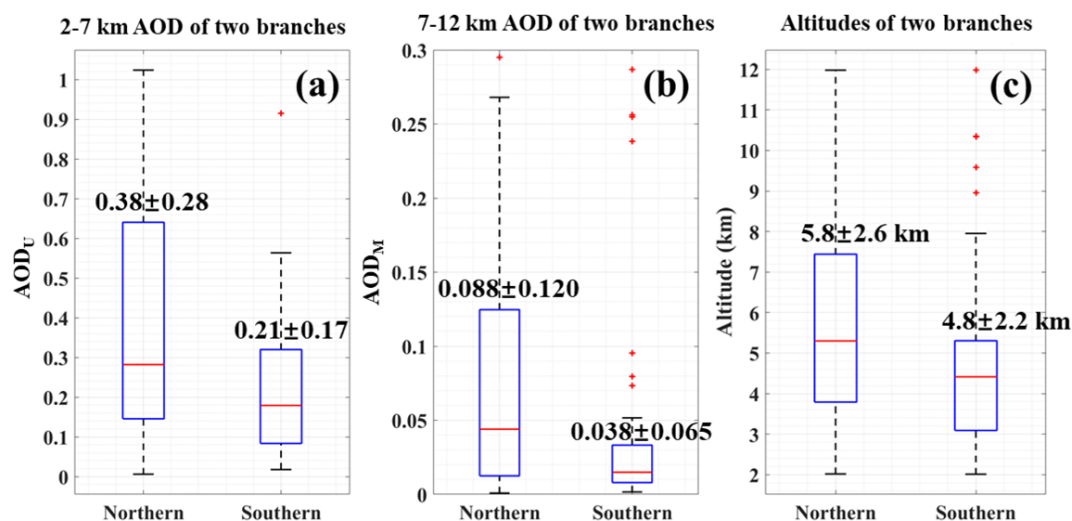
Figure 11. Statistical results of the two branches following the plume separation calculated from ALADIN smoke observations within the purple dotted box (latitude 45–70° N, longitude 40–20° W) and the pink dotted box (latitude 20–45° N, longitude 40–20° W) in Fig. 9a, labelled “Northern” and “Southern”. (a) 2–7 km AOD ( AOD_U ) of two branches; (b) 7–12 km AOD ( AOD_M ) of two branches; (c) Layer altitudes of two branches.
