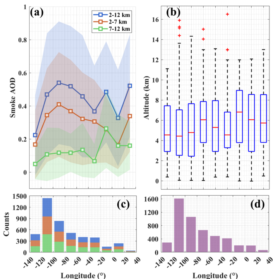
Figure 10. Statistical results (a) smoke AOD (means and standard deviations), (b) smoke bins altitude (boxplot) along longitude. (c, d) The corresponding data counts of the statistics. The statistics were calculated using the Aeolus smoke dataset in the period of 14 to 21 September 2020, in the smoke plume transport region of 140° W to 40° E and 20 to 70° N, and with the longitude grid of 20°. Smoke AOD includes total AOD (2 to 12 km), AOD within 2 to 7 km ( AOD_M ), and AOD within 7 to 12 km ( AOD_U ), indicated by the blue, red and green curves, respectively. In panel (c), the corresponding data counts are also presented by the stacked bars in the same color with the AOD curves.
