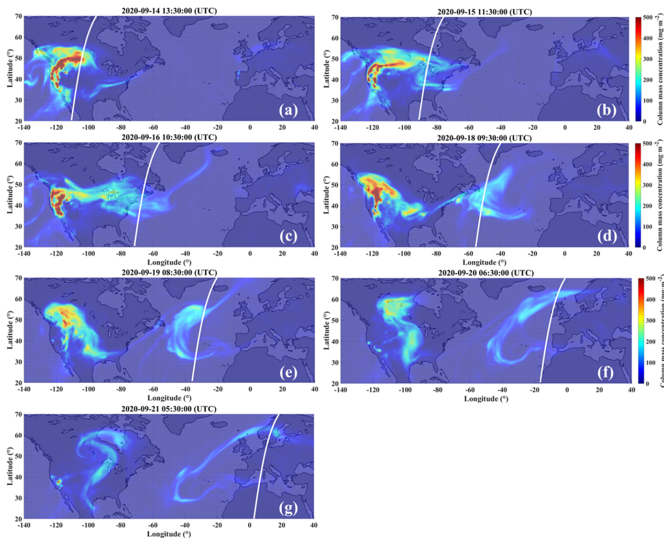
Figure 6. Smoke column mass concentration map in the spatial range of 140^\circ\text{W} to 40^\circ\text{E} , 20^\circ to 70^\circ\text{N} , on (a) 14, (b) 15, (c) 16, (d) 18, (e) 19, (f) 20, (g) 21 September 2020, respectively. The white curves indicate the selected Aeolus orbits on the same days.
