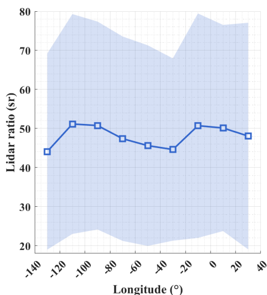
Figure 12. Statistical results (means and standard deviations) of smoke lidar ratio along longitude. The statistics were calculated by using the Aeolus smoke dataset (within the altitude range of 2 to 12 km) in the period of 14 to 21 September 2020, in the smoke plume transport region of 140° W to 40° E and 20 to 70° N, and with the longitude grid of 20°.
