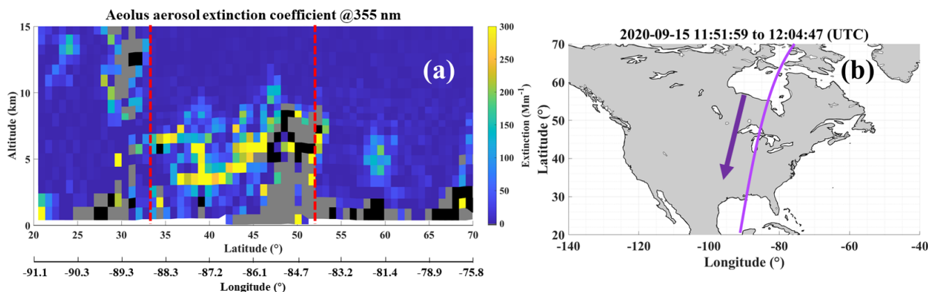
Figure 4. (a) One cross-section example of Aeolus aerosol extinction coefficient crossing the smoke plume, on 15 September 2020, starting at 11:51:59 UTC on 70.0° N, 75.8° W and ending at 12:04:47 UTC on 20.5° N, 91.1° W. (b) The corresponding descending orbit indicated by the purple curve (Aeolus orbit) and the purple arrow (Aeolus flight direction). The data in panel (a) has been processed to derive smoke data from Aeolus by the steps introduced in the section “Derivation of the smoke dataset from ALADIN observations”. The black bins indicate the invalid values, while the grey ones indicate the cloud contaminated bins. The profiles inside two red dashed lines are the “smoke profiles”.
