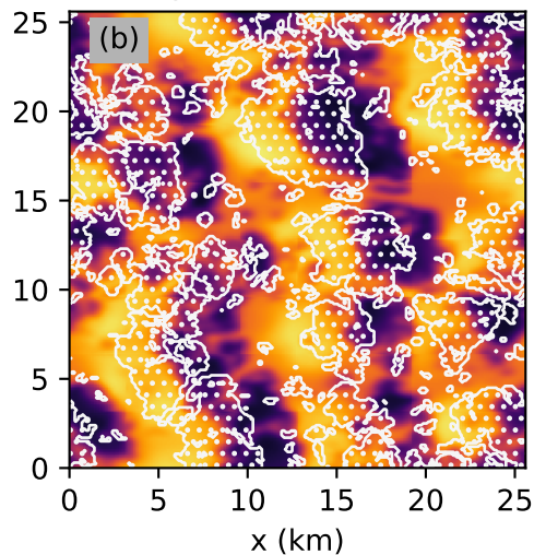
dynamic TenStream
