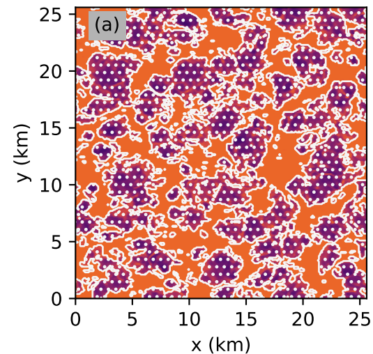
\delta -Eddington
