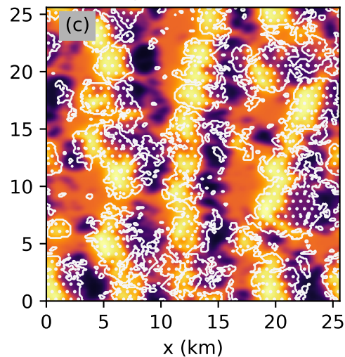
original TenStream
