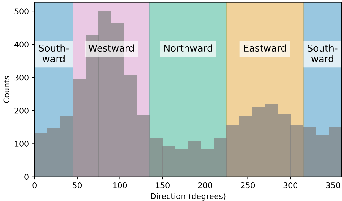
NSA wintertime wind direction at 500 m
