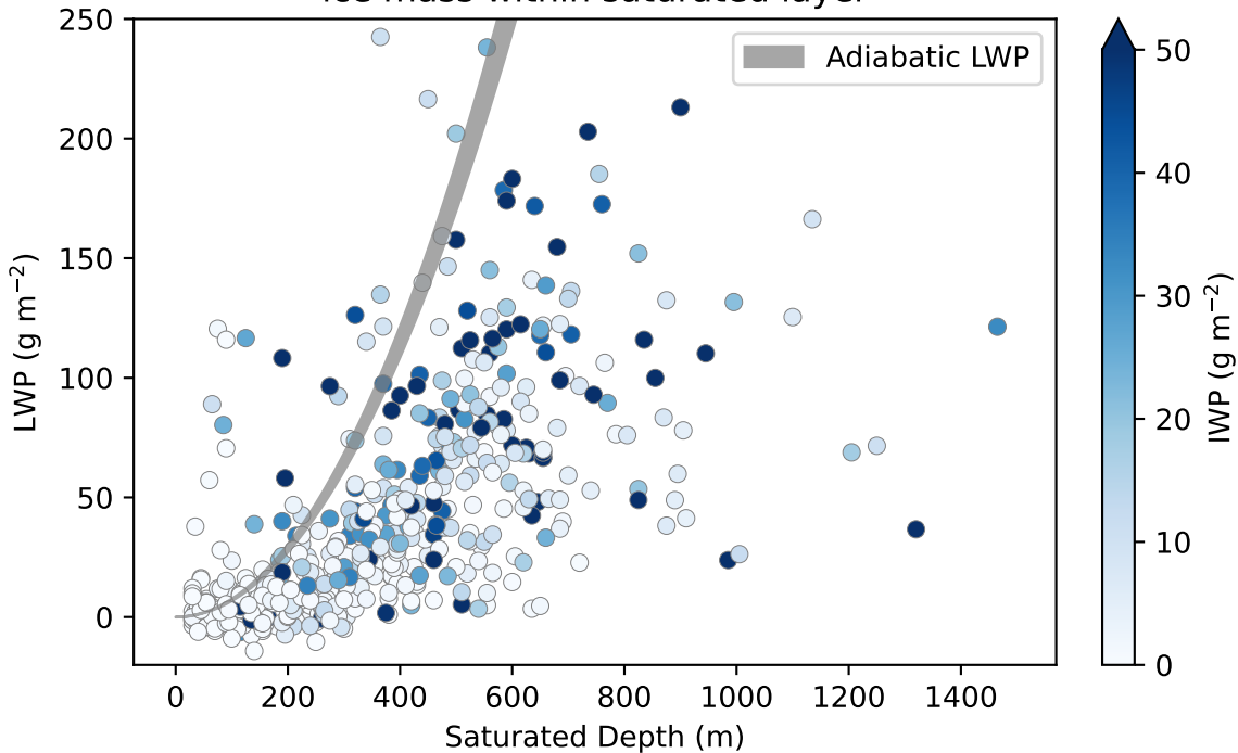
LWP vs Saturated Depth shaded by ice mass within saturated layer
