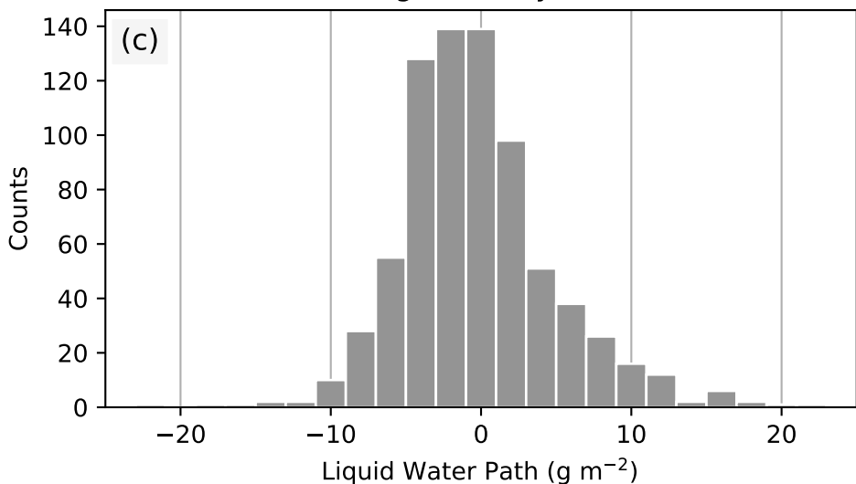
LWP during clear sky conditions
