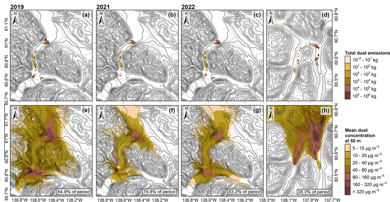
Figure 11. (top row) Summed dust ( 0.2\text{--}20.0\text{ }\mu\text{m} ) emissions (kg) from 0.6\text{ km}^2 grid cells across simulation periods in d01 (a–c) and d02 (d). (bottom row) Mean dust concentration at 50 m during active emission periods (non-zero emissions anywhere within domain) in d01 (e–g) and d02 (h). Percentage of period with active emissions indicated in each figure. Contours kriged from model topography.
