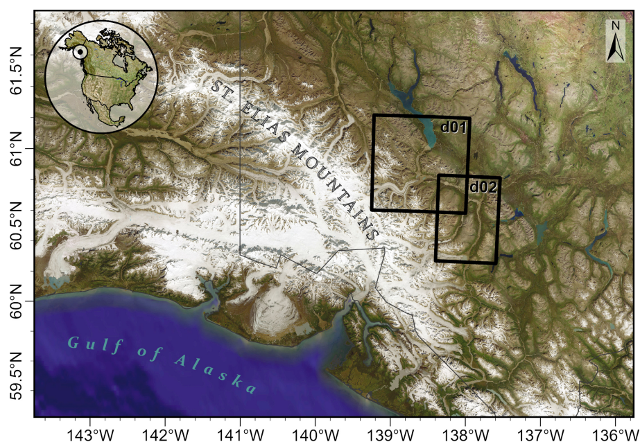
Figure 1. Overview of the study region and location of the two model domains (d01; d02) (Source: Maxar, Esri, USGS | Powered by Esri).
