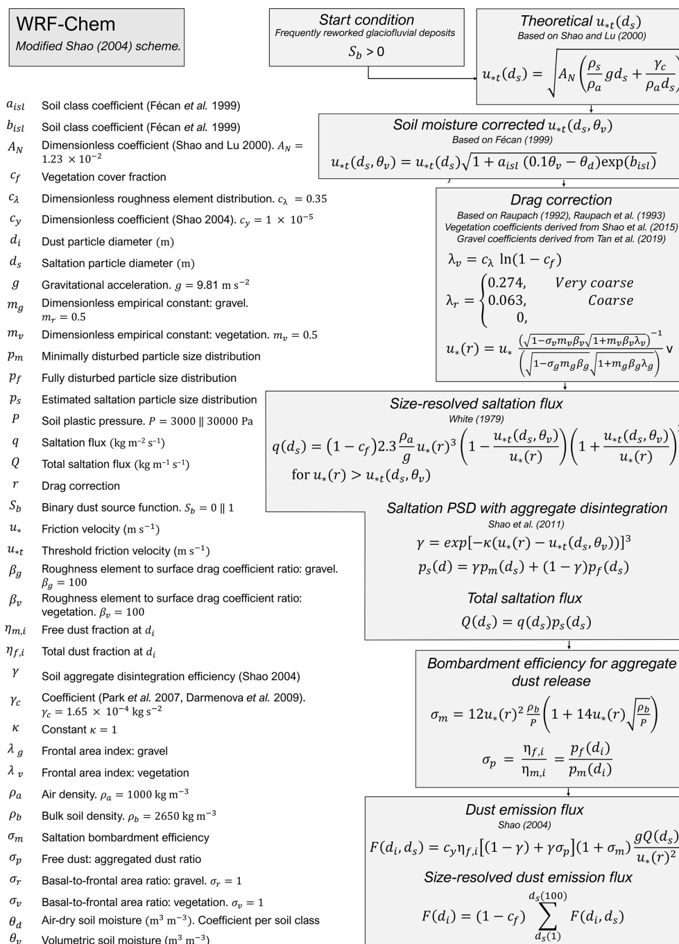
Figure 2. Overview of the modified Shao (2004) scheme in WRF-Chem developed in this work. Modifications were applied to the drag partition parameterisation ( \lambda_r , u_*(r) ), further detailed in Sect. 2.2.3.
