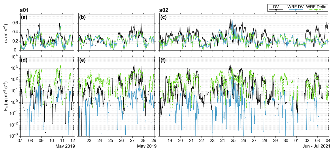
Figure 7. Comparison of measured (DV) and WRF-simulated variables: at the DV grid point (WRF.DV) and averaged over emissive grid cells of the A'äy Chù delta (WRF.Delta). (a–c) Friction velocity ( u_* ). (d–f) Vertical dust flux ( F_d ) (0.25–9.81 \mu\text{m} ).
