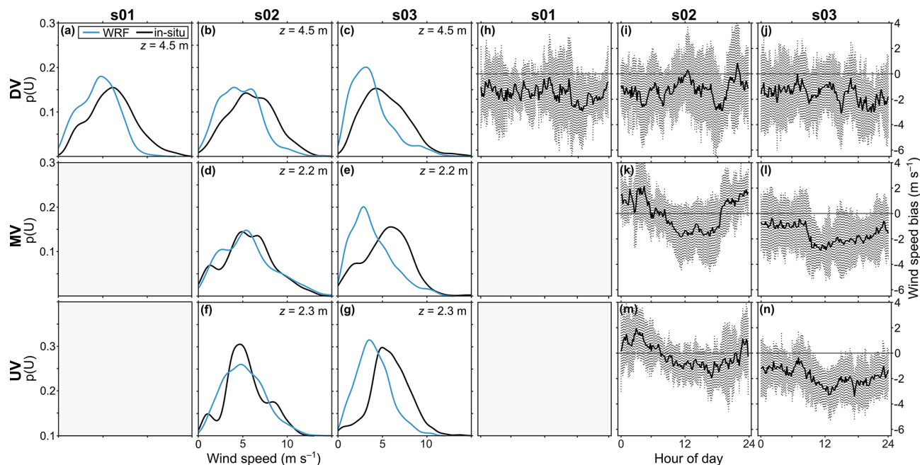
Figure 6. (a–g) Observed and simulated wind speed distributions at respective sensor height ( z ) for each simulation periods (s01: 2019 – 12 d; s02: 2021 – 11 d; s03: 2022 – 19 d). The s02 comparison only compares records from 24 June 2021–3 July 2021 due to station data availability. (h–n) WRF wind speed bias vs. surface observations, shaded interval indicates 1\sigma .
