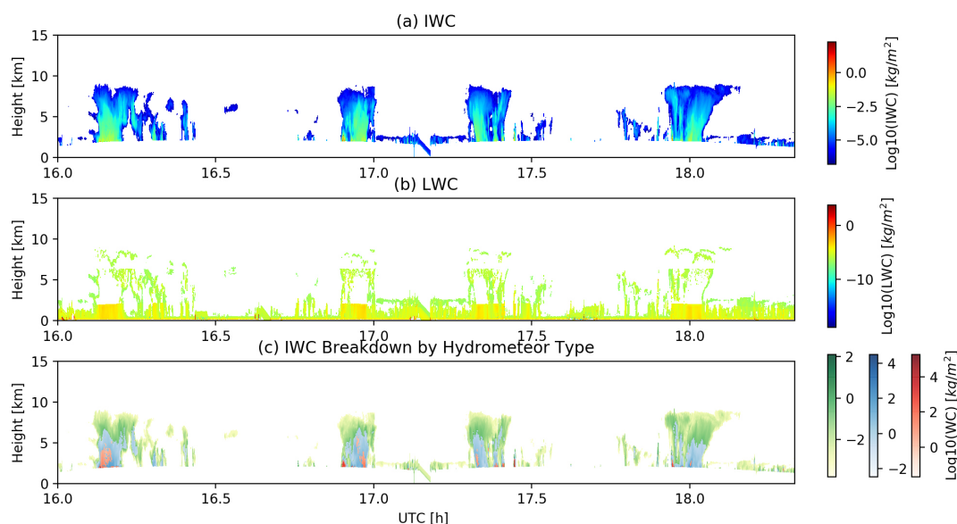
Figure 5. Vertical water content (WC) profile retrieved from CRS plus HIRWAP. (a) IWC; (b) LWC; (c) IWC from cloud ice (green), snow aggregates (blue), graupel (red) and liquid. Colorbars are in \text{Log}_{10} -scale. Note that positive LWC pixels overlap with many of the positive IWC pixels (e.g., cloud top, cloud boundary, SCLW layer, etc.), so they are shown separately in (a) and (b) to ease visual comparison.
