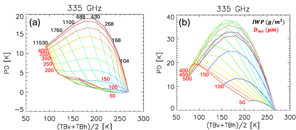
Figure 14. Look-up-table (LUT) for 325.15 + 10 GHz for (a) 6-bullet rosette and (b) column ice.
