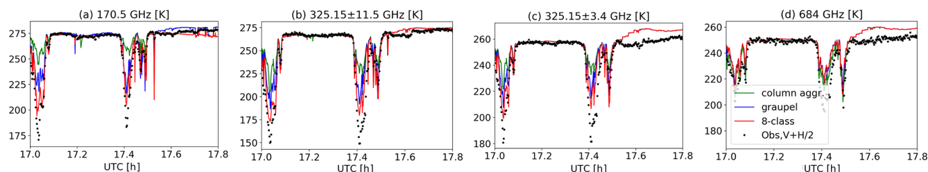
Figure 7. Timeseries of observed TB (black asterisks) versus simulated TB. Red, blue and green lines are using detailed frozen hydrometeors, uniform graupel and uniform LCA assumptions, respectively. (a) 170.5 GHz; (b) 325.15 \pm 11.5 GHz; (c) 325.15 \pm 3.4 GHz; (d) 684 GHz. The observed TB is an average between V-pol and H-pol measurements.
