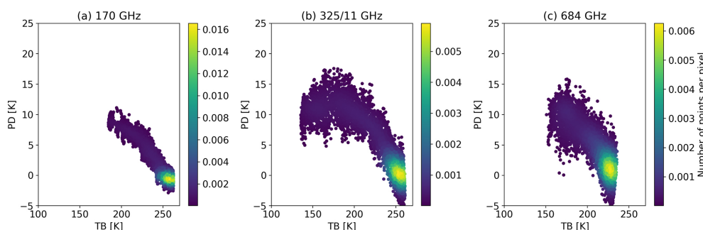
Figure 13. Density plots of the observed PD–TB relationship during 16:05–16:24 UTC for (a) 170, (b) 325.15 \pm 11 and (c) 684 GHz.
