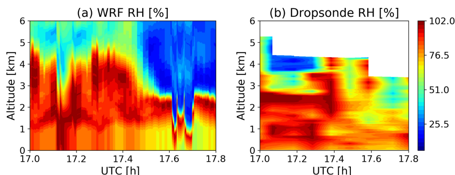
Figure 8. Timeseries of (a) WRF model simulated relative humidity (RH, unit in %) and (b) dropsonde observed ones during the same period of Fig. 7 (17:00–17:48 UTC).
