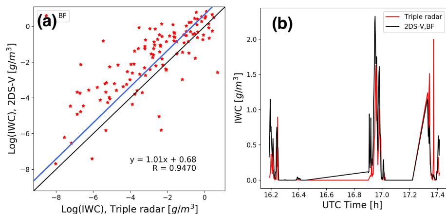
Figure 9. Comparison between joint CRS+HIWRAP IWC retrievals and 2D-S cloud probe retrievals at the collocated radar range bin where P-3 was cruising. (a) Scatter plots from the collocated samples and (b) displaying the same data samples using a timeseries. The Brown and Francis (1995) m – D relationship is used for 2D-S. Linear regression results for (a) are added as the blue line and equation/ R -value written in the bottom right corner of panel (a).
