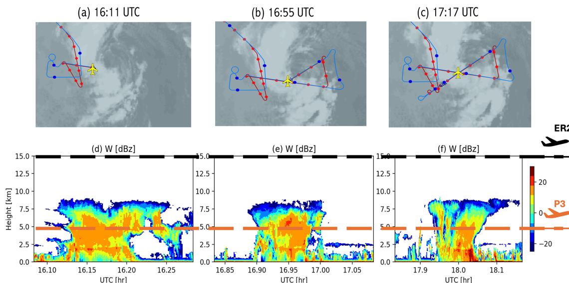
Figure 1. Illustration of the weather system and flight patterns of the 15 January 2023 IMPACTS campaign case. Top rows are ER-2 (blue) and P-3 (red) flight routes overlaid on GOES-16 satellite false-color Advanced Baseline Imager (ABI) albedo measurements at three different UTC times. Dots mark the time at intervals of 5, 10, 15 min, and so on. Cyclone center was roughly at 37° N, 70° W. Bottom row presents the CRS radar reflectivity curtains during the corresponding time segments. Two aircraft icons roughly represent ER-2 and P-3 flight altitudes. Top panels are cropped from https://catalog.eol.ucar.edu/maps/impacts_2023 (last access: 26 June 2026), and bottom panels are calibrated L1B CRS W-band radar reflectivities at corresponding periods. GOES-16 ABI data courtesy of NOAA. NCAR/EOL map products courtesy of NCAR/UCAR. CRS radar data courtesy of NASA.
