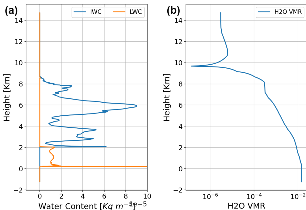
Figure A1. Sample (a) IWC (blue), LWC (orange) and (b) water vapor mixing ratio profiles at 18:00 UTC. IWC and LWC are retrieved from triple-frequency radar measurements, and water vapor mixing ratio is from the WRF simulation.
