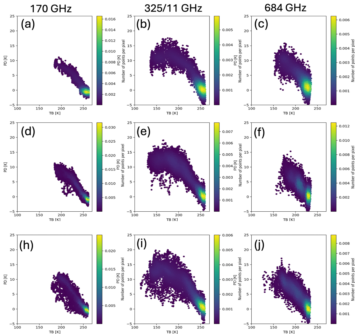
Figure B1. Same with Fig. 13, except the second row is made up from samples collected during 16:05–16:24 UTC, and last row from 17:15–17:30 UTC.
