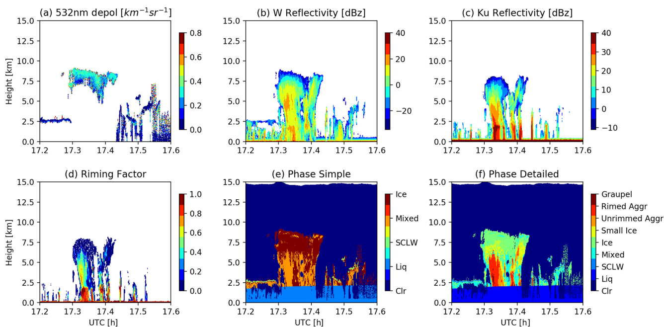
Figure 3. An example to show how the final hydrometeor type is decided based on (a) lidar 532 nm depolarization ratio ( \delta ) and backscatter ( \beta ; not shown); (b) W-band reflectivity; (c) Ku-band reflectivity; and (d) calculated riming parameter ( r ). The final coarse and detailed type classification products are shown in (e) and (f), respectively.
