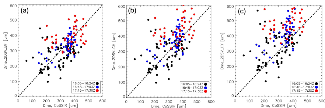
Figure 15. Scatter plots of retrieved D_{\text{me}} from CoSSIR 325.15 \pm 11 GHz (horizontal axis) in comparison with collocated 2D-S retrievals using the m – D relationship from (a) Brown and Francis (1995), (b) Chase et al. (2021) and (c) Heymsfield et al. (2010). Black, blue and red dots are taken from 16:05–16:24, 16:48–17:03 and 17:15–17:30 UTC periods, respectively.
