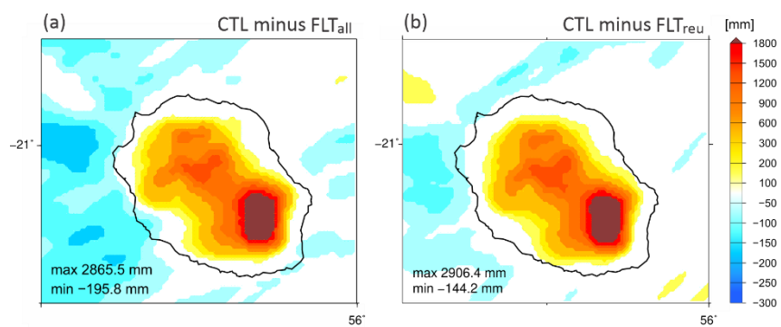
Figure S1. The difference in five-day accumulated precipitation (a) between CTL and FLT_{all} (CTL minus FLT_{all} ), and (b) CTL and FLT_{reu} (CTL minus FLT_{reu} ).
