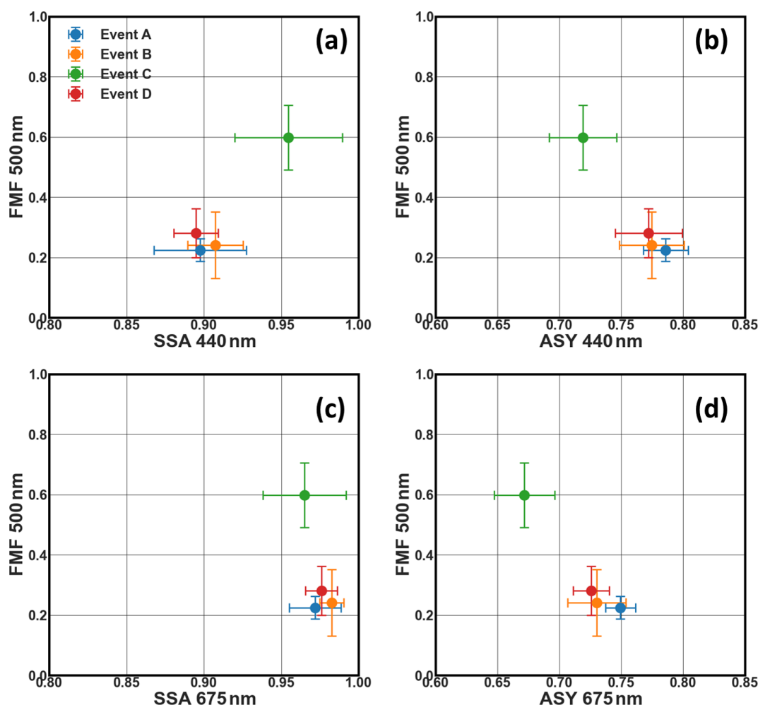
Figure 10. Comparison of FMF at 500 nm with (a, c) SSA at 440 and 675 nm and (b, d) ASY at 440 and 675 nm for different aerosol events. Data points represent the averaged values over all stations on their peak date during event A (blue), event B (orange), event C (green), and Event D (red), with horizontal and vertical error bars indicating uncertainties in the respective measurements.
