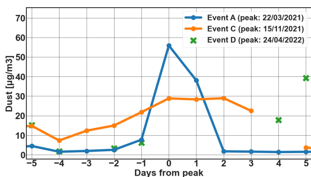
Figure 12. Surface dust concentration measured at CAO-Agia Marina Xyliatou during the events that affected the station.
