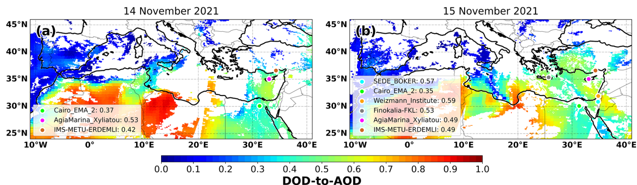
Figure C3. DOD-to-AOD ratios (at 550 nm) over the Mediterranean Basin from MIDAS for event C. The days with the available almucantar AERONET retrievals are displayed along with the specific stations (colored circles).
