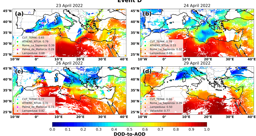
Figure C4. DOD-to-AOD ratios (at 550 nm) over the Mediterranean Basin from MIDAS for event D. The days with the available almucantar AERONET retrievals are displayed along with the specific stations (colored circles).
