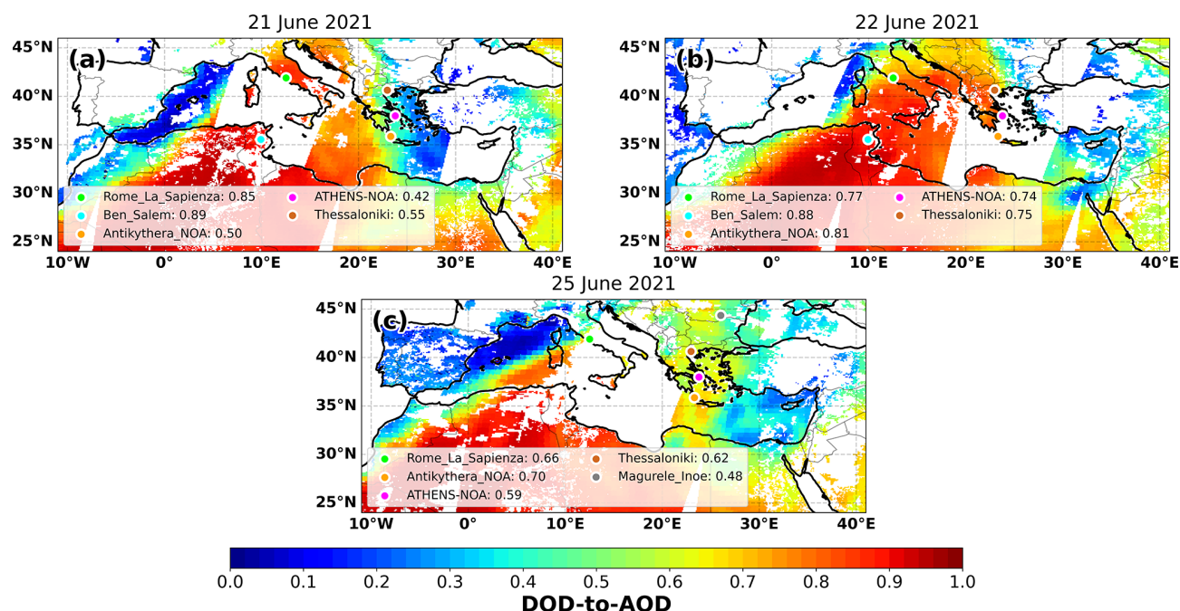
Figure C2. DOD-to-AOD ratios (at 550 nm) over the Mediterranean Basin from MIDAS for event B. The days with the available almucantar AERONET retrievals are displayed along with the specific stations (colored circles).
