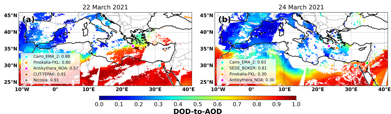
Figure C1. DOD-to-AOD ratios (at 550 nm) over the Mediterranean Basin from MIDAS for event A. The days with the available almucantar AERONET retrievals are displayed along with the specific stations (colored circles).
