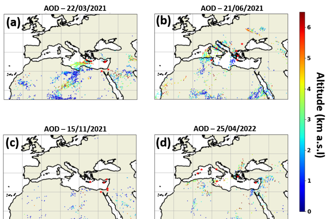
Figure D2. Spatial distribution of IASI-MAPIR derived mean dust plume altitude (colored pixels, km a.s.l.), during the four selected dust events.
