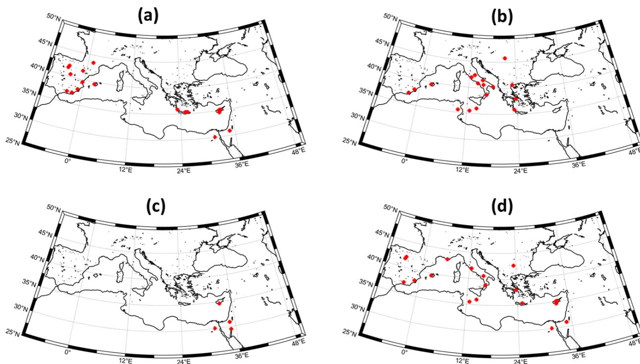
Figure 1. Map of AERONET stations where \text{AOD} > 0.2 and (ii) -0.1 < \text{AE} < 0.3 between (a) 18 and 29 March 2021, (b) 17 and 28 June 2021, (c) 10 and 21 November 2021, and (d) 20 April and 10 May 2022.
